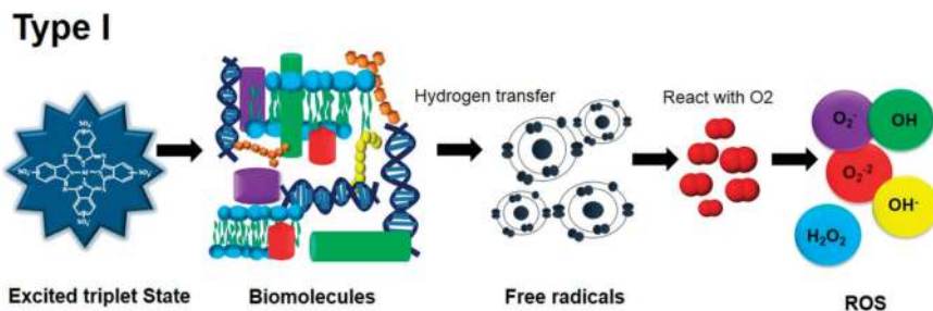
Figure 5. Type I reaction in PDT.
