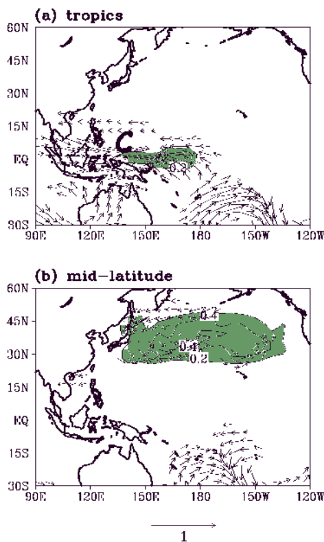
Fig. 7. SST anomalies (contour) and 850 hPa wind anomalies from the model simulations with the prescribed SST anomalies over (a) the equatorial region (130°E-175°E, 5°S-5°N) and (b) mid-latitudes (140°E-120°W, 25°N-45°N). Adapted from Tu et al. (2009).
