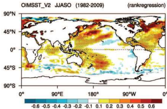
Fig. 10. Trend of SST in JJASO for the period of 1982-2009. The unit is °C per decade. The dotted area denotes that the trend is statistically significant at the 5% level.
