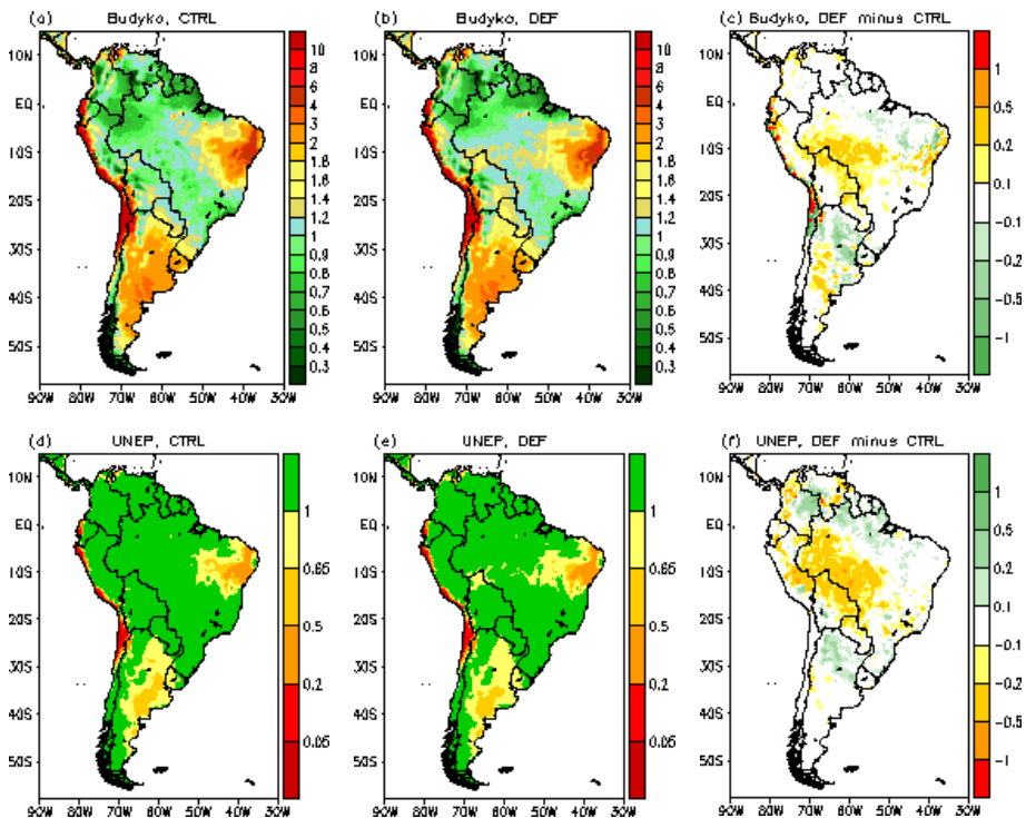
Figure 3. Distribution of aridity using Budyko index: a) control experiment, b) deforestation experiment and c) changes (deforestation minus control); and using UNEP index: d) control experiment, e) deforestation experiment and f) changes (deforestation minus control).
