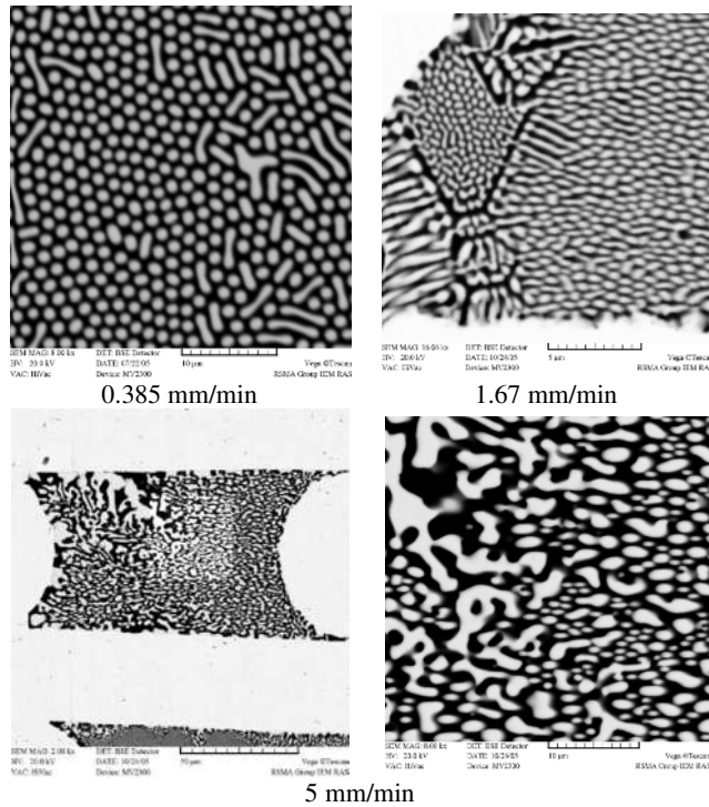
Figure 12. The microstructures of \text{Al}_2\text{O}_3\text{-GdAlO}_3 eutectic eutectic fibres crystallised with various pulling rates.
