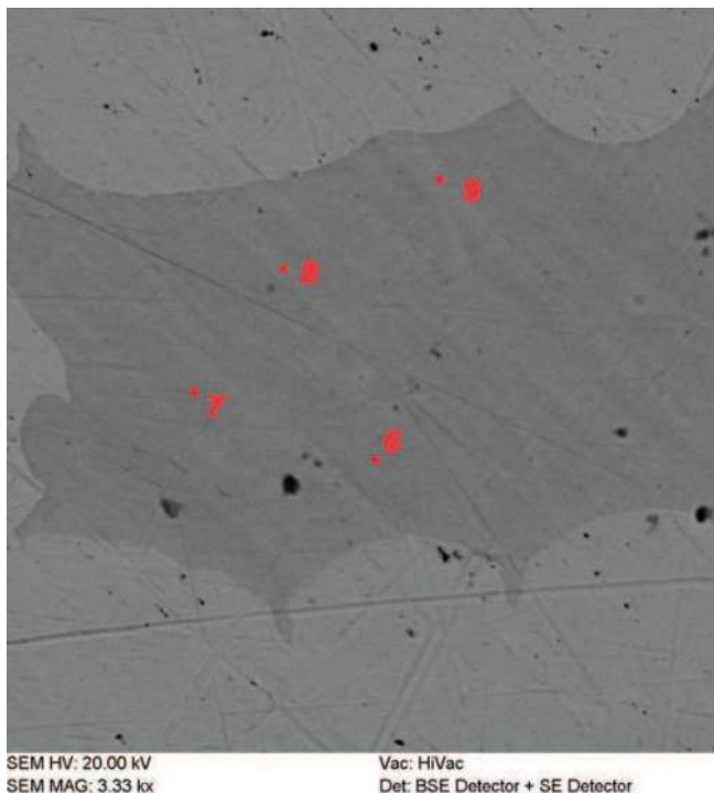
Figure 38. A typical microstructure of the molybdenum-silicide-fibre/molybdenum-matrix composite.
