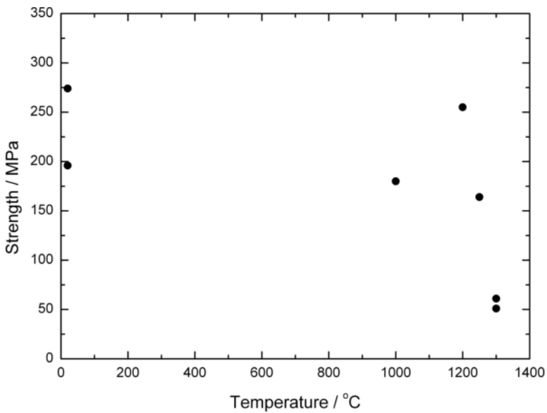
Figure 30. Temperature dependence of the bending strength of the composites reinforced with \text{Al}_2\text{O}_3\text{-Y}_3\text{Al}_5\text{O}_{12}\text{-ZrO}_2 -eutectic fibre. The fibre volume fractions are between 40 and 50%.
