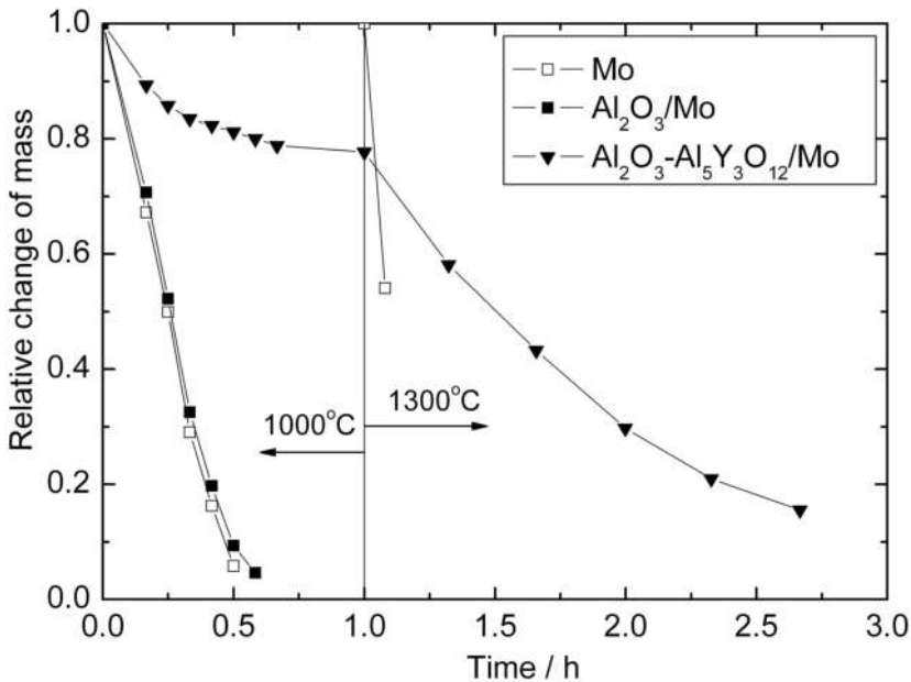
Figure 31. A relative decrease in the mass of molybdenum and oxide/molybdenum specimens with a surface of 20\text{ cm}^2 versus time of the exposure in air at 1000 and 1300^\circ\text{C} .
