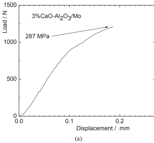
Figure 37. Load/displacement curve of a composite with brittle molybdenum matrix under 3-point bending (a); Failure surface of similar specimen with a fibre obtained from raw mixture \text{Al}_2\text{O}_3+2\%\text{CaO} at pulling rate of 1 mm/min.
