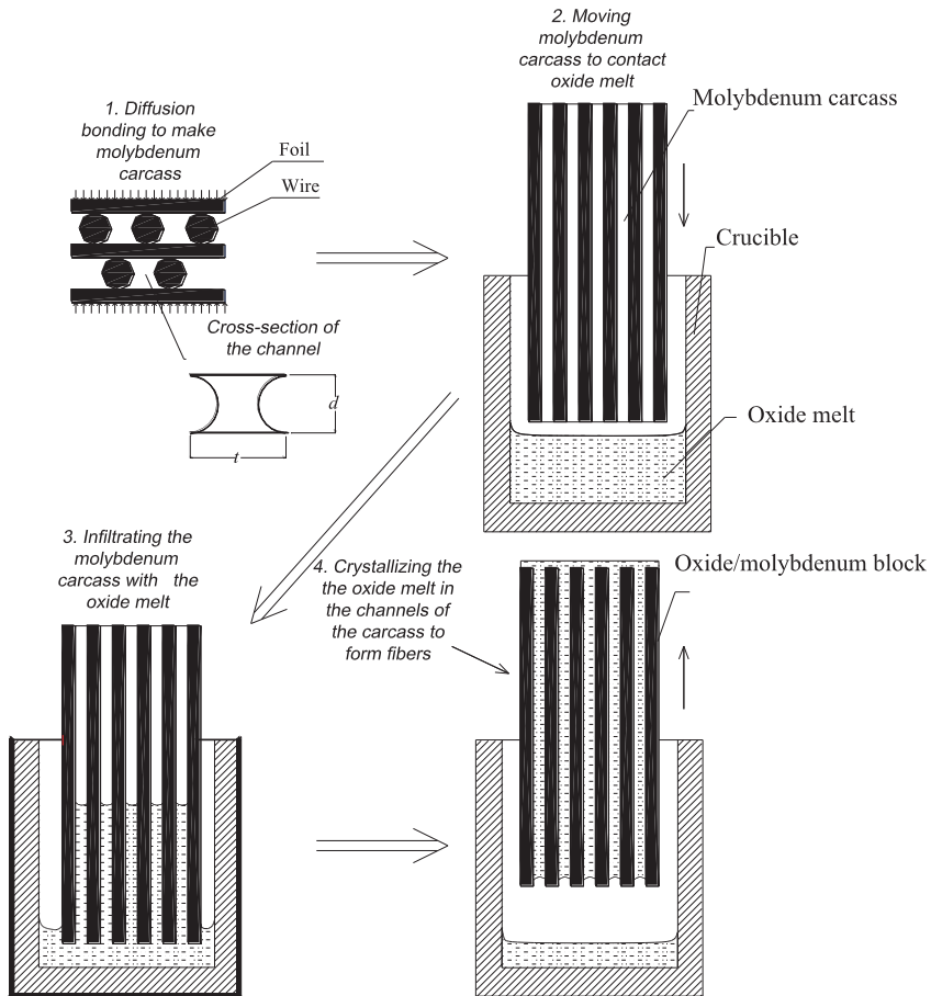
Figure 3. Schematic of the internal crystallization method (ICM).
