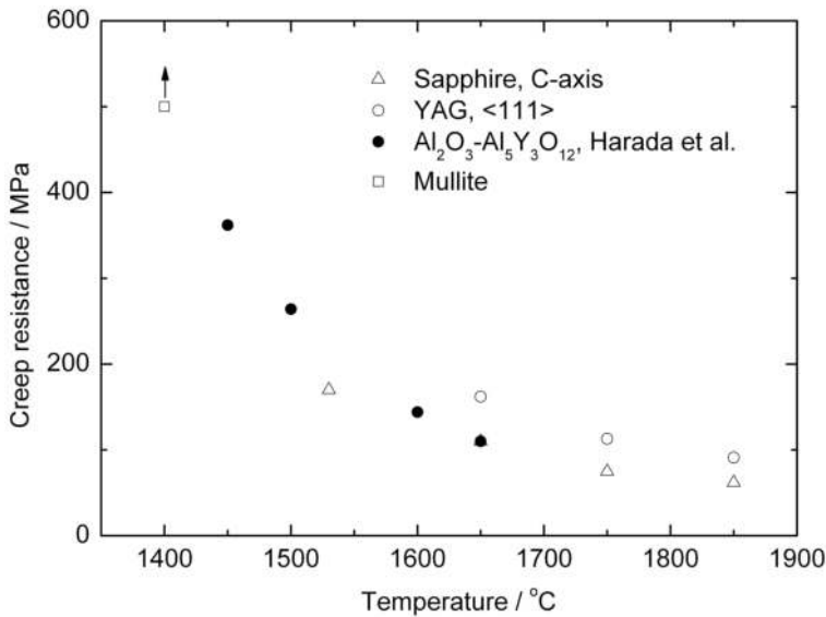
Figure 21. Temperature dependence of the creep resistance (a stress to cause 1% creep strain for 100 h) of some oxides in the form of bulk crystals. Data on sapphire and garnet YAG are after Corman [44], on mullite are after Dokko et al. [35], on Al 2 O 3 -Al 5 Y 3 O 12 -eutectics are after Harada et al. [45].
