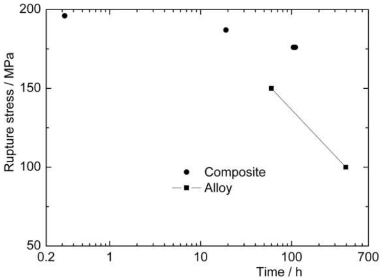
Figure 35. Creep strength of an \text{Al}_2\text{O}_3\text{-Y}_3\text{Al}_5\text{O}_{17}/\text{Mo} composite with fibre volume fraction of about 40% and that of most creep resistant three-phase Mo-Si-B alloy (acquired from experimental results in [11])
