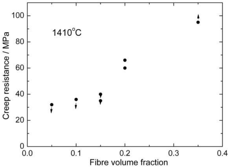
Figure 40. Creep resistance at 1410°C of Mo 3 Si-Mo composites versus fibre volume fraction.
