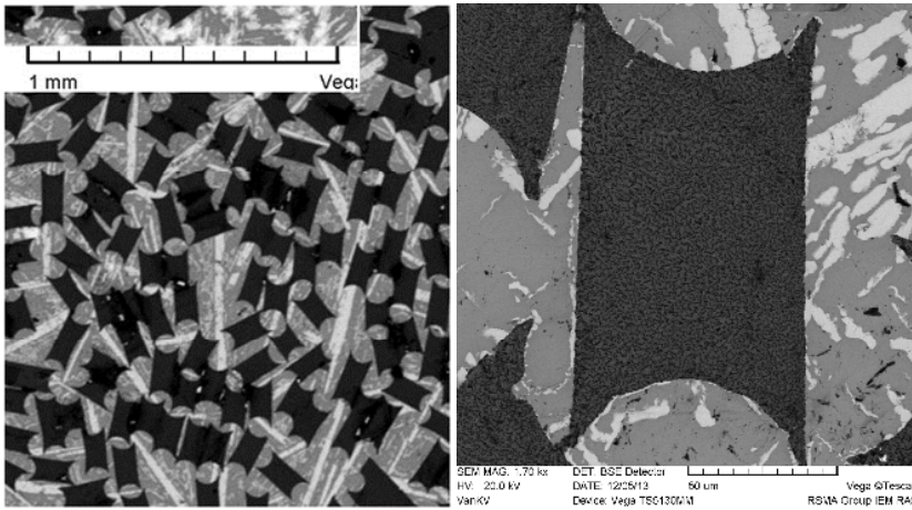
Figure 29. (a) A micrograph of a part of the cross-section of a specimen with \text{Al}_2\text{O}_3\text{-Y}_3\text{Al}_5\text{O}_{12} -eutectic fibre. (b) The microstructure at higher magnification.
