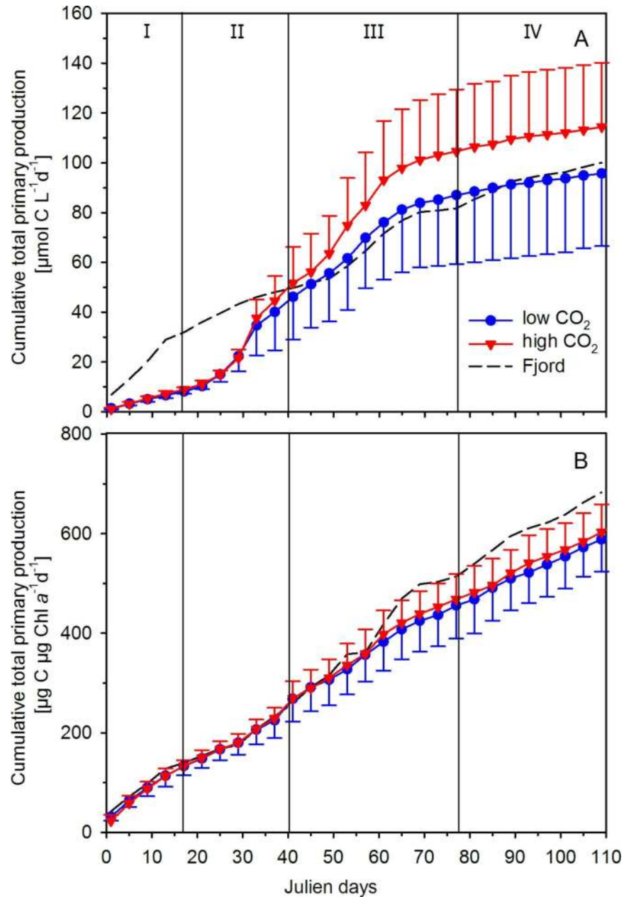
Fig 3. Cumulative total primary production (from 14 C-based 24 h incubations; A) and normalized to chlorophyll a concentrations (B) from mesocosm and fjord samples. Triangles (red; high p\text{CO}_2 ) and circles (blue; low p\text{CO}_2 ) represent the mean \pm SD of five biological replicates. Roman numbers denote the different phases of the experiment.
