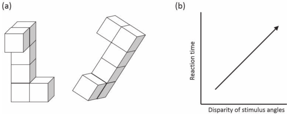
Figure 1. (a) MR task for three-dimensional objects: same-different judgment task. (b) The schematic linear relationship between reaction times (vertical axis) disparity angle of two objects (horizontal axis) [42].
