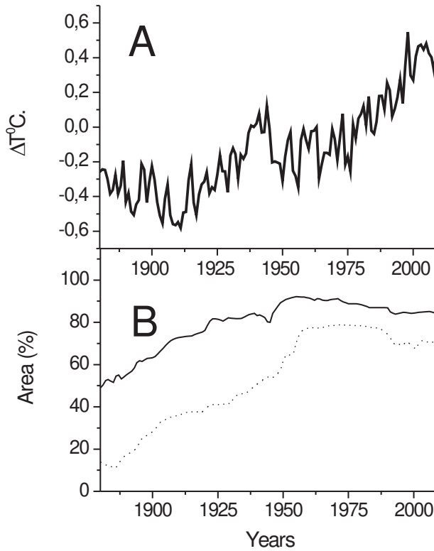
Figure 1. A – observed changes in a global average annual temperature ( http://www.cru.uea.ac.uk/cru/info/warming/ ). B – the percent of hemispheric area located within 1200 km of a reporting weather station. Solid line – Northern Hemisphere, dotted line – Southern Hemisphere. Data were electronically scanned from http:// data.giss.nasa.gov/gistemp/station_data/#form and digitized.
