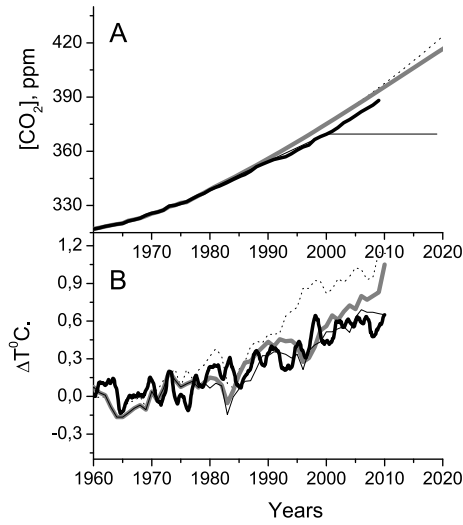
Figure 10. A – Concentration of CO 2 in the Earth’s atmosphere: black thick line – experimental measurement at Mauna-Loa ( www.esrl.noaa.gov/gmd/ccgg/trends/ ), dotted line – scenario A by Hansen et al. [35], gray line – scenario B [35], black thin line – scenario C [28]. B – Global surface temperature computed for scenarios A, B, and C, compared with observational data: black thick line – instrumental measurement ( ftp://ftp.ncdc.noaa.gov/pub/data/anomalies/monthly.land_ocean.90S.90N.df_1901-2000mean.dat ), other lines – corresponding scenarios [35].
