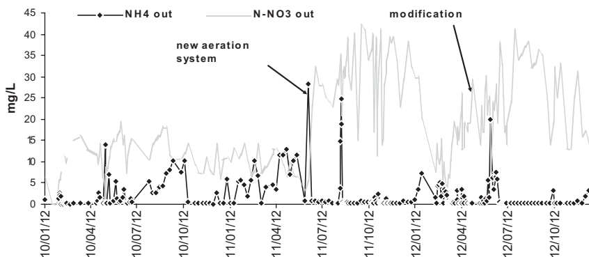
Figure 12.2 Concentration of NH 4 + and NO 3 -N in the effluent of WWTP 5 in 2010–2012 (Ragazzo et al. 2013).
