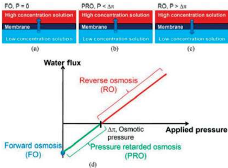
Figure 1. Illustration of FO, PRO, and RO processes [22].
