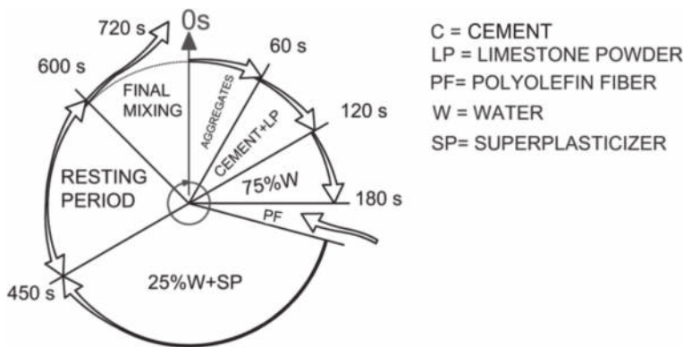
Figure 5. Mixing sequence of a polyolefin fibre-reinforced concrete.
