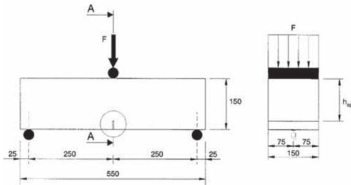
Figure 11. Test set-up in [38]. Measures in mm.
