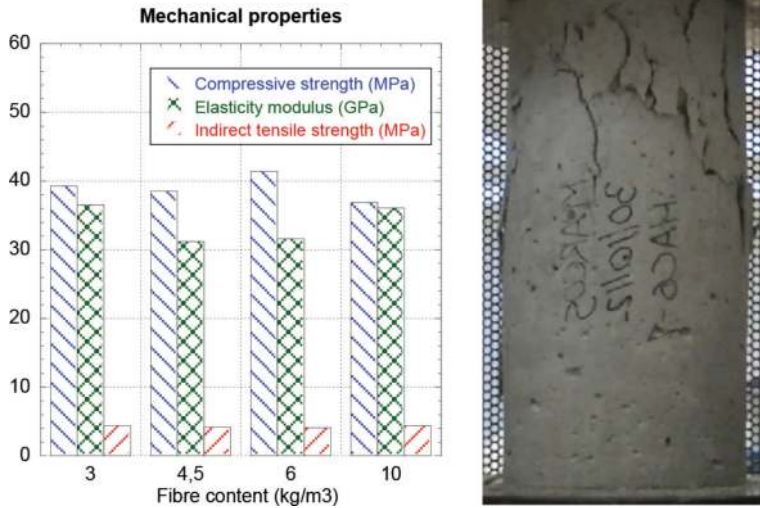
Figure 8. Mechanical properties and compressive strength sample after testing.
