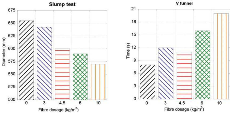
Figure 7. Slump test in an SCC PFRC [28].
