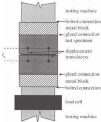
Figure 10. Uni-axial tension testing for concrete [30].
