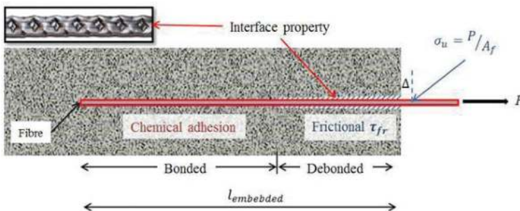
Figure 3. Pull-out mechanisms [8, 28].
