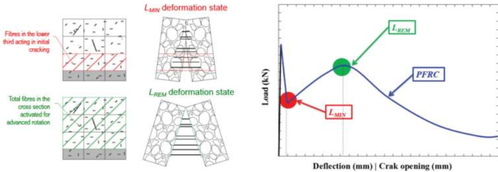
Figure 15. Deformation states of SLS or ULS.
