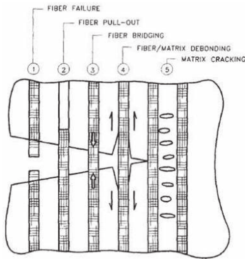
Figure 2. Energy absorbing the fibre matrix mechanisms [29].
