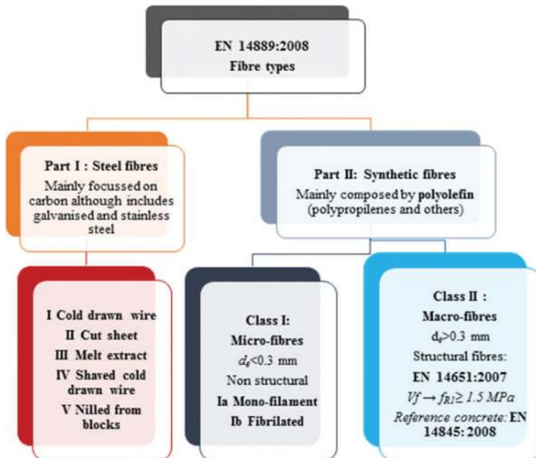
Figure 1. Fibre classification following EN-14889 [13].
