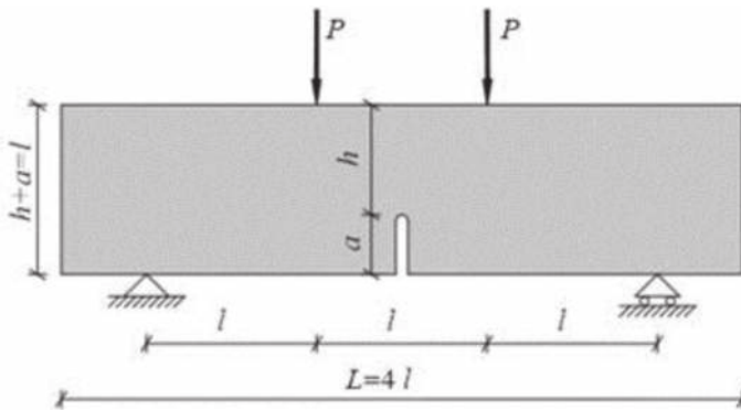
Figure 12. Four-point bending test [38, 46].
