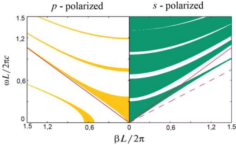
Figure 7. Dispersion diagrams of the magnetophotonic crystal containing plasma layers.
