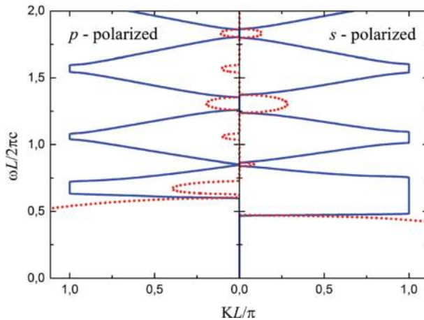
Figure 2: Dispersion characteristics of the one-dimensional photonic crystal.
