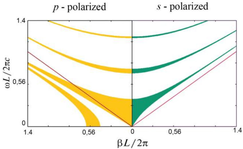
Figure 3. Dispersion diagrams for both polarizations.
