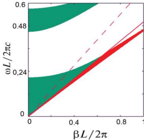
Figure 8. Band structure of the ferrite magnetophotonic crystal.
