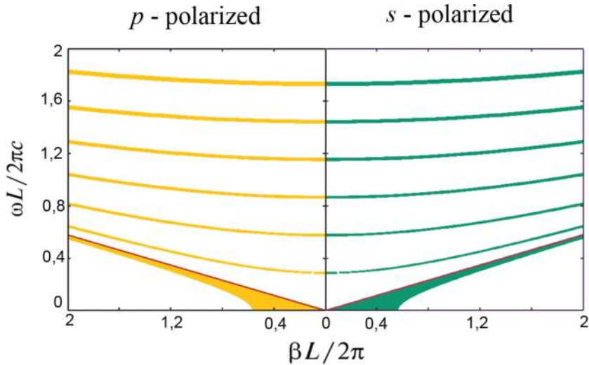
Figure 4. Dispersion diagram of the photonic crystal with metamaterial layer.
