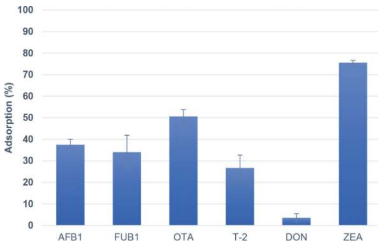
Figure 4. Percentage of adsorption of different mycotoxins on chitosan. Bars are the mean values. Error bars displays an interval around each mean, which are based on Fisher's least significant difference (LSD) procedure.
