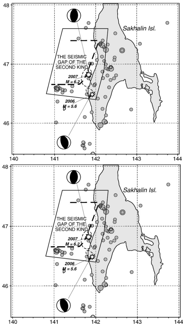
Fig. 17. Map of crust earthquake M \geq 3.0 epicenters, 1993–2005, recorded by the “Datamark” network of stations and the “IRIS-2” system, installed at the “Yuzhno-Sakhalinsk” seismic station. Note: the area of the seismic gap of the second kind is outlined with the bold dash line, while the source zones of the 17 August 2006, Mw 5.6 Gornozavodsk and the 2 August 2007, Mw 6.2 Nevelsk earthquakes, with a thin dash line; asterisks indicate the epicenters of main shocks; focal mechanisms are given based on data from [http://www.globalcmt.org]. The area limited by the polygon is the geographical area within which a large earthquake M=6.6 \pm 0.6 may occur.
