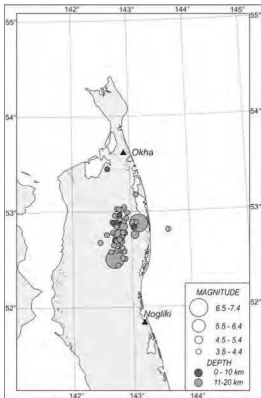
Fig. 10. Epicenters of the May 27, 1995 Mw 7.1 Neftegorsk earthquake and first-day aftershocks of magnitude M \geq 3.5 .
