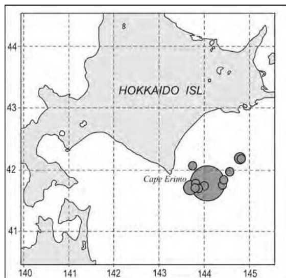
Fig. 14. Map of the 26 September, Mw 8.3 Tokachi-oki earthquake epicenter (large circle) and its first-day aftershocks of magnitude M \geq 5.0 (small circles).
