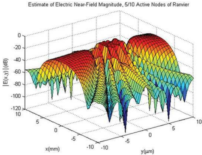
Figure 7. Extracellular region electric near-field magnitude, sparse Array.
