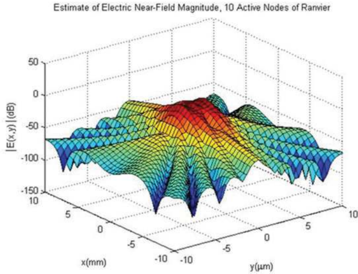
Figure 6. Extracellular region electric near-field magnitude, full Array.
