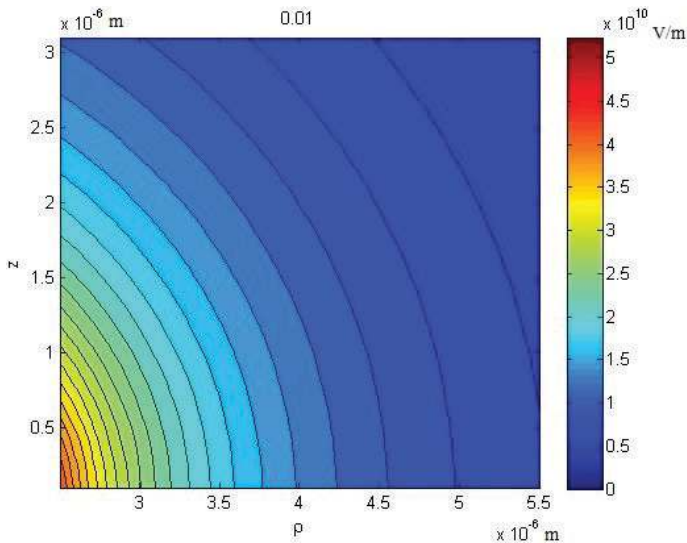
Figure 11. Snapshot of the time-varying electric near-field generated due to a ring of voltage-gated ion channels in a node of Ranvier. Video of time-varying field and clinical measurements available from the author.
