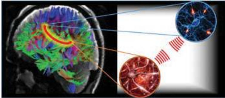
Figure 8. Electric near-field wireless network augmentation of the human Connectome.
