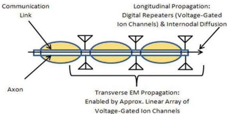
Figure 2. Axonal EC longitudinal Classical Channel and EM Transverse Channel (small triangular shapes positioned at nodes of Ranvier are symbols for antenna elements).
