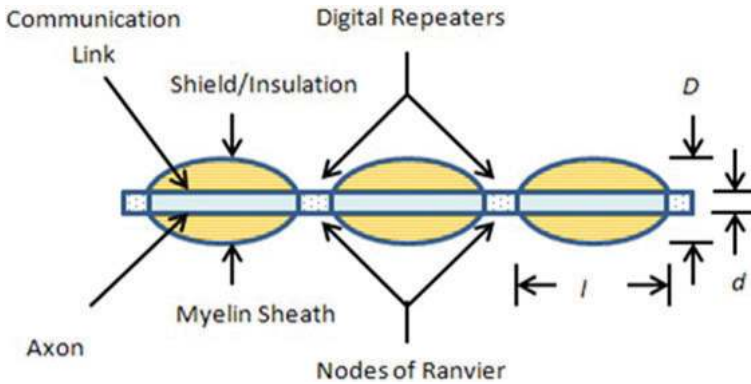
Figure 1. Elements of a Myelinated axon.
