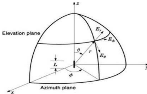
Figure 5. Electric field geometry and components.
