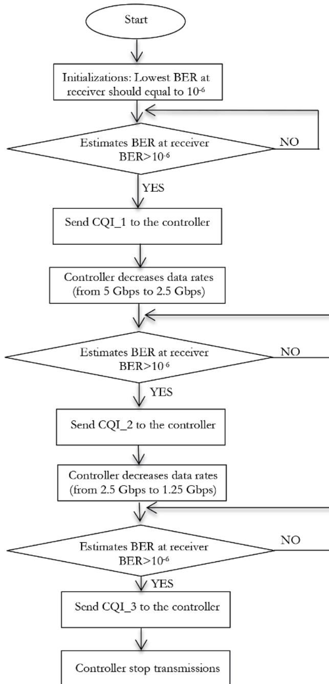
Figure 7. Flow chart of ART (down convert case).
