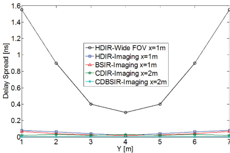
Figure 11. Delay spread of IROW proposed systems.
