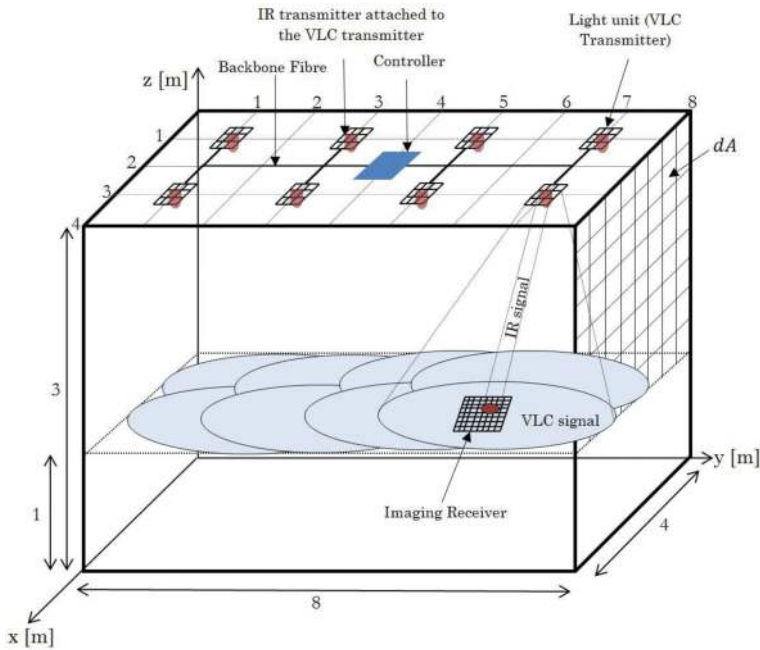
Figure 6. Architecture of VLC/IROW collaborative system.
