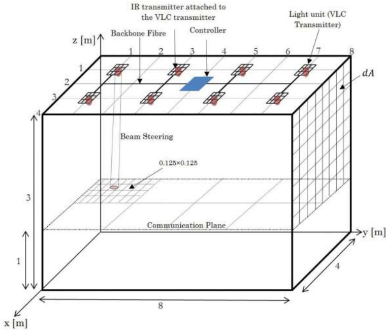
Figure 5. Architecture of CDBSIR system.
