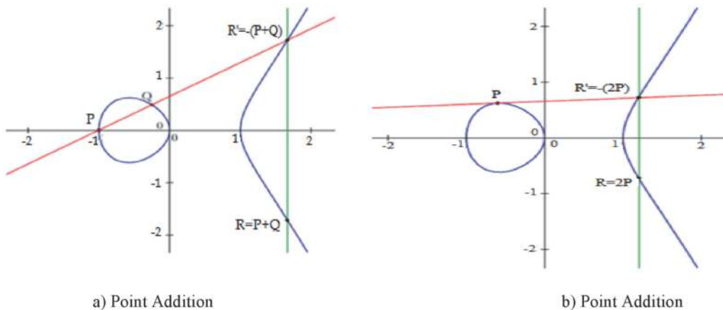
Figure 2. Point addition and point doubling operations.
