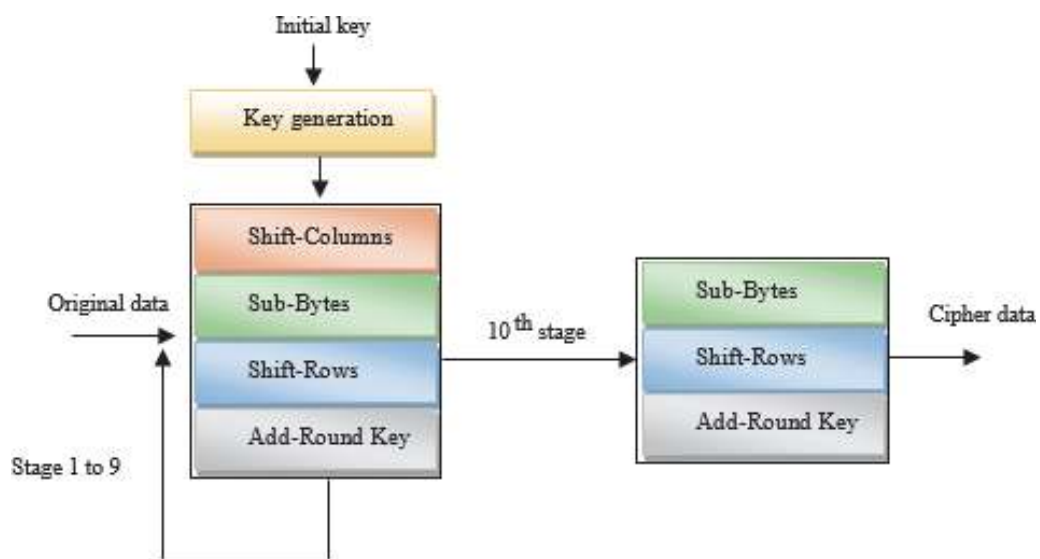
Figure 1. Flow design of AES algorithm.
