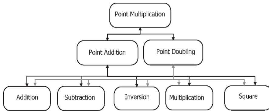
Figure 3. Hierarchy of scalar multiplication.
