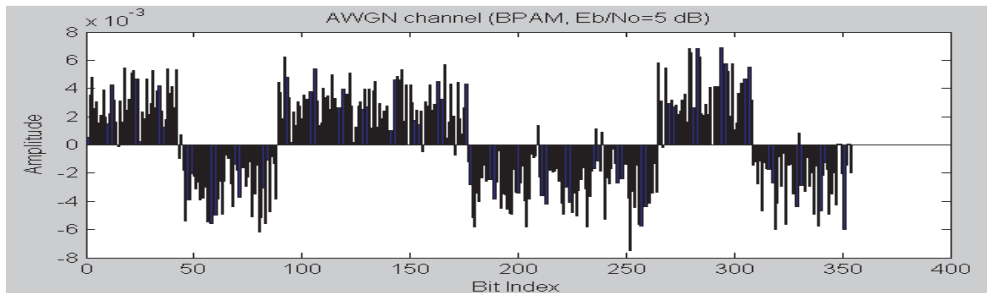
Fig. 4.9. AWGN channel output (BPAM), where E_b/N_0=5 dB.
