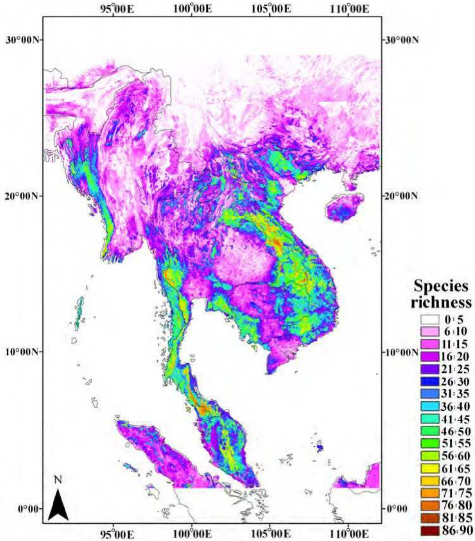
Fig. 1. The current projected species richness for 171 Southeast Asian bat species on a km 2 basis. Projections were generated using Maxent, methods are shown in Box 1. Environmental variables used in projections are included in Appendix 1.
