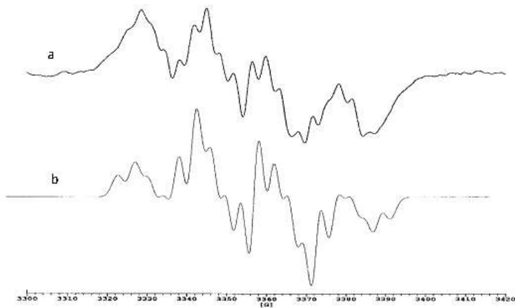
Figure 11. EPR spectra of ^{60}\text{Co} - \gamma irradiated 3NAP single crystal at 120 K when (a) the magnetic field is in the a^*c -plane and is away 165^\circ from the a^* -axis and (b) simulation of the spectrum; line width is 0.34 mT.
