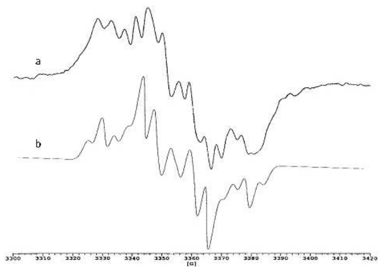
Figure 9. EPR spectra of ^{60}\text{Co} - \gamma irradiated 3NAP single crystal at 120 K when (a) the magnetic field is in the a^*c -plane and is away 140^\circ from the a^* -axis and (b) simulation of the spectrum; line width is 0.38 mT.
