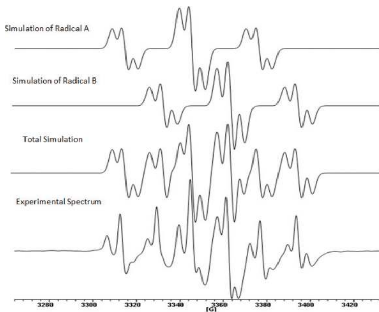
Figure 5. Experimental and simulated EPR spectra of gamma-irradiated succinic anhydride single crystal at 125 K when the magnetic field is in the bc plane at an angle 90^\circ toward the axis.
