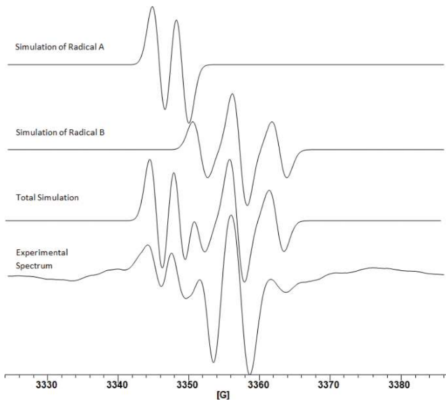
Figure 2. EPR spectrum of gamma-irradiated PHM single crystal at 125 K when the magnetic field is in the ab plane at an angle 0^\circ toward the axis.
