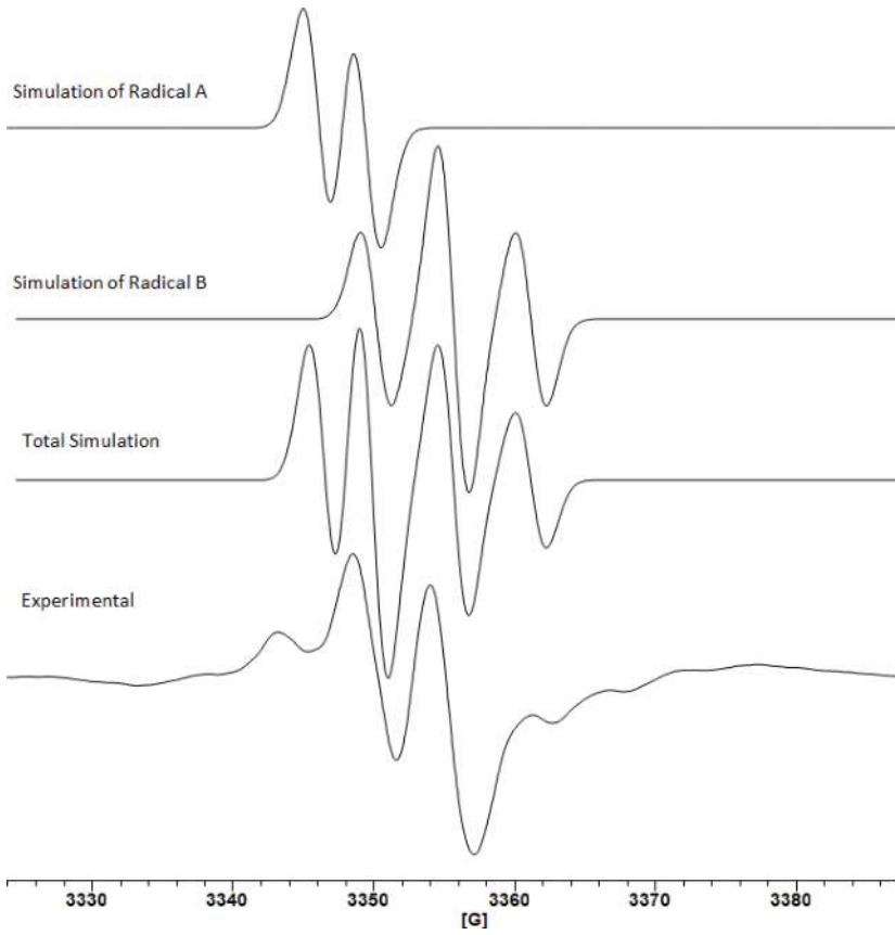
Figure 3. EPR spectrum of gamma-irradiated PHM single crystal at 125 K when the magnetic field is in the ac plane at an angle 70° toward the axis.
