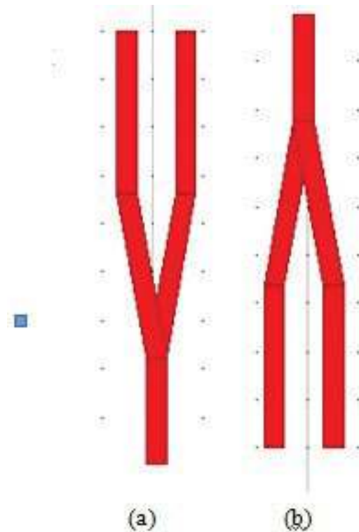
Figure 1. Y branches (a) Branch [1-2] (b) Branch [2-1].
