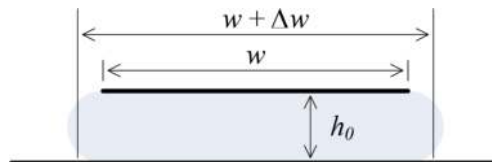
Figure 19. Schematic diagram of extended squeeze-film model.
