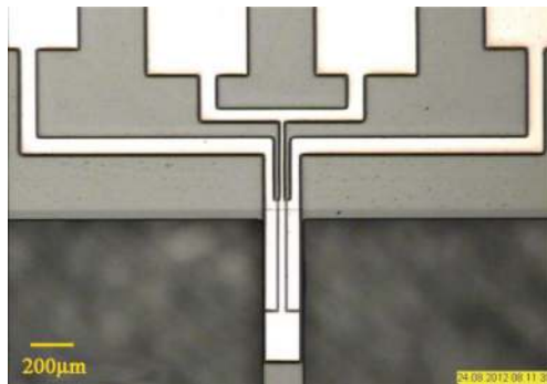
Figure 2. Micrograph of a piezoelectric resonator.
