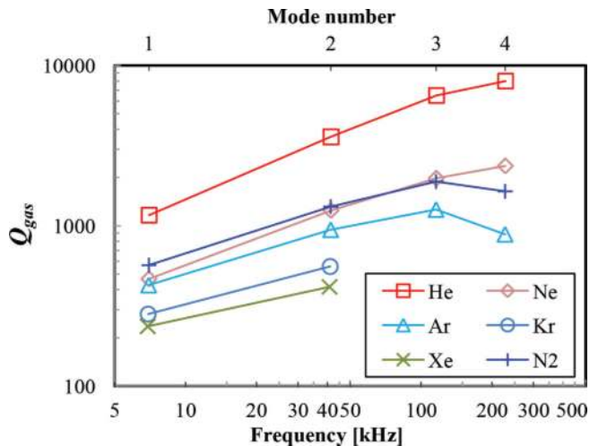
Figure 13. Q factors due to gas damping of the different flexural modes at atmospheric pressure [25].
