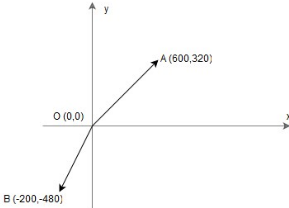
Figure 3.14: Quiver Plot.
