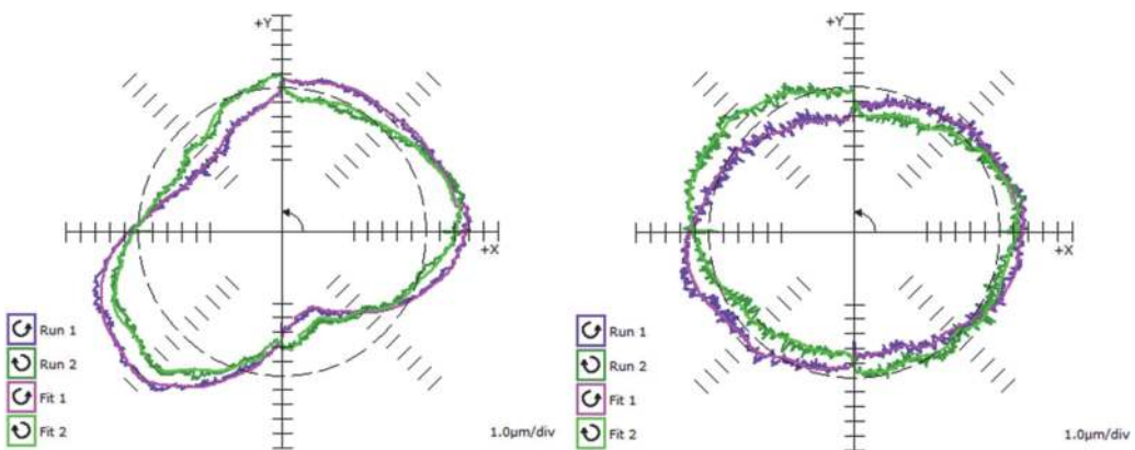
Figure 10. Accuracy of circular interpolation in XY plane before and after volumetric compensation [13].
