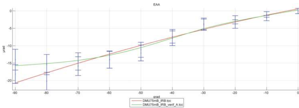
Figure 11. Error of EAA axis A [13].
