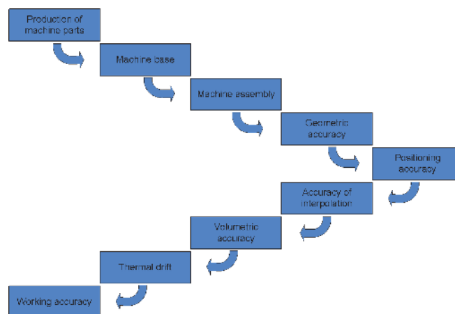
Figure 13. Cascading of accuracies in machine tools [13].
