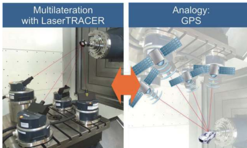
Figure 4. Principle of measurement with LaserTRACER [etalon].
