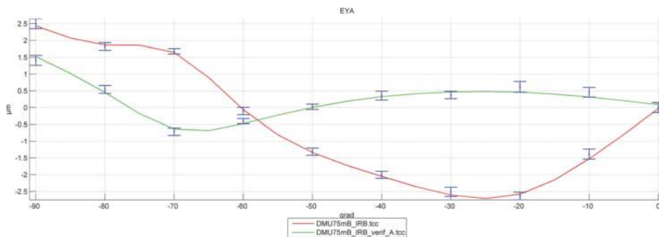
Figure 12. Error of EYA axis A [13].
