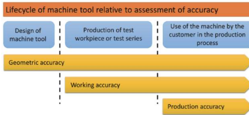
Figure 6. Relationships between individual accuracies of a CNC machine tool throughout its life cycle.
