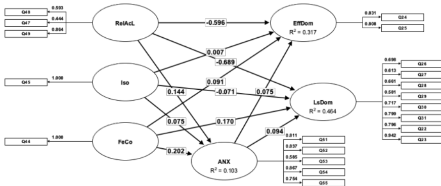
Figure 2. The results of the full SEM
