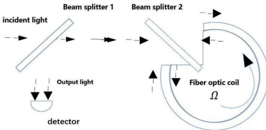
Figure 2. The basic composition of FOG.
