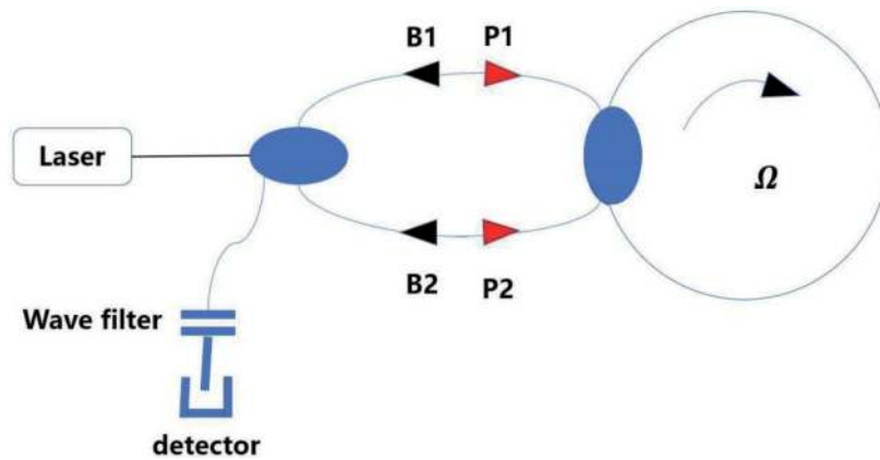
Figure 5. The principle diagram of stimulated Brillouin FOG.
