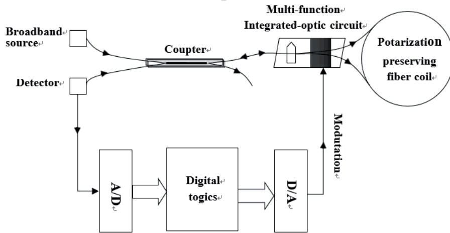
Figure 2. The basic composition of FOG.
