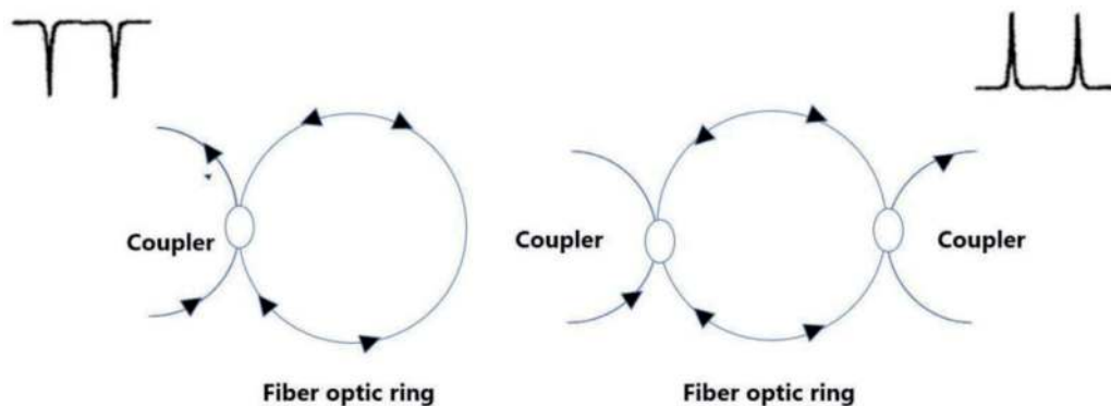
Figure 4. The reflective resonator.
