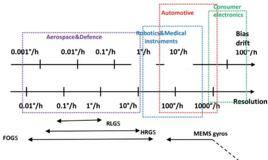
Figure 1. The application requirements of different FOGs.
