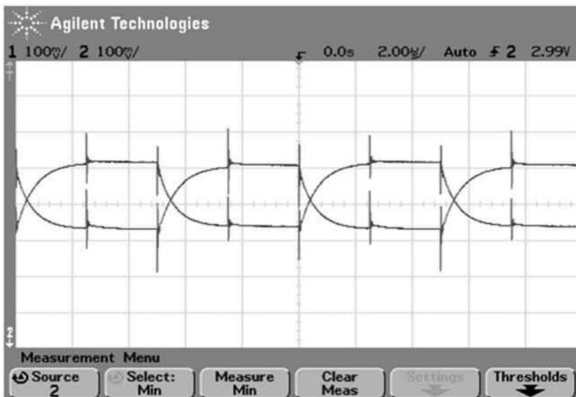
Fig. 18. The measured output waveform of two neighboring channels under dot inversion for the RGB digital inputs of '000000000', where the voltage levels for negative and positive polarities are 2.425 V and 2.598 V, respectively.
