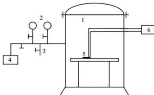
Figure 10. Detection test device for the CNTs sensor adsorbing gases dissolved in transformer oil. 1: sealed metal can, 2: vacuum gauge and pressure gauge, 3: intake valve, 4: vacuum pump, 5: CNTs sensors, 6: impedance analyzer.
