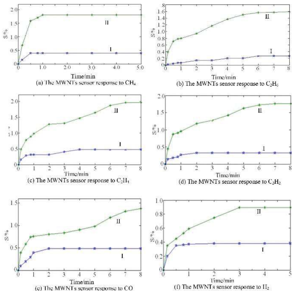
Figure 11. The MWNTs sensor response to \text{CH}_4 , \text{C}_2\text{H}_2 , \text{C}_2\text{H}_4 , \text{C}_2\text{H}_6 , \text{CO} , \text{H}_2 .
