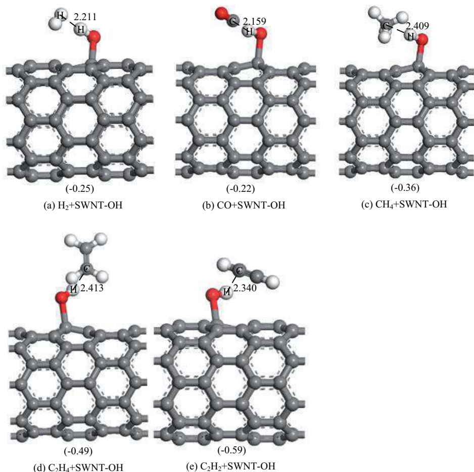
Figure 5. The most stable configurations of \text{H}_2 , \text{CO} , \text{C}_2\text{H}_4 , and \text{C}_2\text{H}_2 interacting with SWNT-OH after optimization, respectively.
