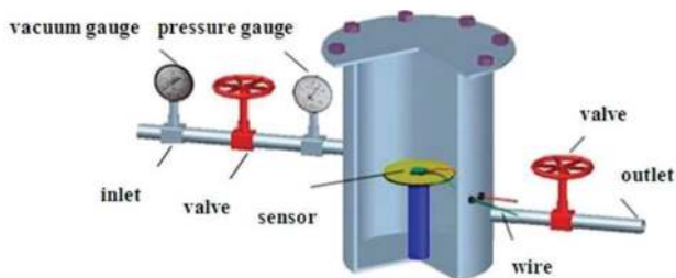
Figure 12. Geometry of the experimental equipment.
