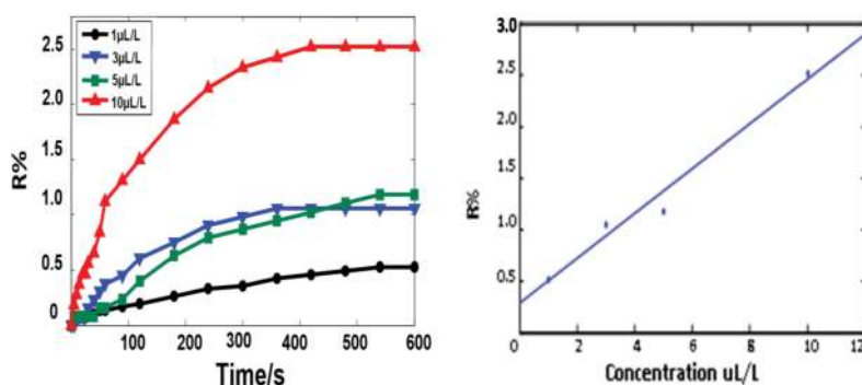
Figure 14. The gas response of Ni-CNTs sensors to different concentrations of C_2H_2 . (a) Gas response curve to different concentrations of C_2H_2 , (b) linear fitting curve.
