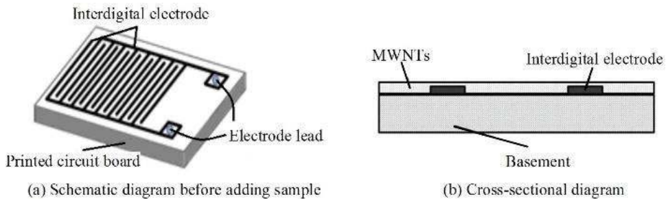
Figure 9. The geometric sketch of CNTs sensor.
