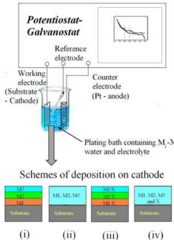
Figure 3. Schemes of cathodic electrodeposition of precursor film to be post annealed (EDA) for p-type photovoltaic absorber layers in literatures. Here, M_i represent constituent metal and X represents oxidized anion.
