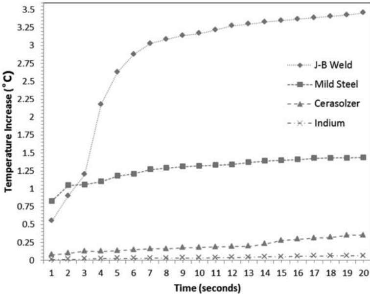
Figure 4. The average recorded temperature increase using the TPS sensor type 7577 for the samples made from mild steel, indium, J-B weld epoxy steel resin and Cerasolzer CS186.
