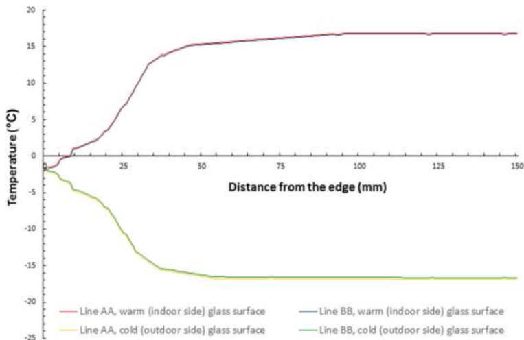
Figure 6. The temperature loss, due to a wider edge seal, along the glazing surface lines AA and BB showing the temperature gradient from the glazing edge to the central area of the glazing of the one quarter of total sample of 300 \times 300 mm using ASTM boundary conditions.
