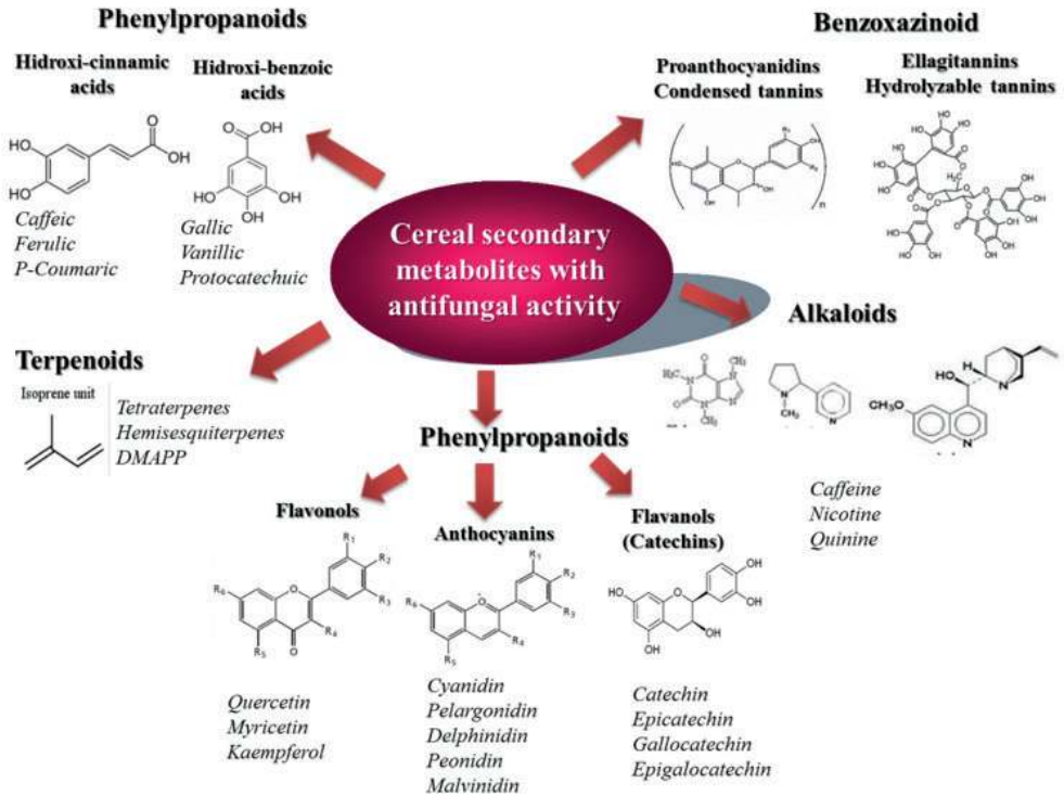
Figure 2. Cereal secondary metabolites with antifungal activity.
