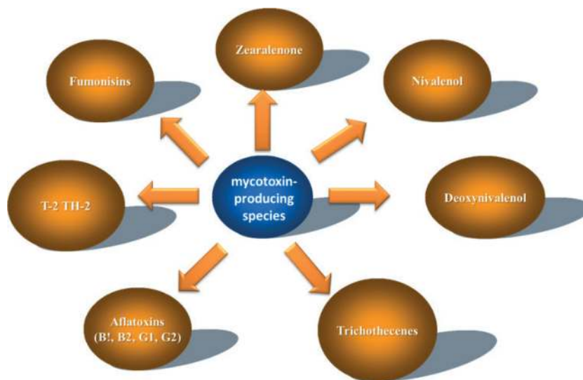
Figure 1. Group of mycotoxin-producing species.
