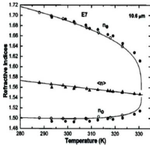
Figure 5. Temperature-dependent refractive indices of E7 at 10.6 \mu\text{m} . The filled circles are the refractive indices measured by the wedged LCell refractometer method. The filled triangles are the average refractive index calculated by the experimental data. The open circles represent n_o and n_e extrapolated from the experimental data measured at visible spectrum using the extended Cauchy model. The open triangles are the average refractive index calculated by the extrapolated n_e and n_o , respectively. The solid curves are the fitting using Eqs. (10) and (11).
