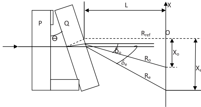
Figure 1. The used liquid crystal wedged cell.
