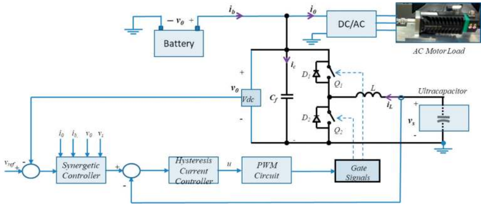
Figure 2. Block diagram of the proposed synergetic-based hybrid energy storage system.
