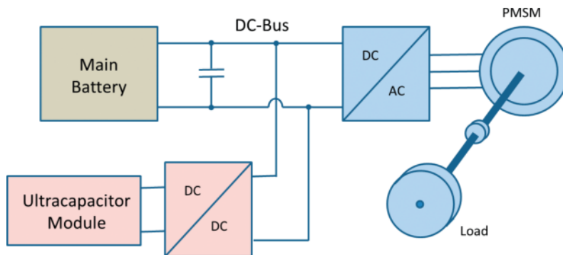
Figure 1. Topology of the hybrid energy storage system.
