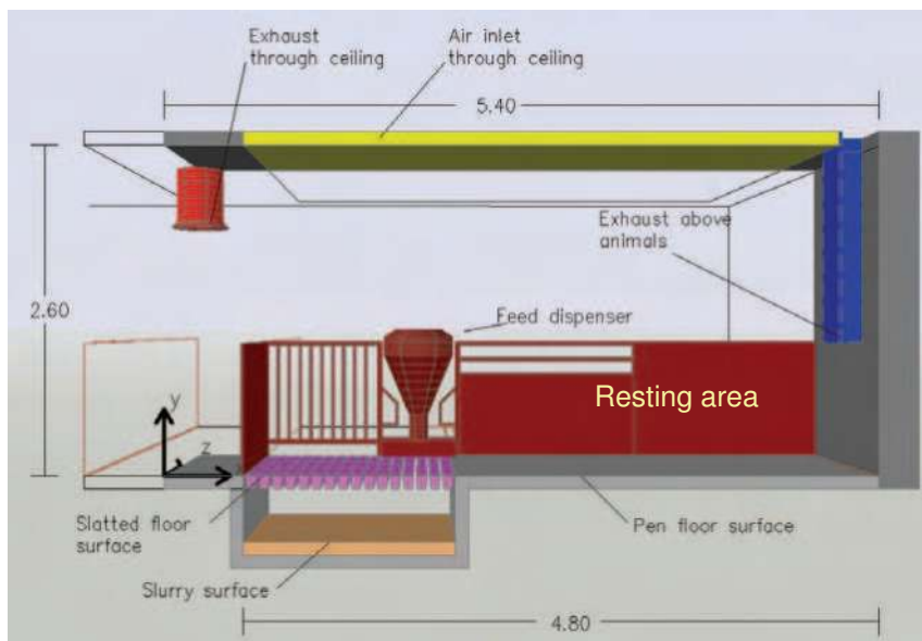
Fig. 12. Pig unit with two alternative ventilation exhausts (through ceiling or above animals).
