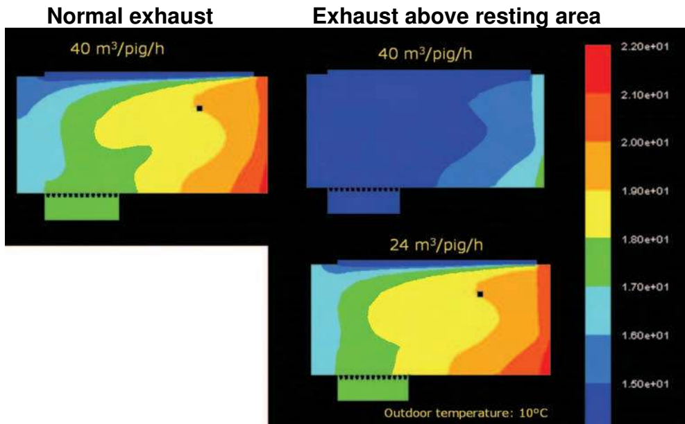
Fig. 13. CFD prediction of temperature distributions ( ^{\circ}\text{C} ) in a pig pen at different exhaust locations and air changes.
