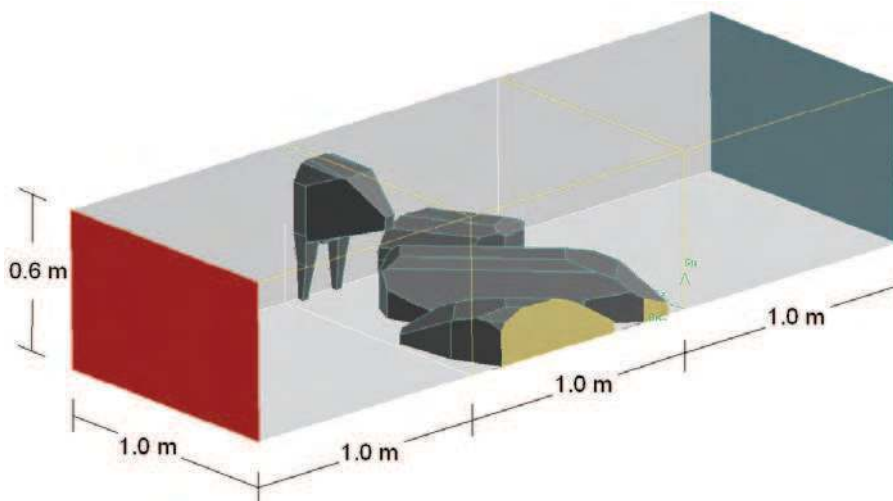
Fig. 7. Geometrical model used in simulation for determination of flow resistance through animal occupied zone with animal density of 2.1 laying and 0.26 standing 50 kg pig pr m 2 . Velocity inlet and pressure outlet boundary condition were assumed at the left and right face, respectively.
