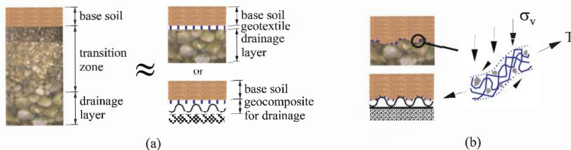
Figure 1. Granular vs. geotextile filter. (a) Idealization; (b) Actual working condition of a nonwoven geotextile.
