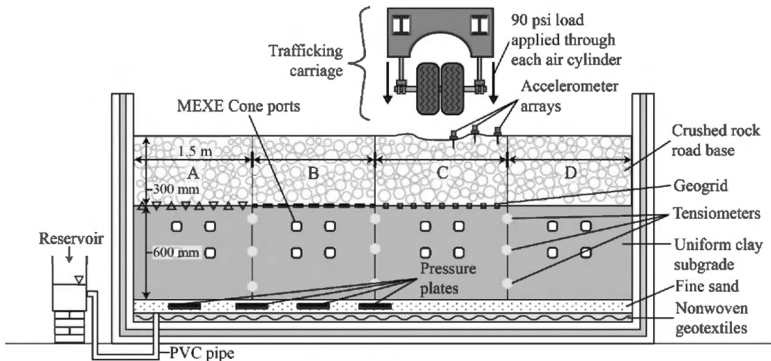
Figure 2. Full-scale wheel trafficker system.
