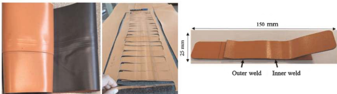
Figure 1. Dual-track geomembrane seam sample and seam specimen.
