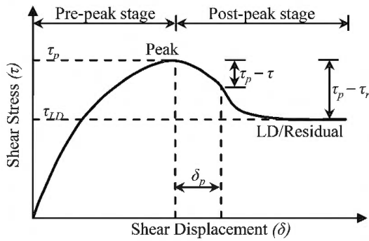
Figure 4. Generalized stress–displacement relationship for clay–geosynthetic interface.
