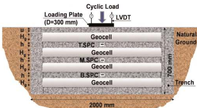
(a) Schematic cross-section of the test set-up (not to scale), “T.SPC”, “M.SPC”, and “B.SPC” indicate the location of soil pressure cells, (b) Photograph of test installation prior to loading include reaction beam, load plate, hydraulic jack and three dial gauges (Moghaddas Tafreshi et al. 2013).
