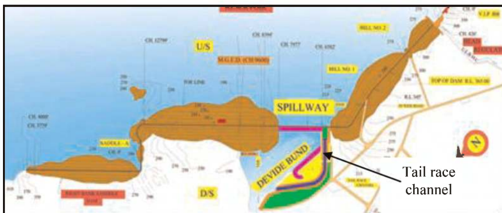
Figure 2. Layout of Ukai dam (Kapadia 2022).
