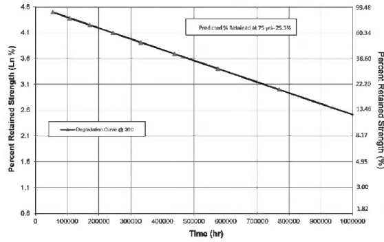
Figure 3. Degradation curve of Geogrid A in pH 11.4.
