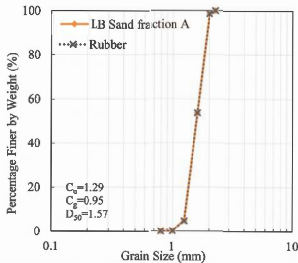
Figure 1. Particle size distribution for sand and rubber materials obtained from sieve analysis.
