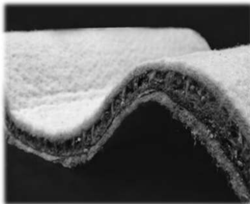
Figure 1. Sectional view of a cementitious geocomposite.
