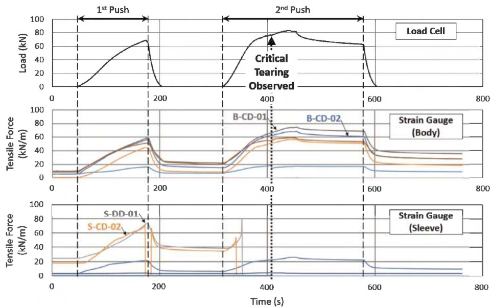
Figure 9. Results of inlet port test T3.
