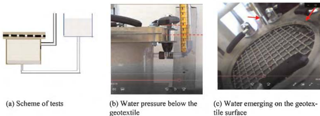
Figure 3. Views of the soil-geotextile test.
