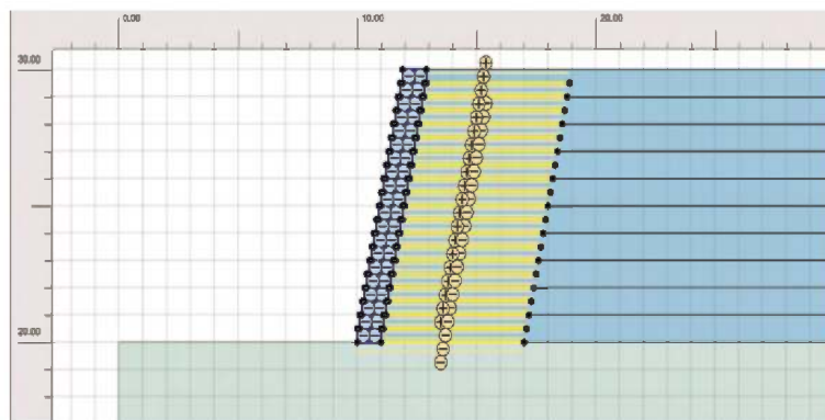
Figure 3. Interaction between soil and reinforcing elements.
