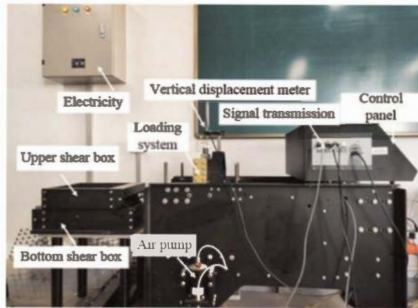
Figure 2. Schematic diagram of direct shear test system.
