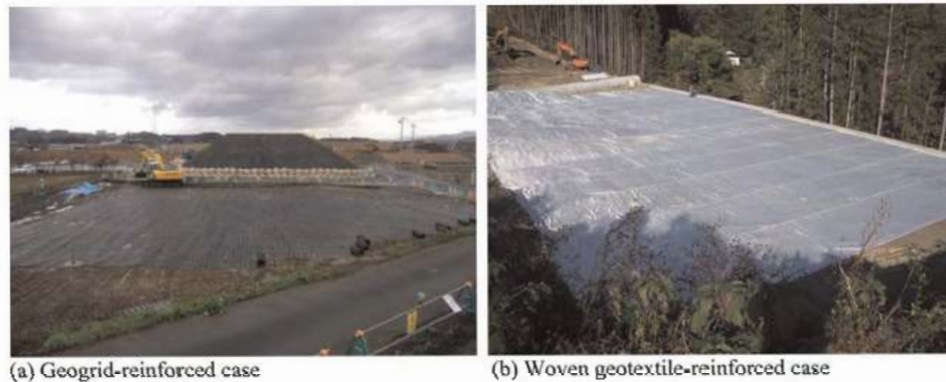
Figure 9. Geosynthetic reinforcement embankment applications in Japan.
