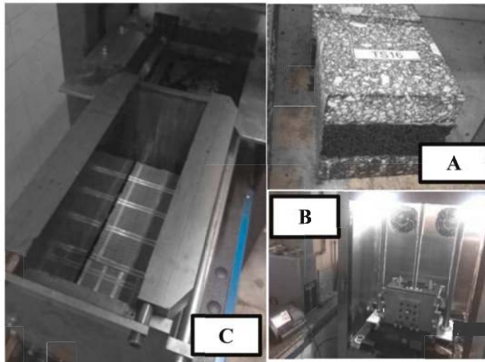
Figure 2. Specimen preparation and rutting test set-up.
