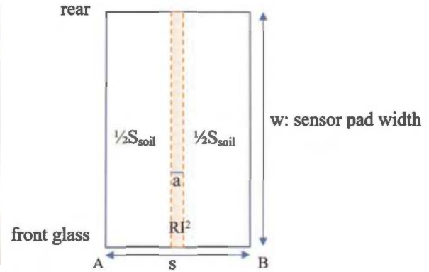
Figure 5. Central mesh of the RI^2 .
