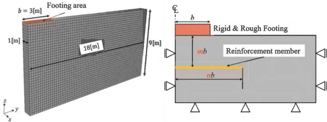
Figure 4. Finite element mesh and boundary conditions.
