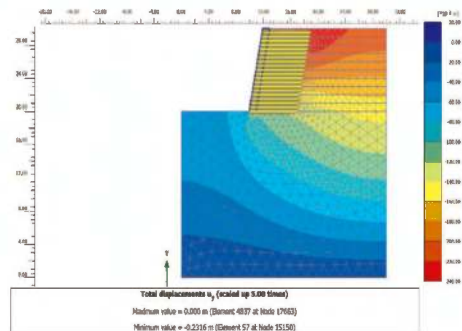
Figure 5. Horizontal displacement.
