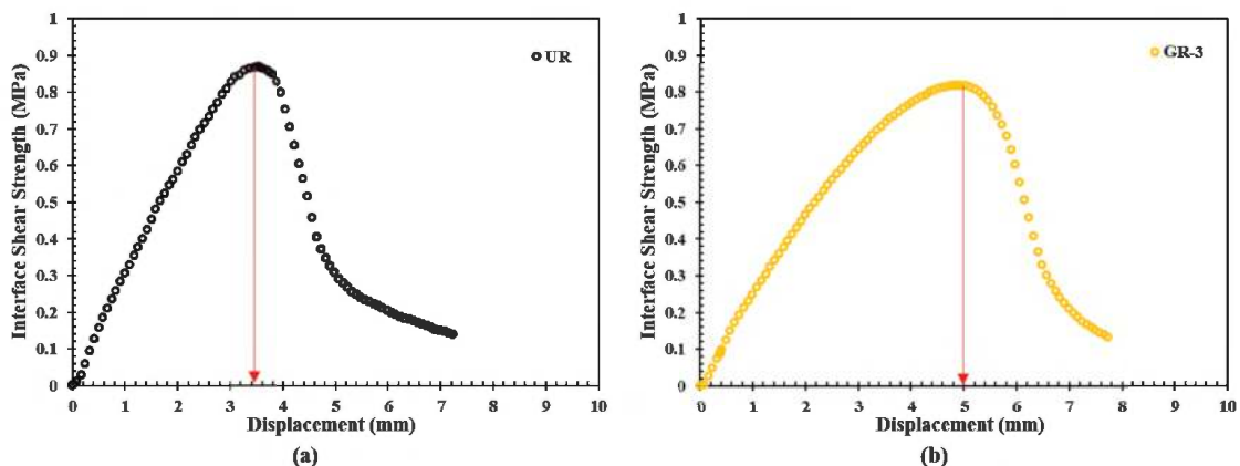
Figure 4. Typical interface shear strength trends: (a) Unreinforced specimen and (b) Geosynthetic-reinforced (GR-3) specimen.
