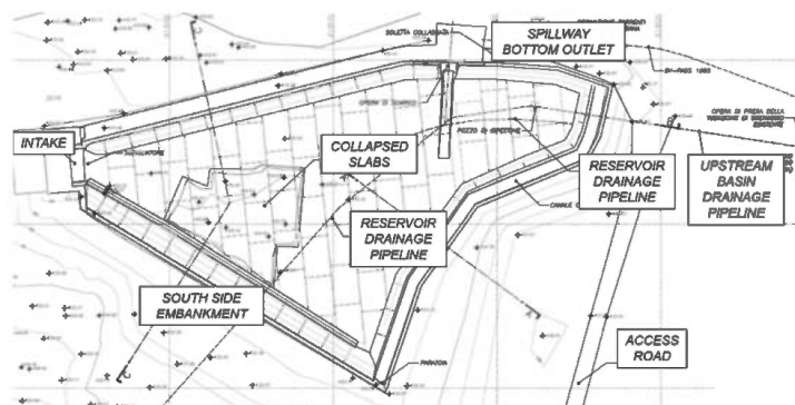
Figure 2. General plan of Sillico reservoir.
