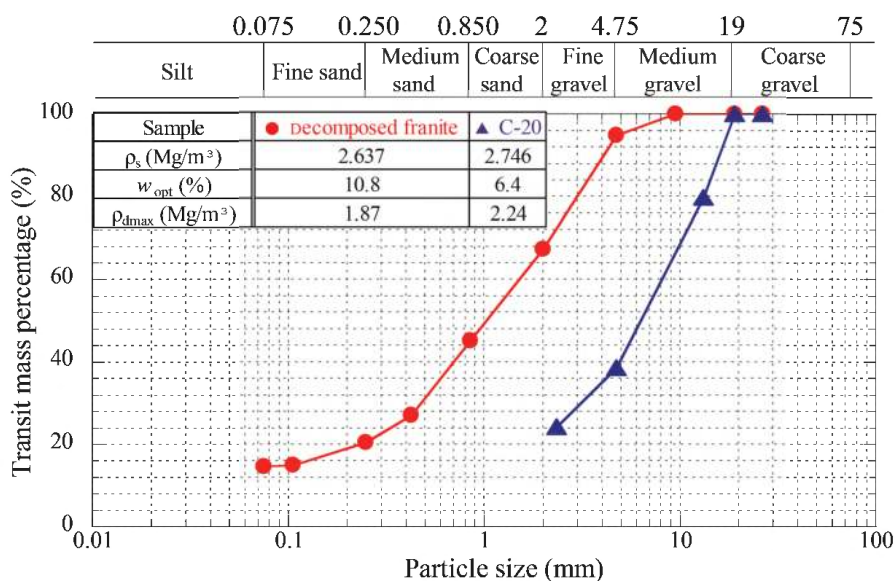
Figure 1. Grain size accumulation curve.
