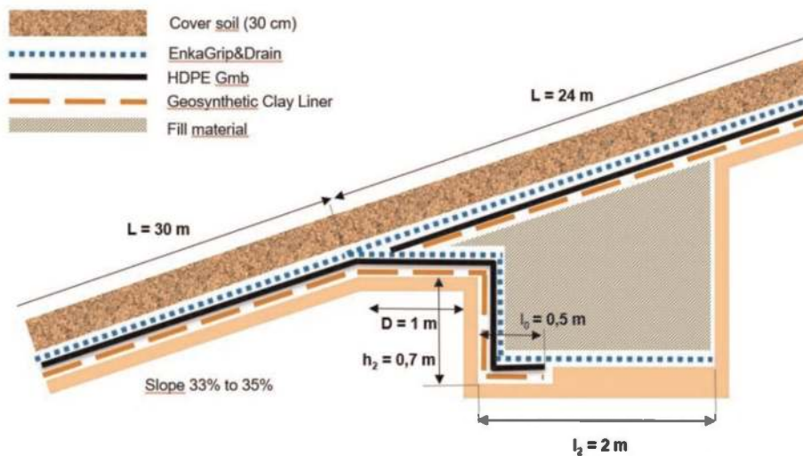
Figure 2. Details of the intermediate anchorage.
