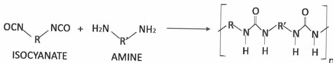
Figure 4. Polyurea reaction.
