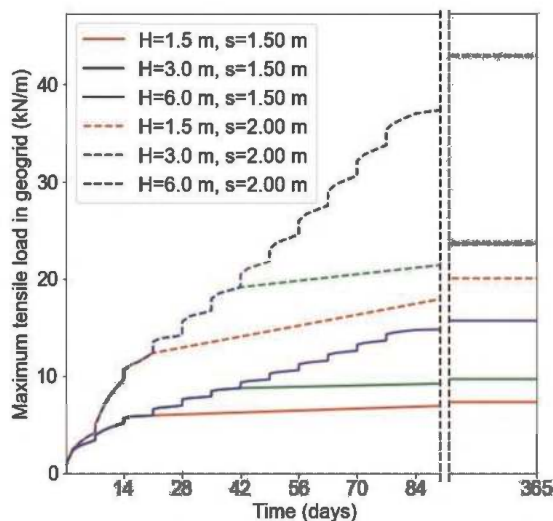
Figure 5. Maximum force in reinforcement.
