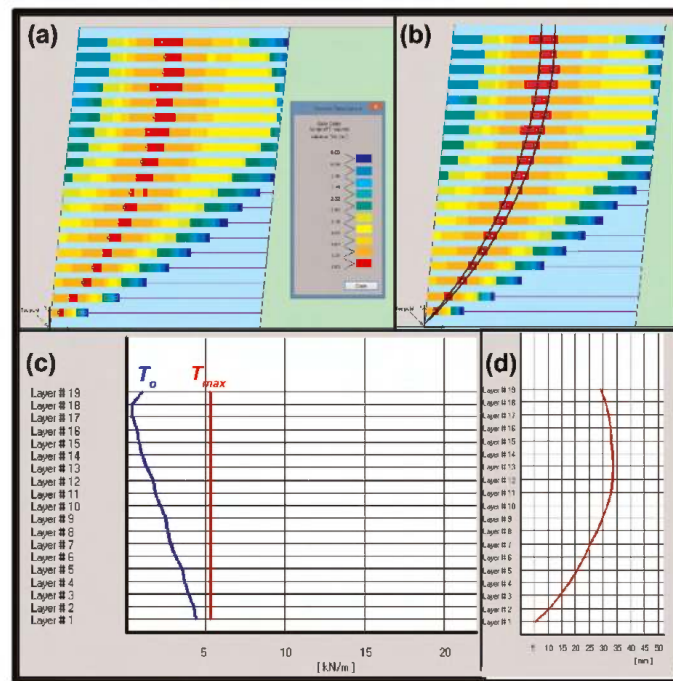
Figure 4. (a) Tension map for closely spaced reinforcement ( S_v=0.3m ) conditions. Note that the location of the maximum T_{max} on each layer is shown with a white, hollow marker. (b) Slip surfaces associated with maximum T_{max} . (c) Distribution of T_{max} and T_o along the profile of the given geometry. (d) Estimated lateral displacement profile based on a stiffness of J=500 kN/m.
