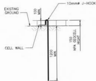
Figure 3b. Anchor design detail.
