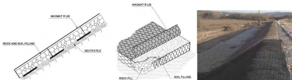
Figure 2. Maccaferri combo Reno Mattresses Plus.
