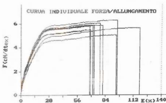
Figure 2. Fiber tenacity test result example.
