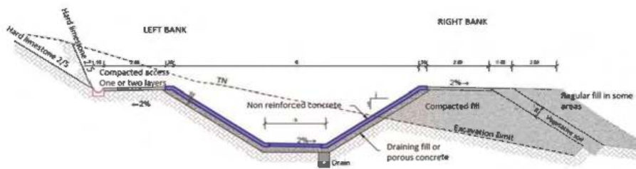
Figure 11. Cross-section type of the Canal de Provence.
