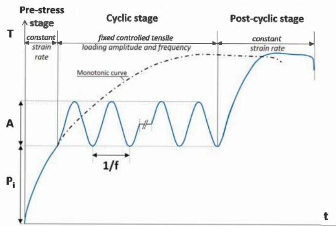
Figure 1. Multistage test procedure (Cardile et al. 2017b).
