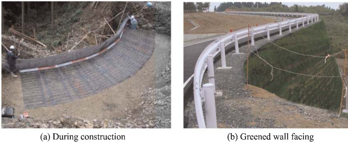
Figure 15. Greening technique combining geogrid and geotextile for geosynthetic MSE wall (courtesy of Dr. Hironaka).
