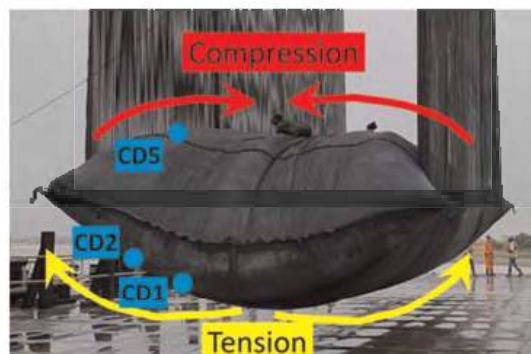
Figure 9. Deformation of geotextile tube during lifting.
