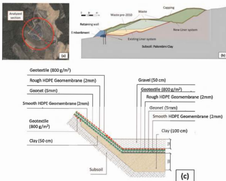
Figure 1. Landfill: (a) Chorography of the site (source “Google Earth”). In the red circle the site of the landfill; (b) Analyzed section; (c) Liner system details.
