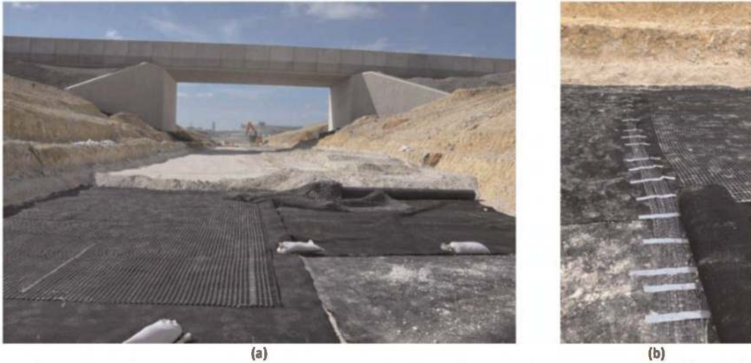
Figure 16: Installation of fibre optic-instrumented geogrid and supporting geogrid at Tilehouse Lane Cutting (Huesker Ltd.)
