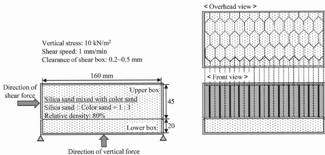
Figure 3. Physical model overview of geocell-reinforced soil.
