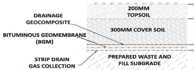
Figure 4. Schematic of Hervey Range Landfill BGM Cap.
