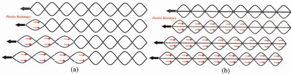
Figure 3. Plan view of deformation patterns and gradual mobilization of passive resistance during pullout: (a) along the typical diamond-shape (conventional); (b) along diagonally enhanced geocell.
