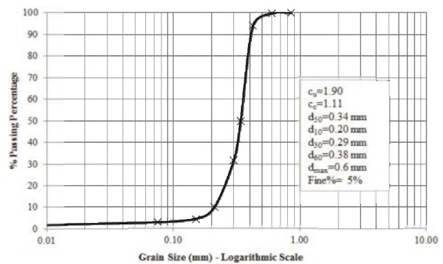
Figure 1. Particle size distribution analysis.
