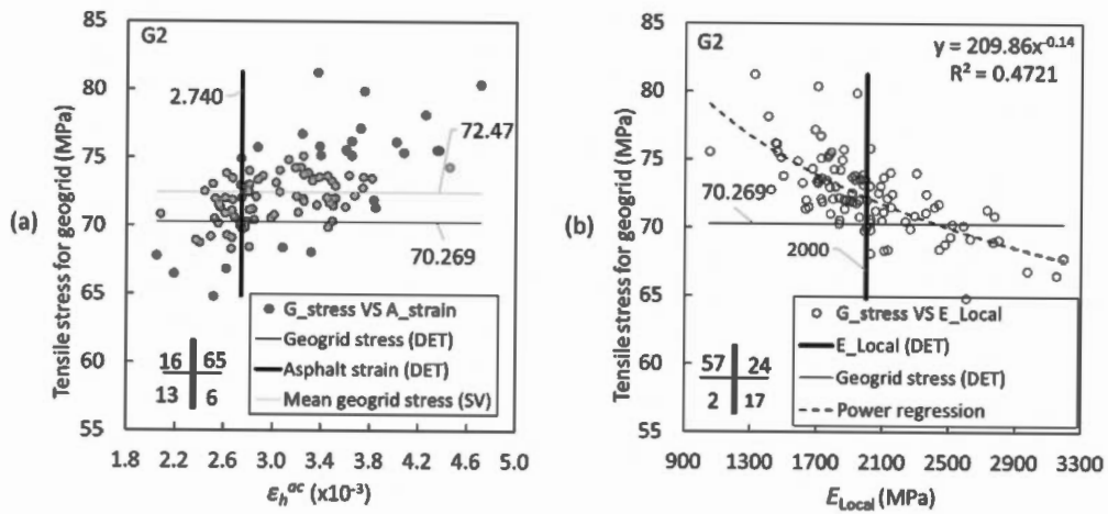
Figure 5. Distribution of the maximum tensile stress of the geogrid (G2): (a) \sigma_h^g versus \epsilon_h^{ac} ; (b) \sigma_h^g versus E_{local} .
