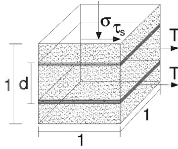
Figure 3. The stabilization and reinforcement effect of the geotextile.
