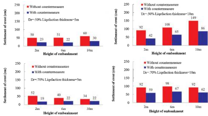
Figure 8. Settlement of embankment crest.
