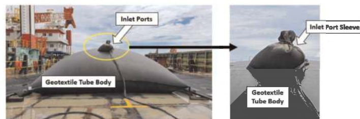
Figure 1. Geotextile tube being infilled on site.
