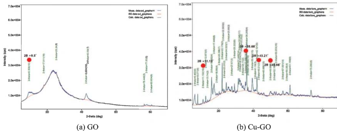
Figure 2. XRD pattern of GO and Cu-GO.
