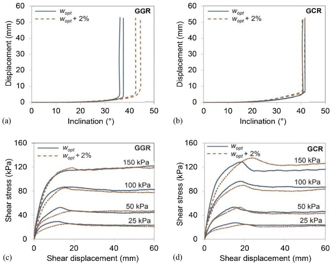
Figure 2. Influence of soil moisture content on soil-geosynthetic interface behaviour: (a) inclined plane tests on soil-GGR interface ( \sigma_v = 10 kPa); (b) inclined plane tests on soil-GCR interface ( \sigma_v = 10 kPa); (c) direct shear tests on soil-GGR interface; (d) direct shear tests on soil-GCR interface.
