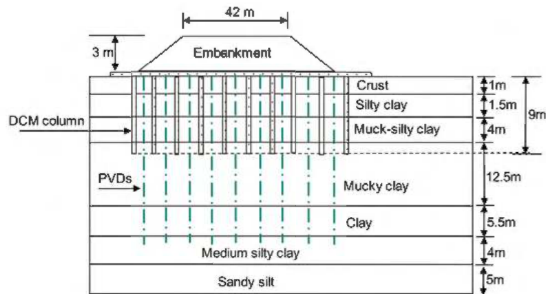
Figure 1. Cross-section of test embankment on composite foundation.
