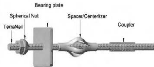
Figure 3. Typical soil nail view.
