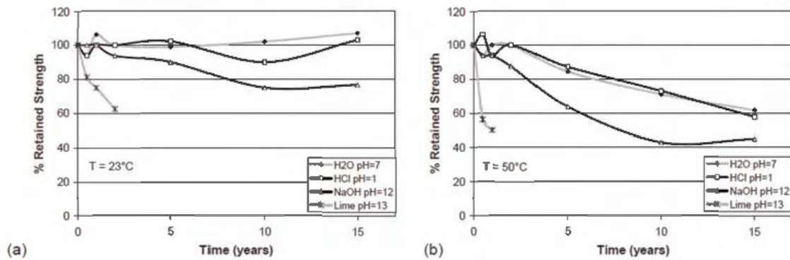
Figure 3. Hydrolytic degradation of PET yarns in various media ( 1 < \text{pH} < 13 ) at (a) 23°C and (b) 50°C over 15 years.
