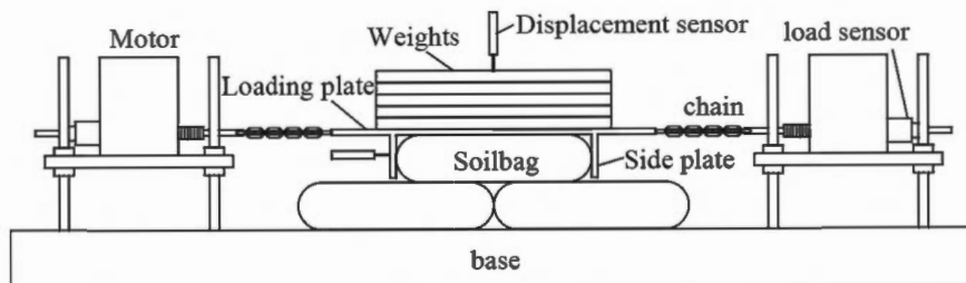
Figure 1. Cyclic shear test device for soilbags.
