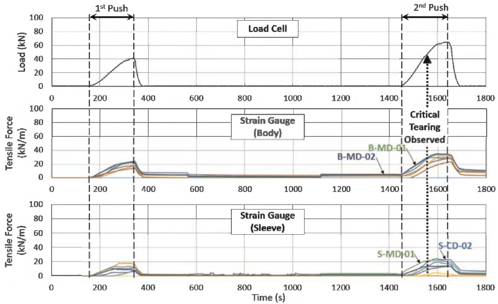
Figure 7. Results of inlet port test T1.
