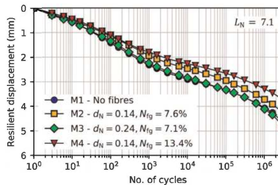
Figure 3. Settlement vs no. of loading cycles.
