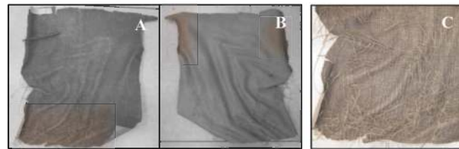
Figure 4. PVC-P geomembrane sample extracted from the north slope crest 258 months after re-waterproofing. A: external face, in contact with the HDPE geomembrane, B: internal face, in contact with the geotextile, C: detail of the state of the external face of the geomembrane.
