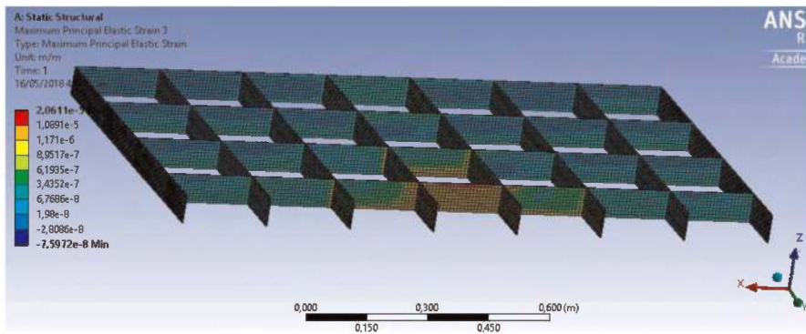
Figure 5. FEA strain in the geocell matrix.
