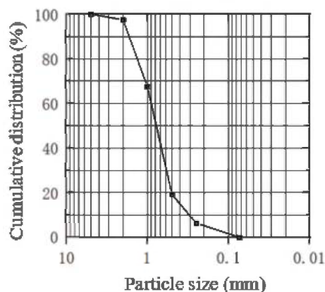
Figure 1. Particle size distribution of test sand.
