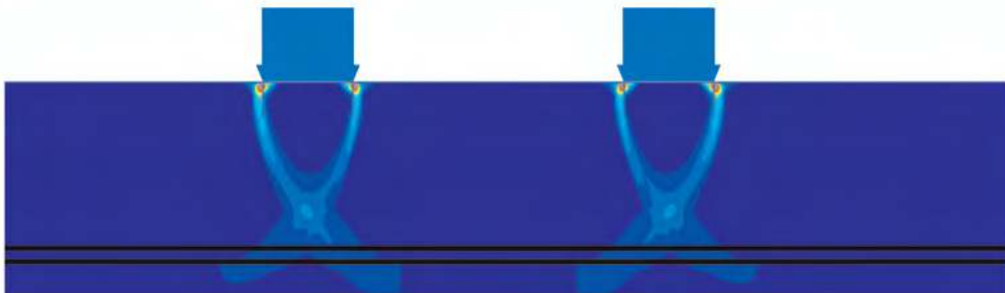
Figure 5. Failure within a thicker working platform with insufficient shear strength ( h_{\text{platform}}=2 m, \varphi_p=27^\circ ).
