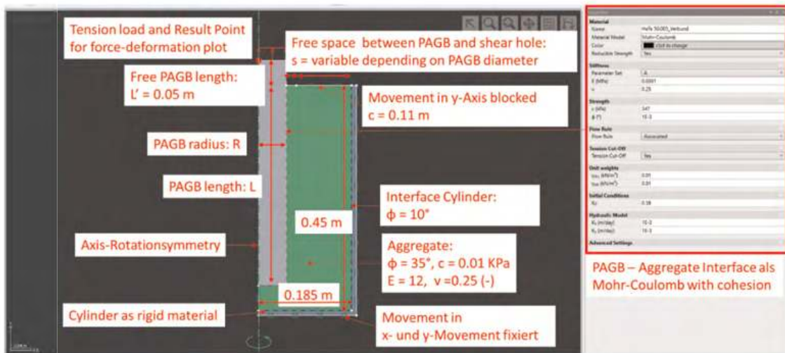
Figure 4. FE model of pull-out test.
