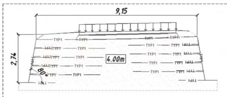
Figure 7. Geometry of reinforced soil.
