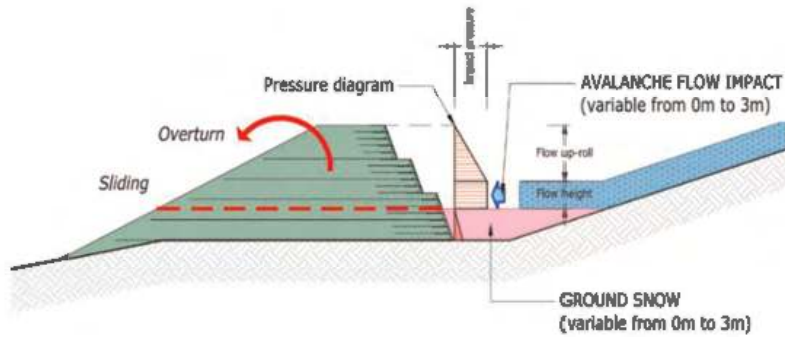
Figure 5. Sliding and overturning analysis schemes.
