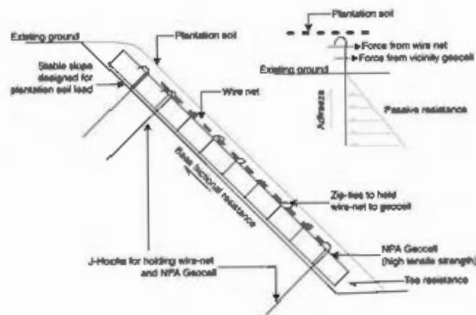
Figure 3a. Schematic section for anchored slope.
