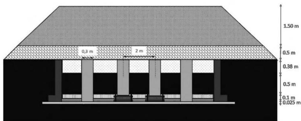
Figure 1. Cross section of the test model.
