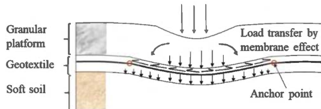
Figure 1. Tensioned membrane effect mechanism involved in reinforced platform by GSY.
