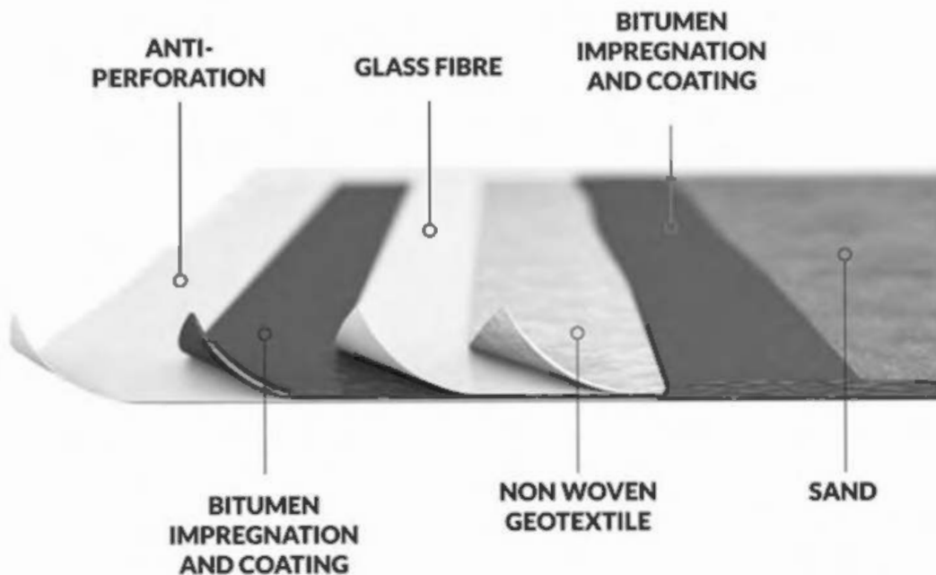
Figure 6. Technical components in the BGM geomembrane.
