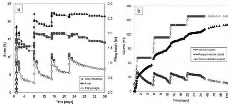
Figure 3. GT1 test. a) circumferential and axial strain during cycles obtained with DWSs and filling height obtained with US. b) volume variation during filling and draining cycles and consolidation period.
