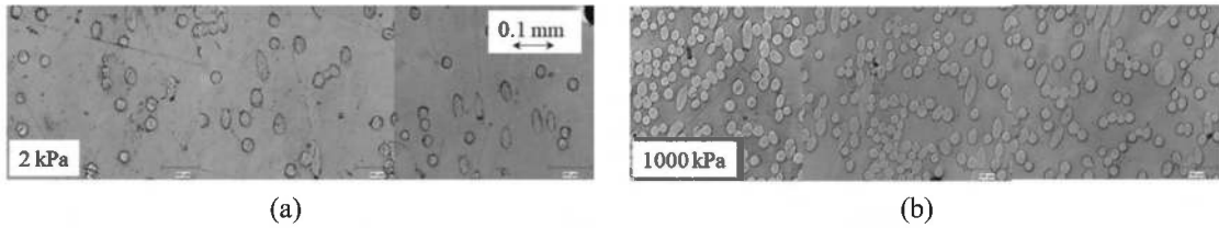
Figure 5. Effect of confining stress on a nonwoven geotextile (Gardoni 2000). (a) 2 kPa, (b) 1000 kPa.
