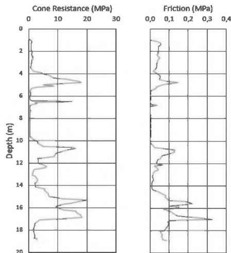
Figure 2. Soil characteristics variation based on CPT measurement.
