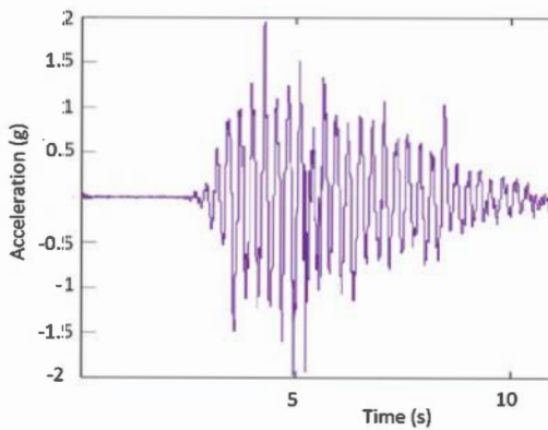
Figure 3. Acceleration applied to the model wall.
