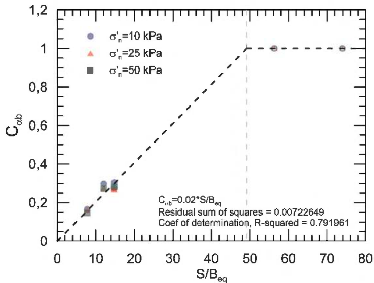
Figure 18. Variation of the reduction factor for the bearing resistance with varying the normalised spacing between transversal members (Cardile et al. 2017a).
