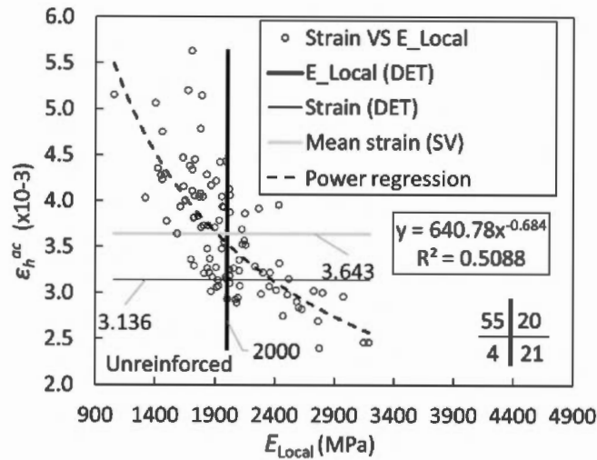
Figure 2. Relationship of E_{local} versus \epsilon_h^{ac} .
