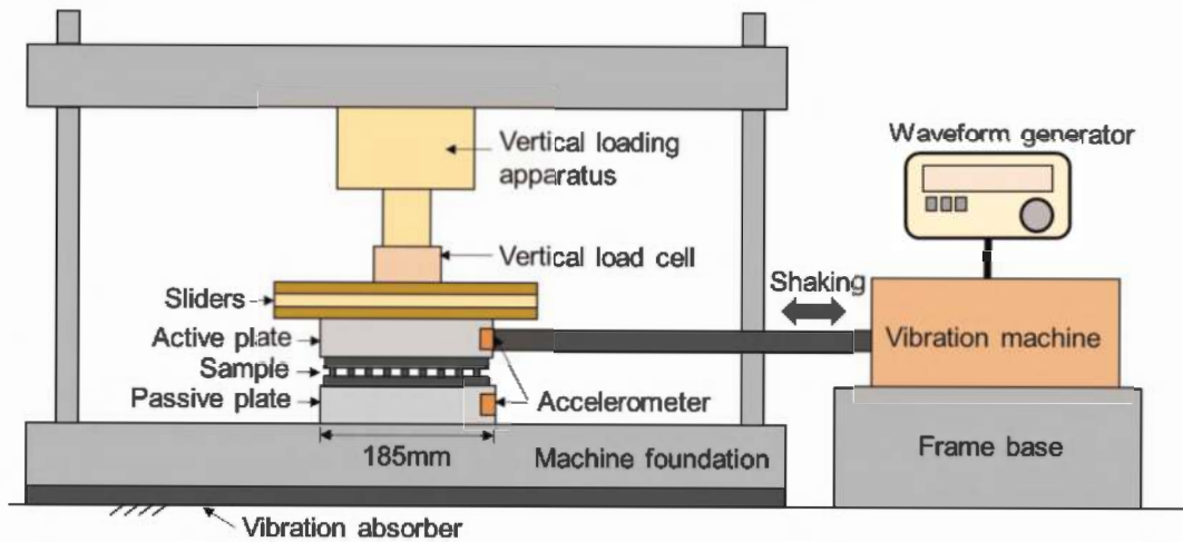
Figure 22. Laboratory model test apparatus to investigate isolation efficiency of geopad geosynthetic samples.
