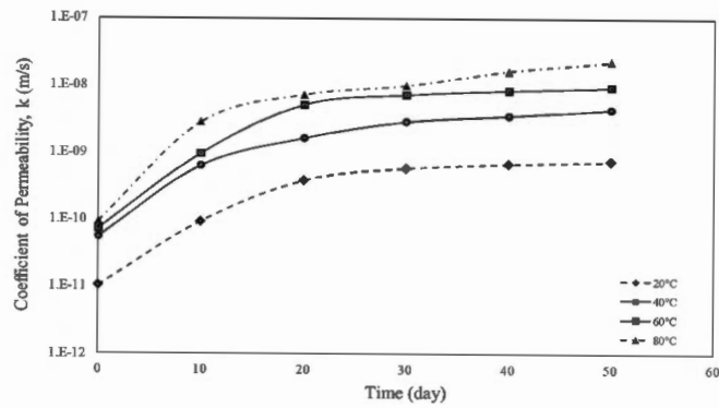
Figure 2. Coefficient of permeability change with respect to time at different temperatures for 2% Na CMC-added GCL.
