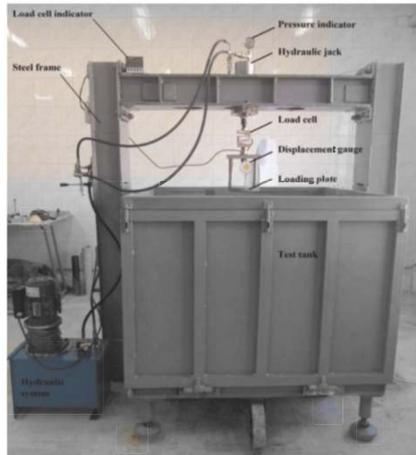
Figure 2. Test tank.
