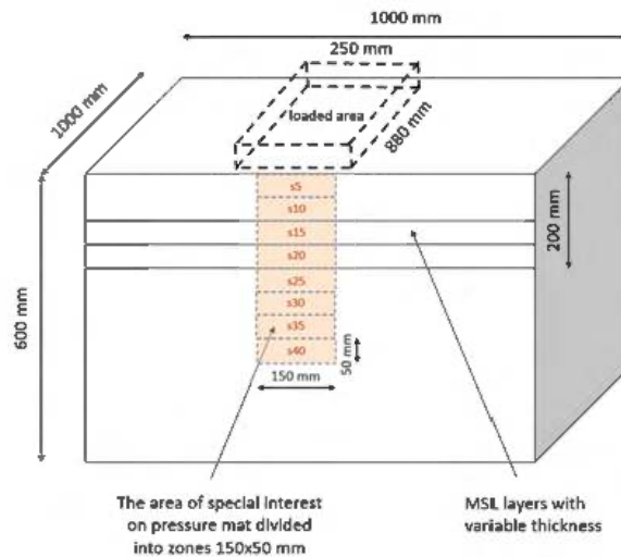
Figure 1. General scheme of the laboratory model.
