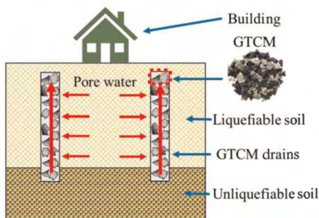
Figure 1. Principle of GTCM drains technique.
