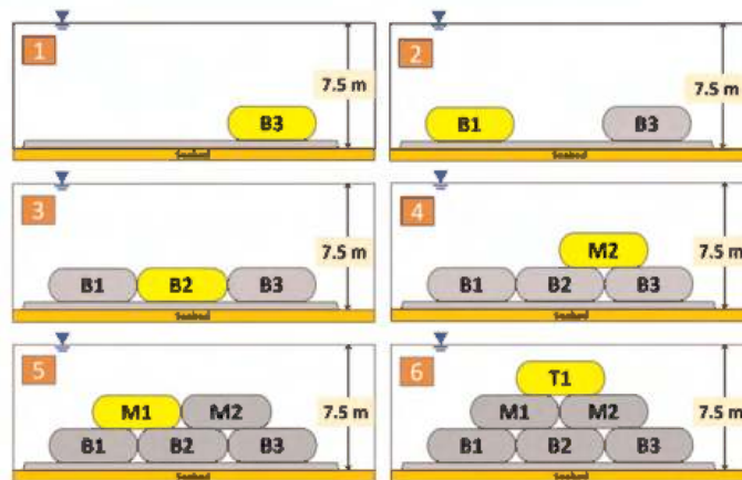
Figure 5. Installation sequence of geotextile tubes.
