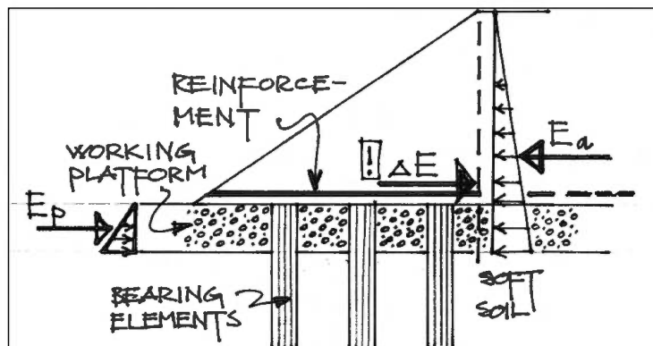
Figure 4. Concept with reduced lateral trust.
