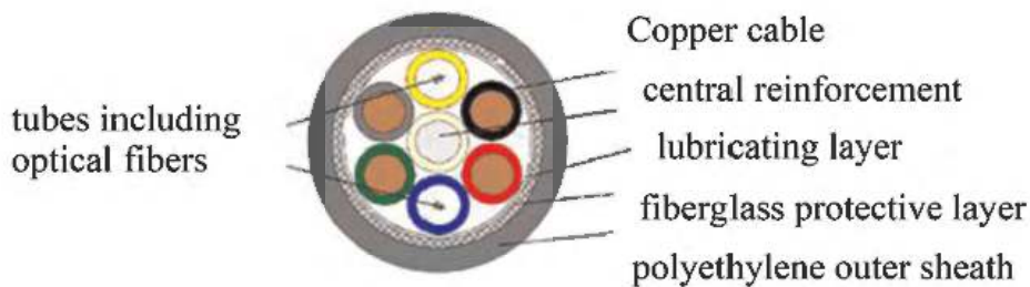
Figure 1. Optical cable used for the active method.
