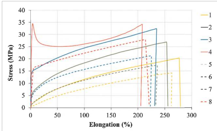
Figure 4. Tensile tests results on the 8 produced geomembranes.
