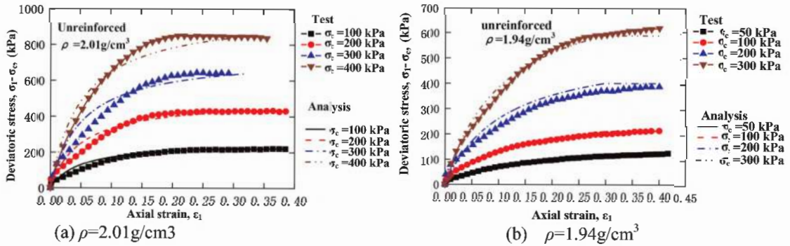
Figure 6. Calibration of calculation parameters of unreinforced soil.
