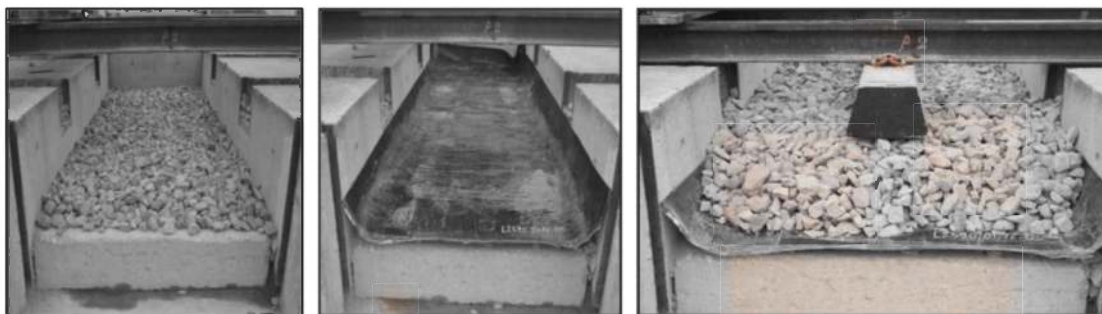
Figure 5. Vibrogyr testing simulating rail traffic on ballast by SNCF (French Railways).
