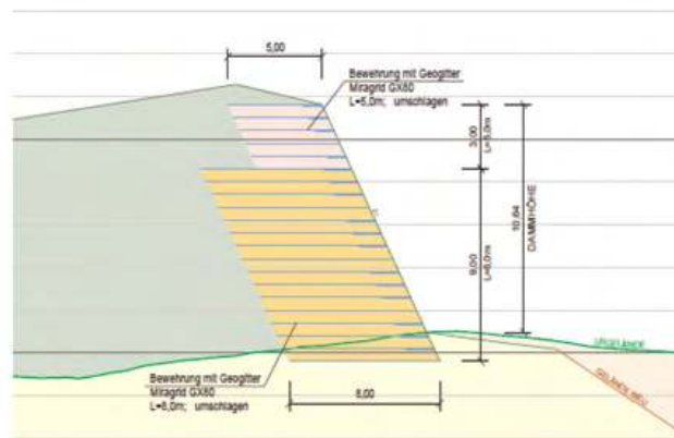
Figure 1. Typical cross section of an avalanche deflecting dam.
