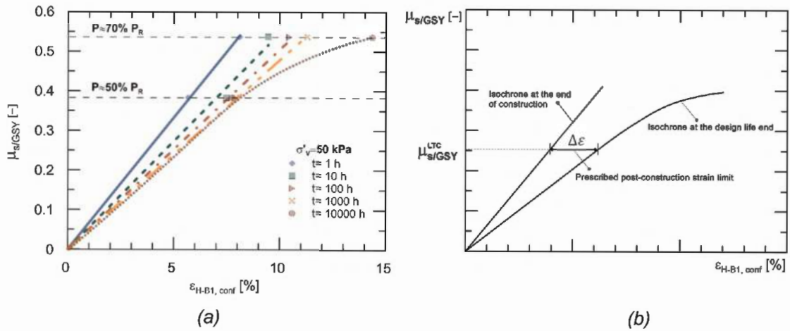
Figure 13. Isochronous interaction curves under long-term pullout conditions. (a) Test results (Cardile et al. 2021); (b) Long-term apparent coefficient of friction assessed at a prescribed limiting value of post-construction strain in reinforcement using isochronous curves.
