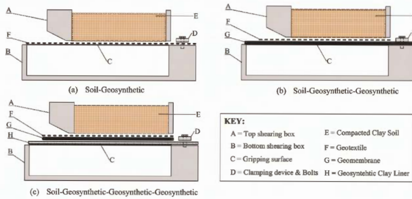
Figure 1. Single and multi-layer interface shear test configurations.
