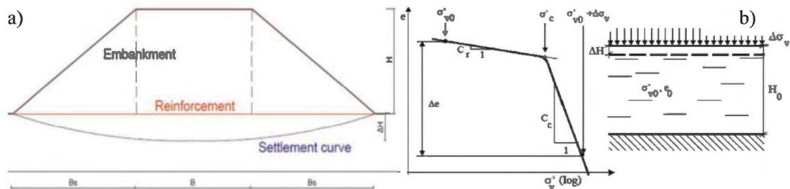
Figure 2. a) The out-of-plane deformation along the settlement curve triggers the tensioned membrane mechanism in geosynthetics for basal reinforcement; b) Scheme for calculating the primary consolidation settlement of a layer of cohesive soil.
