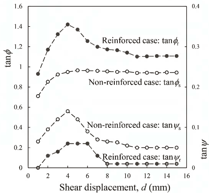
Figure 6. Mobilizations of \tan \phi and \tan \psi .
