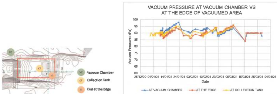
Figure 4. Vacuum pressure during vacuum period.
