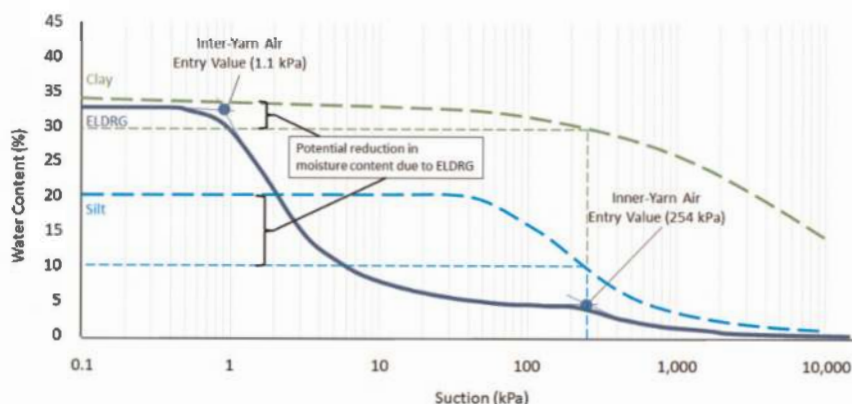
Figure 2. Soil and geotextile water characteristic curves (Lin et al. 2019).
