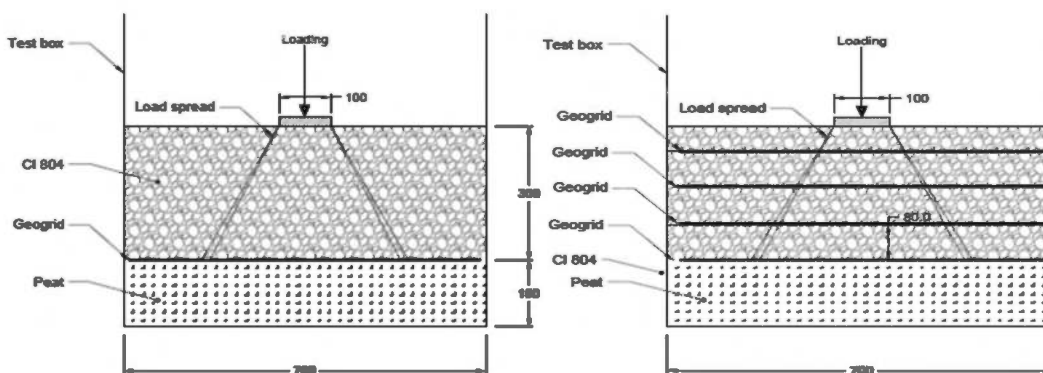
Figure 4. Testing arrangement (Aladwani 2019).
