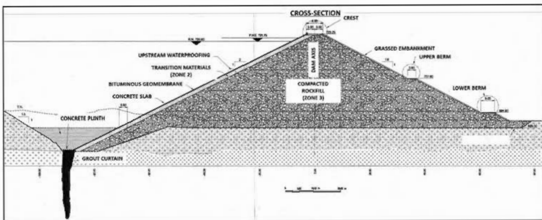
Figure 1. Typical cross-section of La Galaube dam (ISL).
