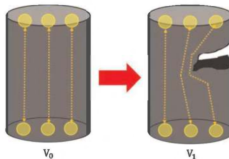
Figure 5. Potential difference due to crack occurrence.
