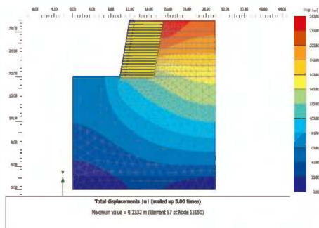
Figure 4. Total displacement.
