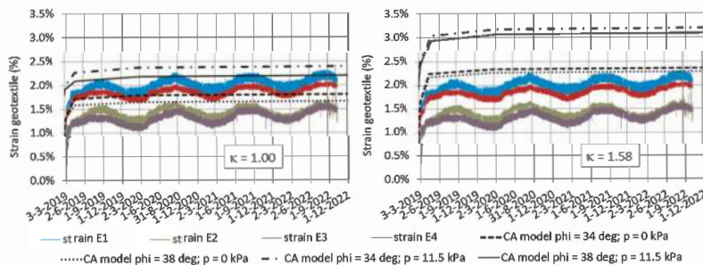
Figure 6. Comparison measured geotextile strains and geotextile strains calculated with the CA model.
