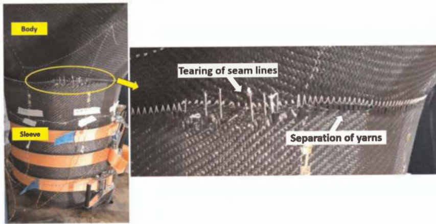
Figure 5. Critical tearing during inlet port loading test.
