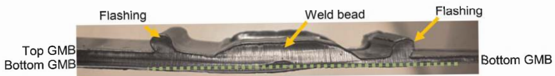
Figure 2. Photographic cross-section view of HDPE extrusion weld.
