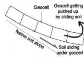
Figure 1c. Sliding failure.
