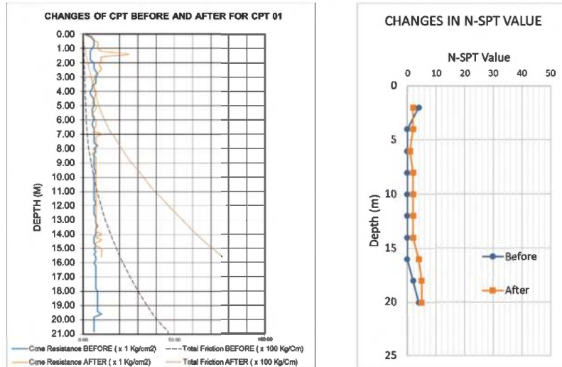
Figure 6. Result of CPT test and SPT test before and after vacuum.
