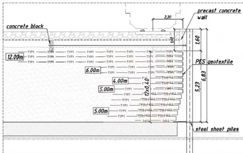
Figure 5. Temporary retaining.
