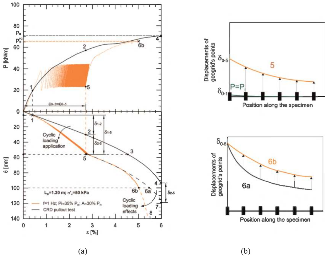
Figure 15. Comparison between P - \varepsilon and \delta - \varepsilon trends obtained in CRD and multistage conditions (a) and qualitative distribution of the geogrid's points displacements in various phases of the test (b) (Cardile et al. 2019).
