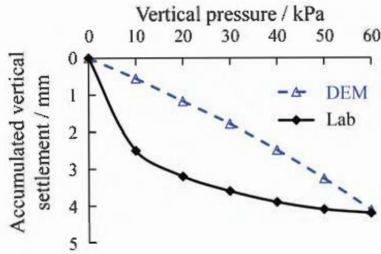
Figure 4. Comparison of vertical pressure and settlement relations.
