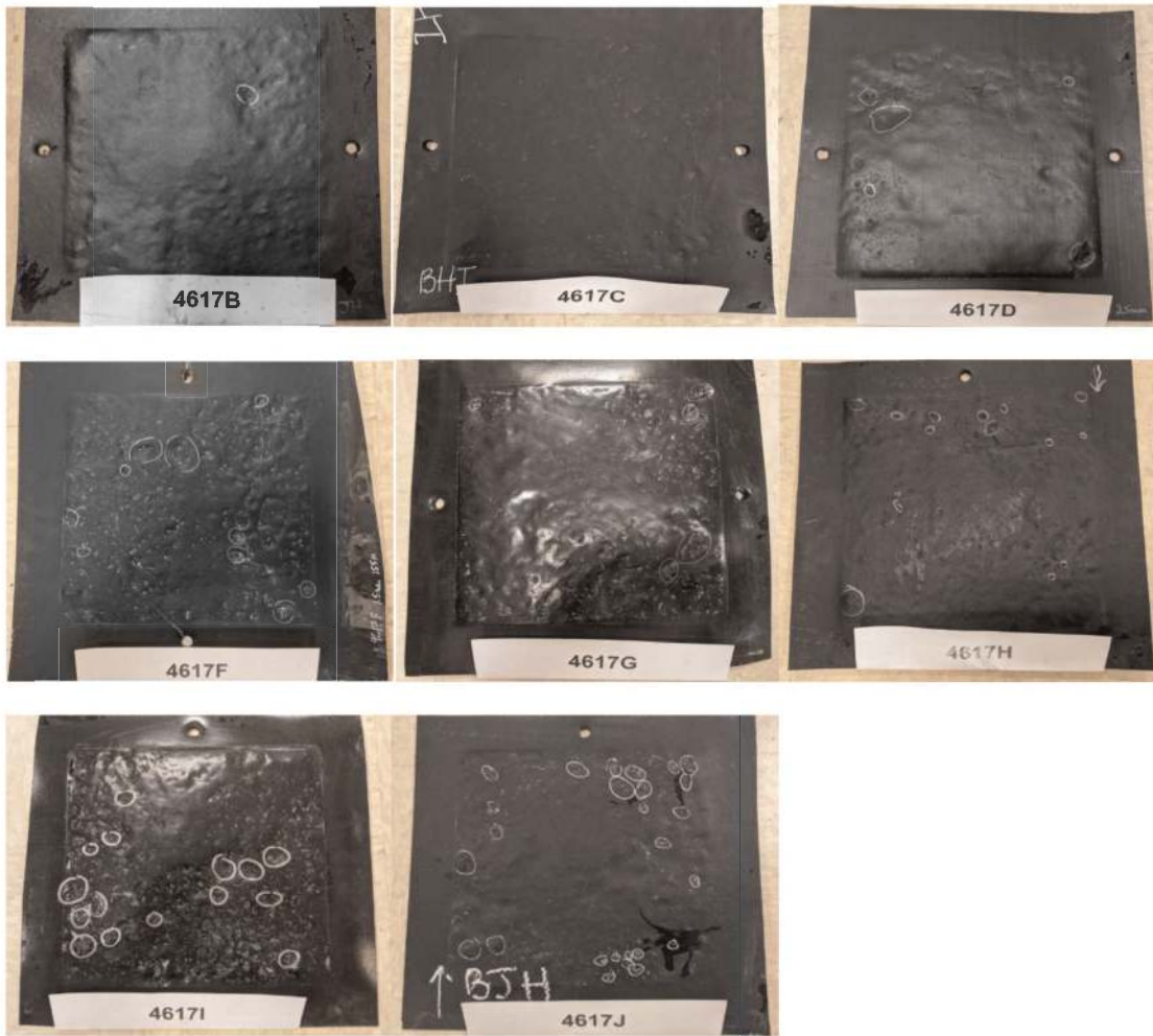
Figure 7. HDPE geomembranes after large scale puncture test.
