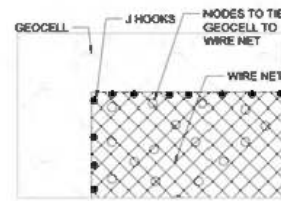
Figure 2b. Wire-net on geocell.
