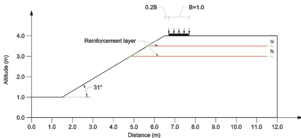
Figure 1. Geometry and dimensions of the problem analysed.
