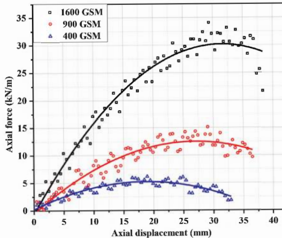
Figure 2. Tensile characteristics of coir geotextiles having different mass density (GSM).
