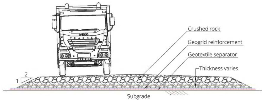
Figure 1. Typical unpaved road cross section.
