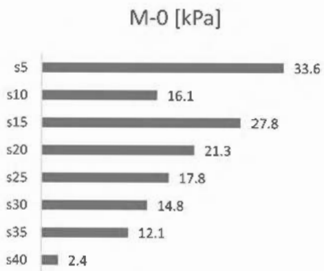
Figure 5. Lateral pressures in model M-0 (kPa).
