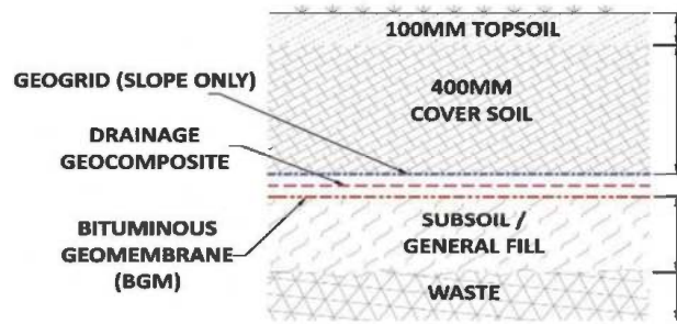
Figure 6. Schematic of industrial waste site cap profile.
