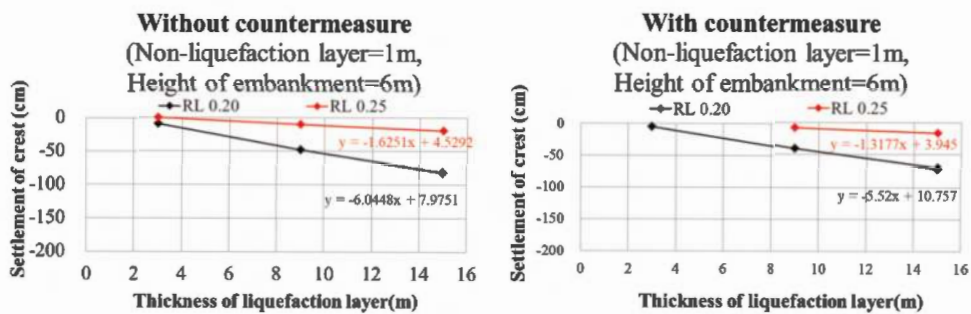
Figure 10. Settlement prediction for level 1 seismic.
