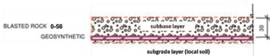
Figure 2. Cross-section of field trial setup.
