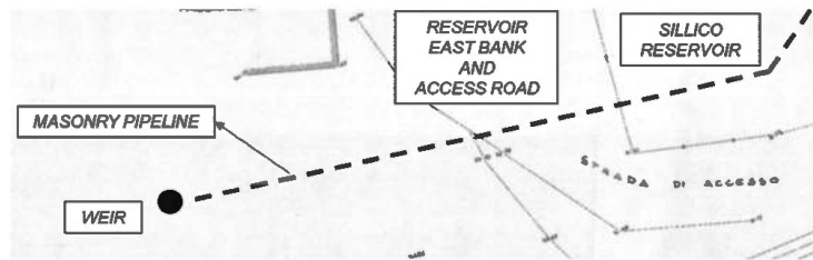
Figure 3. Plan of the drainage system.
