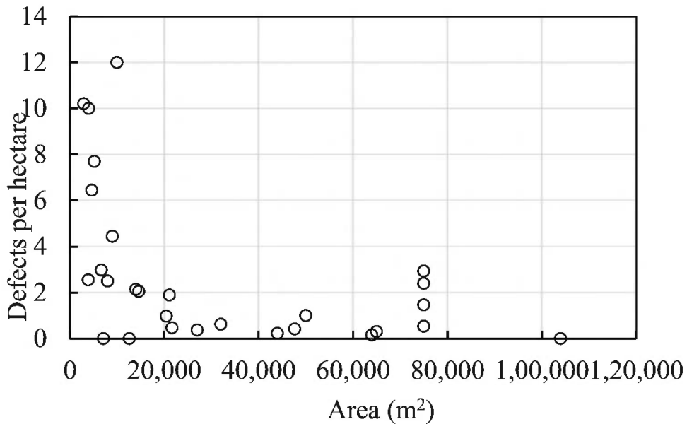
Figure 2. Variation of defect density versus area surveyed.
