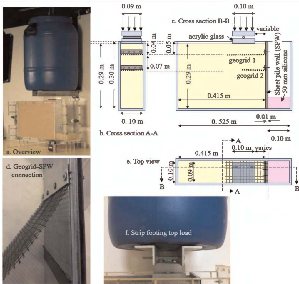
Figure 1. Test set-up.
