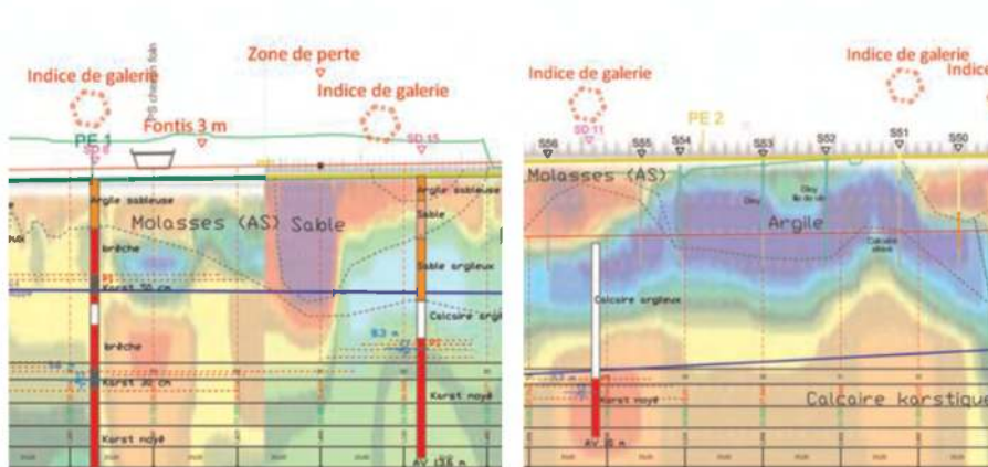
Figure 3. Geotechnical model (samples) – absence of accessible voids is shown.
