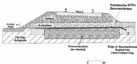
Figure 6a. Designed cross section for BNSF.
