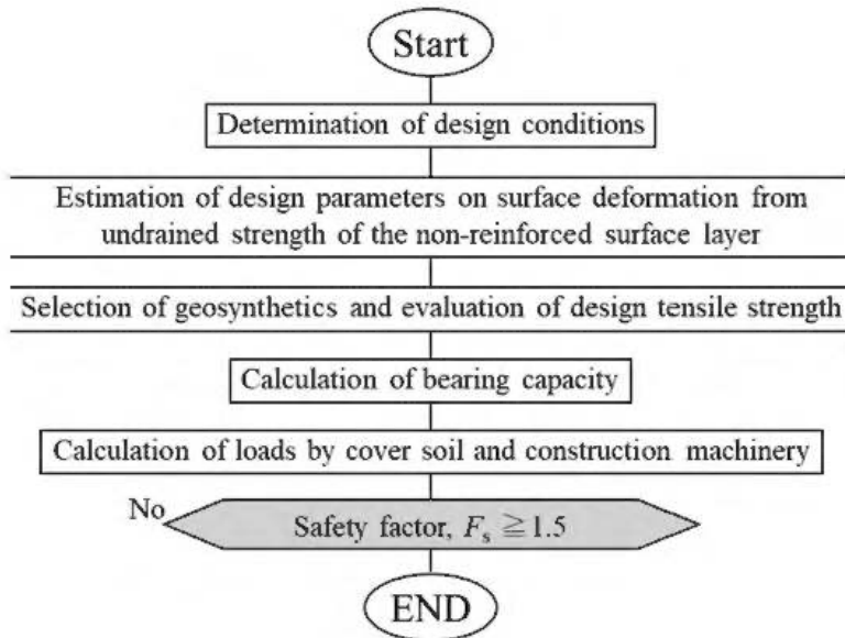
Figure 2. Design flow of geosynthetic reinforcement applied to the surface layer of a super soft soil foundation.
