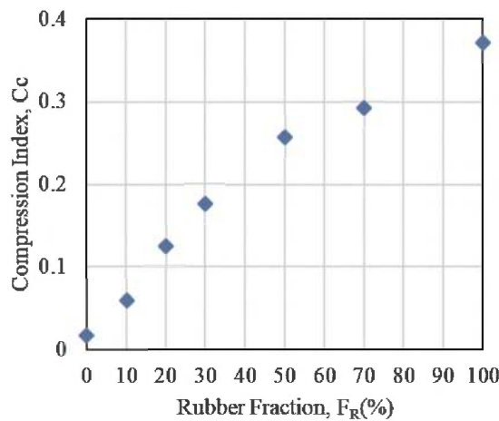
Figure 3. Compression indexes against rubber fraction.
