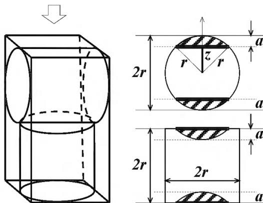
Figure 4. Geometric image of compression (rubber chips).
