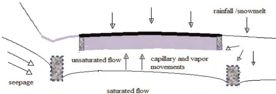
Figure 1. Different ways in which water can act on paving layers.
