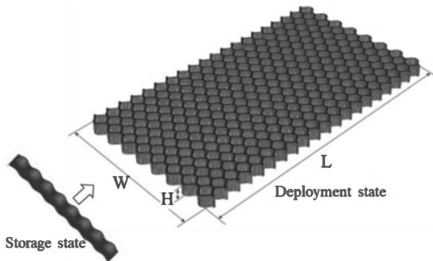
Figure 1. Overview of a geocell.
