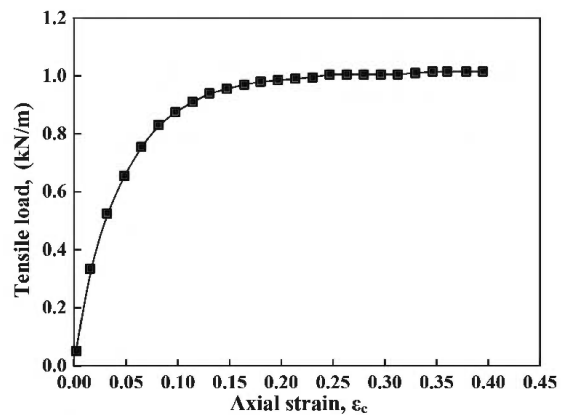
Figure 2. Tensile load-strain curve of geocell sheet.
