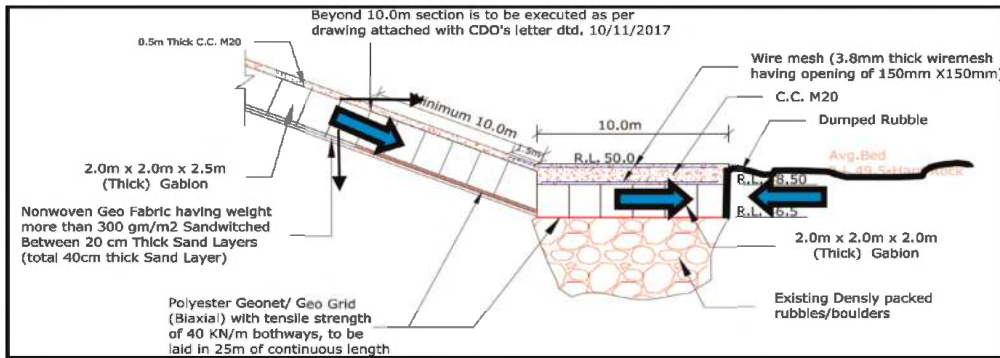
Figure 4. Restoration details - cross section (Kapadia 2022).
