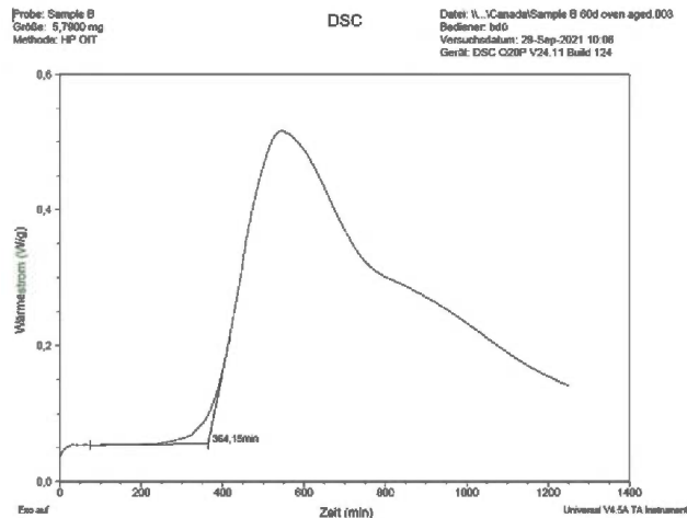
Figure 2. HP-OIT with no shoulder.
