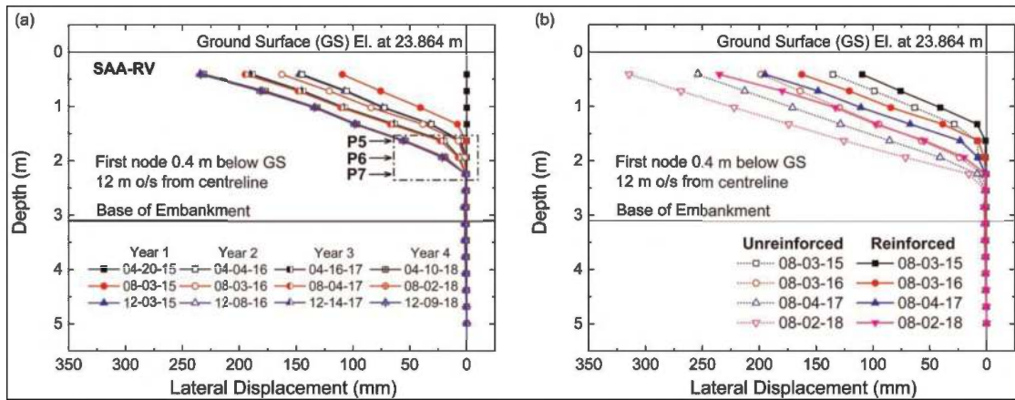
Figure 3. Lateral displacements at (a) different time steps recorded from SAA-RV and (b) comparison with unreinforced test section.
