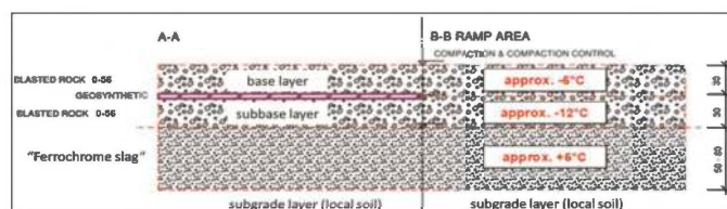
Figure 2. Cross-section of field trial setup.
