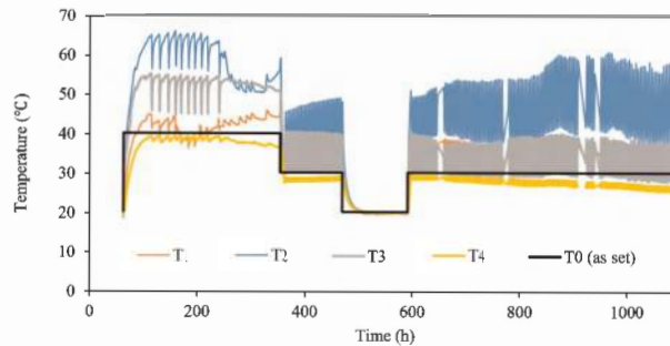
Figure 3. Temperature–time curves at five locations.
