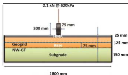
Figure 2. Cross-section of the pavement test section.
