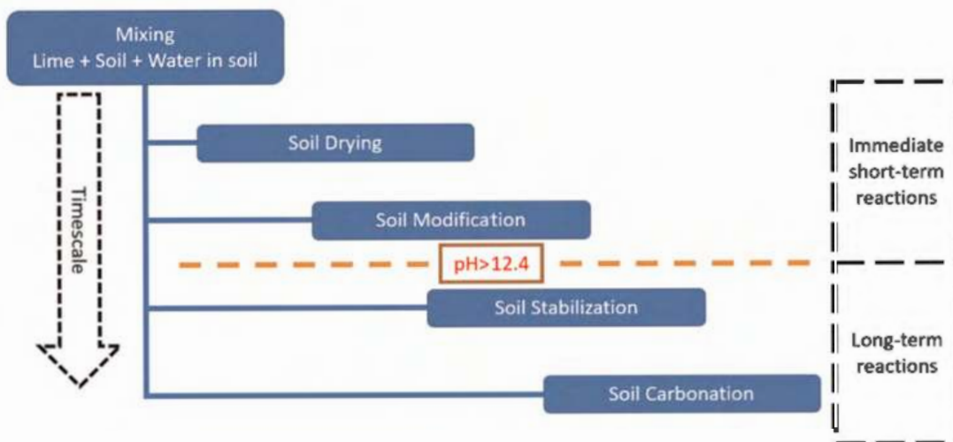
Figure 1. Chronology of lime/soil reactions.
