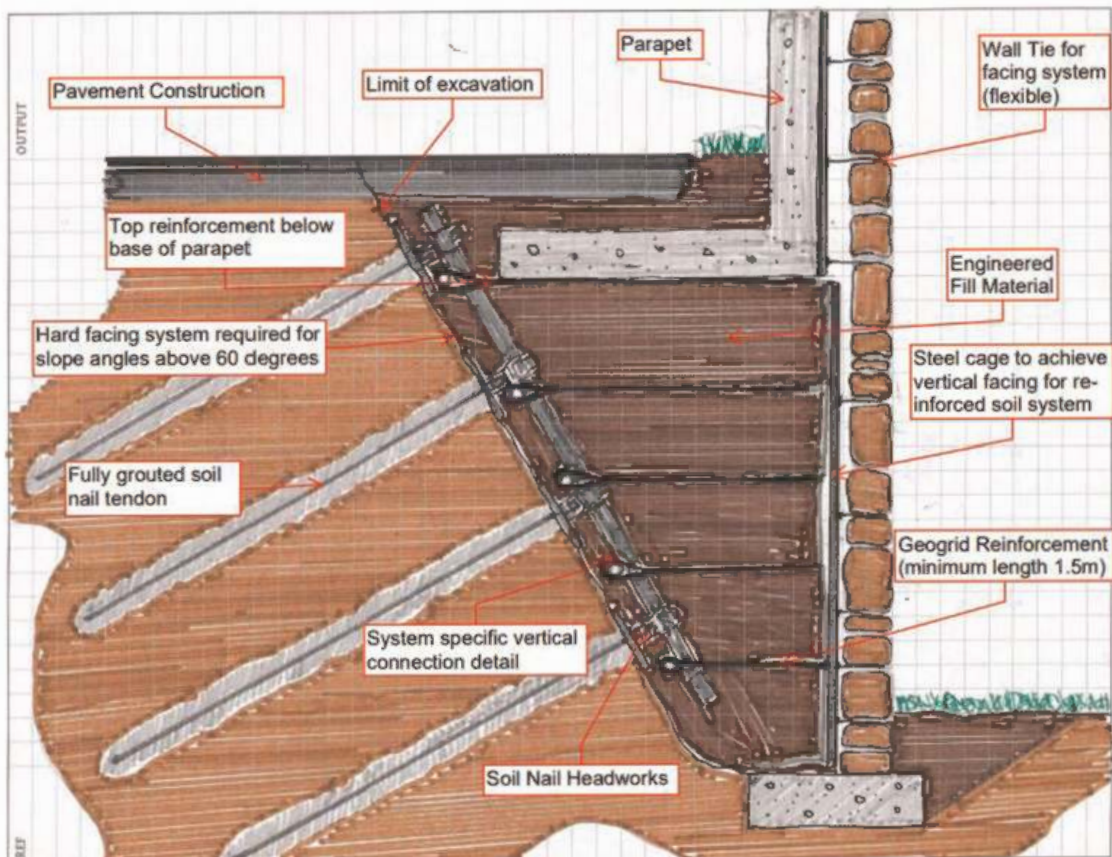
Figure 1. Initial design sketch of hybrid wall concept.
