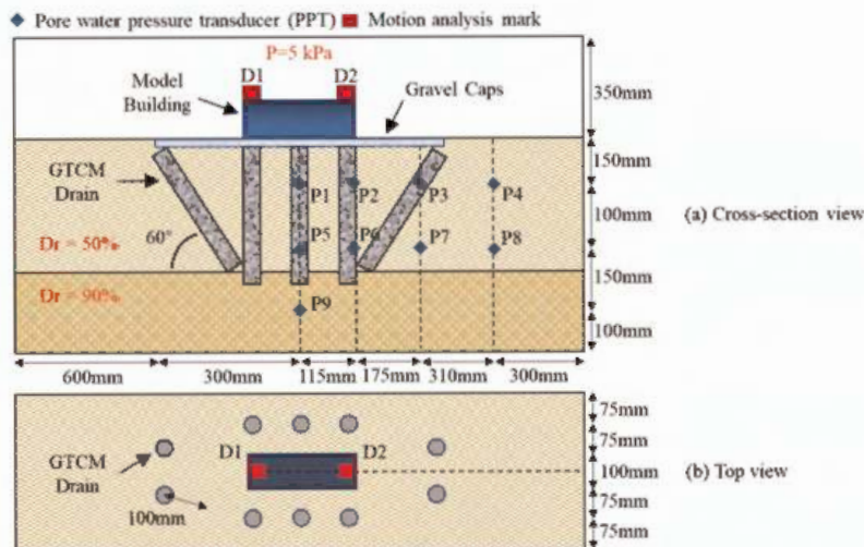
Figure 4. Layout of model test Case 2.
