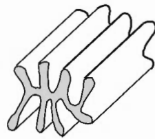
Figure 31. Shape of a wicking geotextile fibre.
