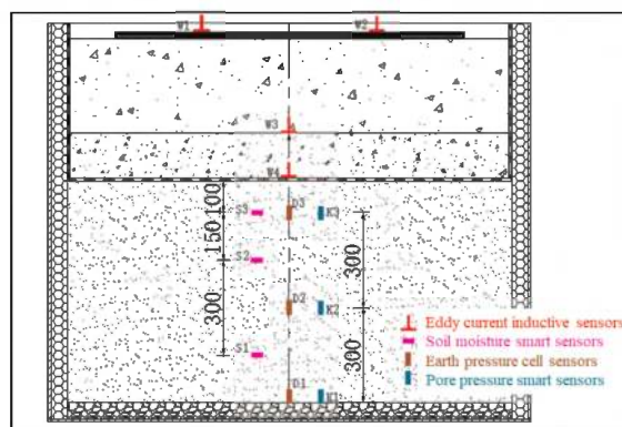
Figure 4. Instrumentations installed in each model.
