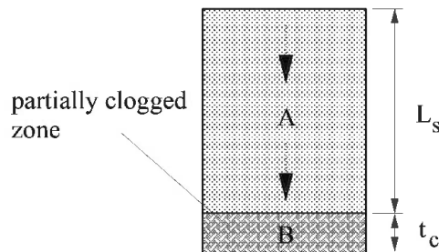
Figure 16. Schematic simplified condition in a filtration test.
