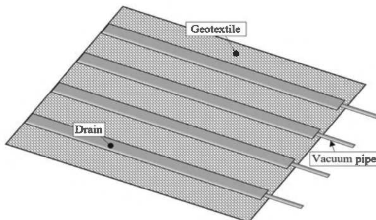
Figure 1. Configuration of horizontal drainage enhanced geotextile sheet.
