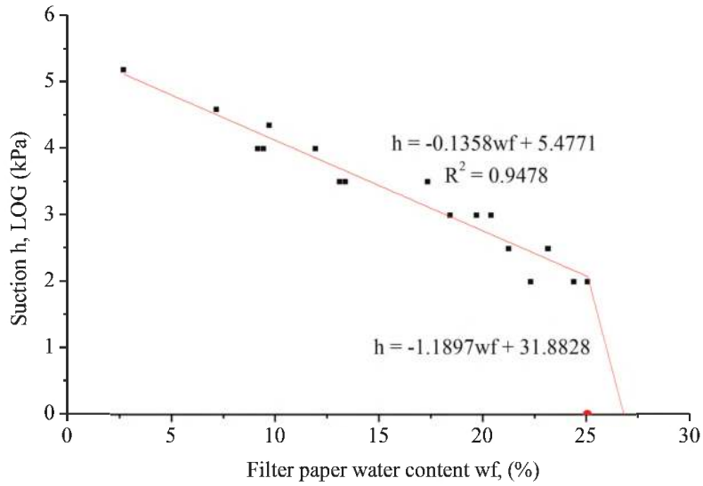
Figure 2. Filter paper lab calibration curve.
