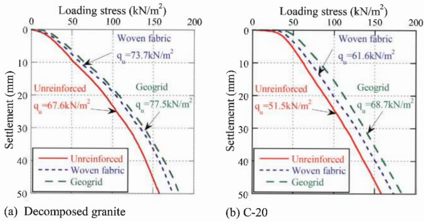
Figure 3. Loading stress and settlement.
