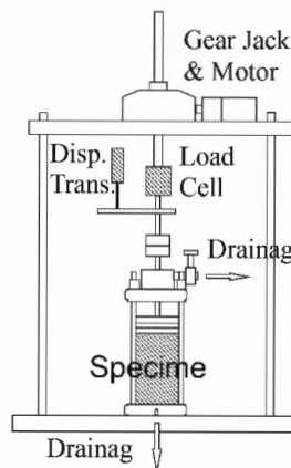
Figure 1. One-dimensional compression test apparatus.
