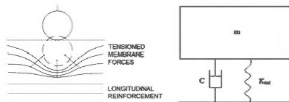
Figure 2. a) Elastic resistance of the longitudinal reinforcements through the tensioned-membrane effect; b) Scheme of the 1-DOF oscillator.
