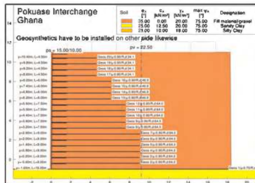
Figure 3. Layout and input parameters for stability analysis in GGU Stability software.
