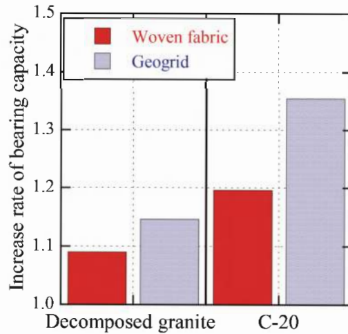
Figure 4. Increase rate of bearing capacity.
