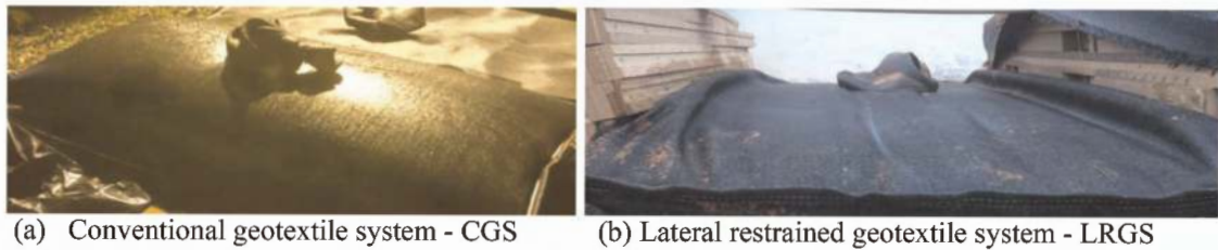
Figure 3. View of the tested bags.
