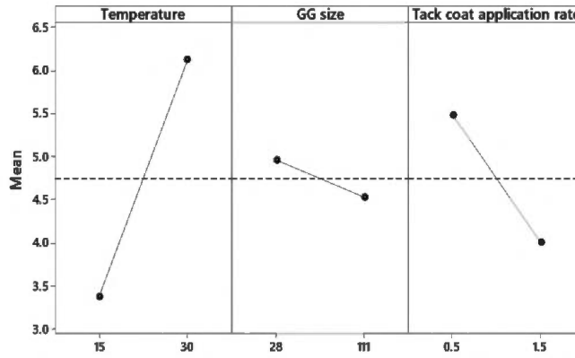
Figure 6. Main effects plot for 600 cycle rutting depth results based on the factors.
