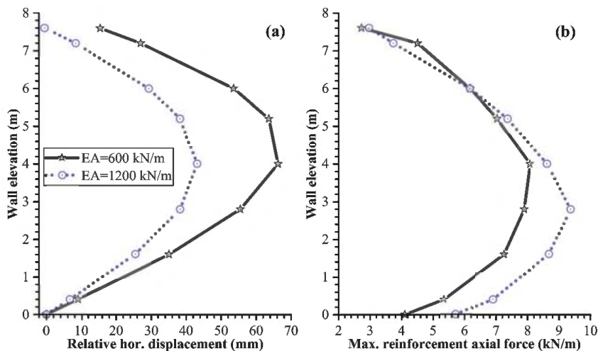
Figure 2. The effect of EA on the wall behavior in the static condition a: (a) relative horizontal displacements and (b) maximum reinforcement axial forces along the wall height.
