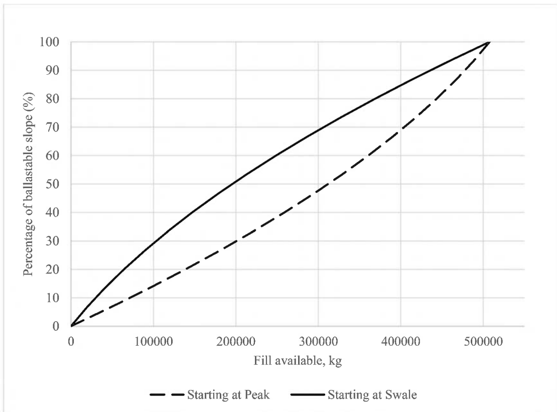
Figure 1. Percentage of ballastable slope vs available fill.
