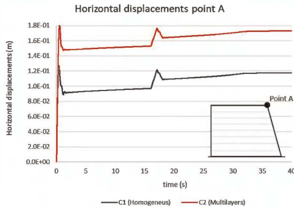
Figure 6. Point A horizontal displacements vs time.
