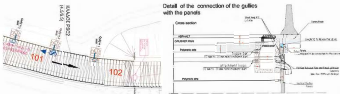
Figure 4. T6A-T6M ramp: (a) Plan view of geostrips layout; (b) detail of connection of gully with panels.
