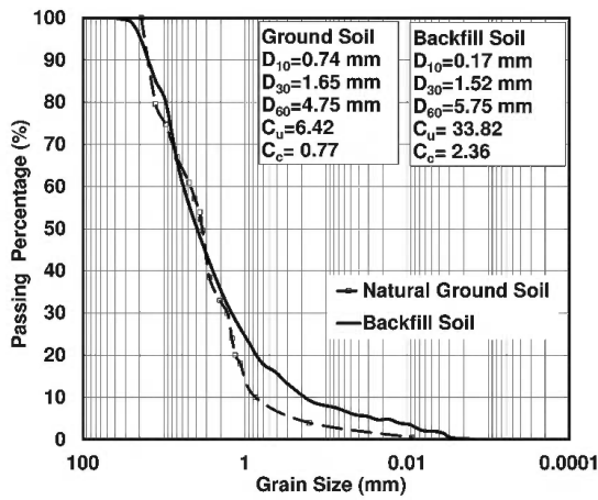
(a) Particle size distribution curves for backfill and natural soils (b) A view of geocell layer spread over soil in the test pit (Moghaddas Tafreshi et al. 2013).
