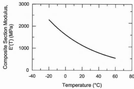
(a) Composite section modulus of soil-geomembrane interface
