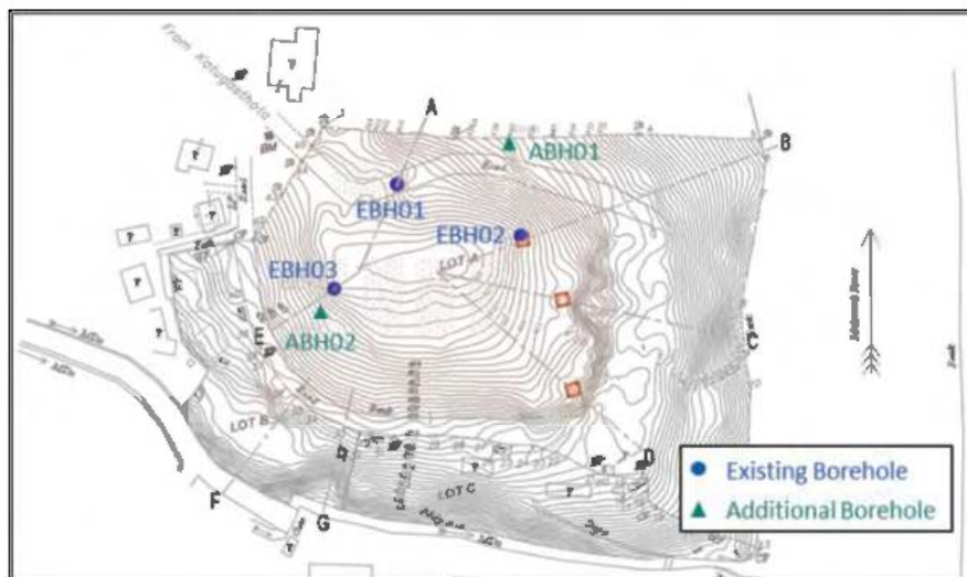
Figure 2. Borehole location and section.
