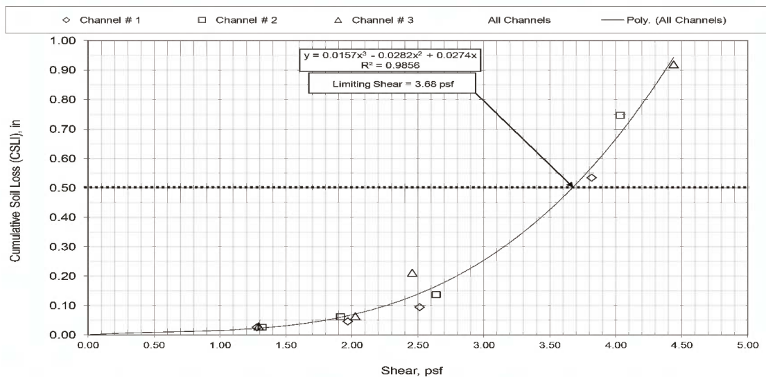
Figure 12. Example large-scale channel erosion testing results.
