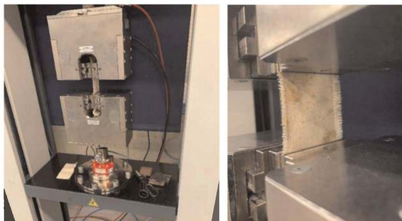
Figure 2. Photos for tensile tests.
