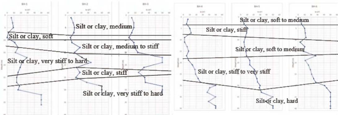
Figure 4. Geotechnical profile for BH-1 until BH-6.
