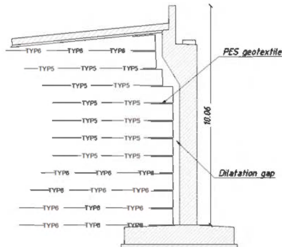
Figure 10. Section of reinforced soil – solution.
