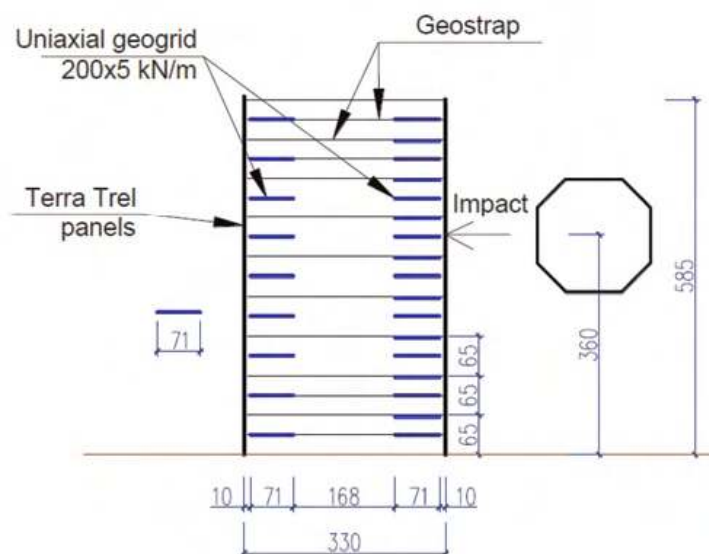
Figure 1. The cross section design of the embankment.
