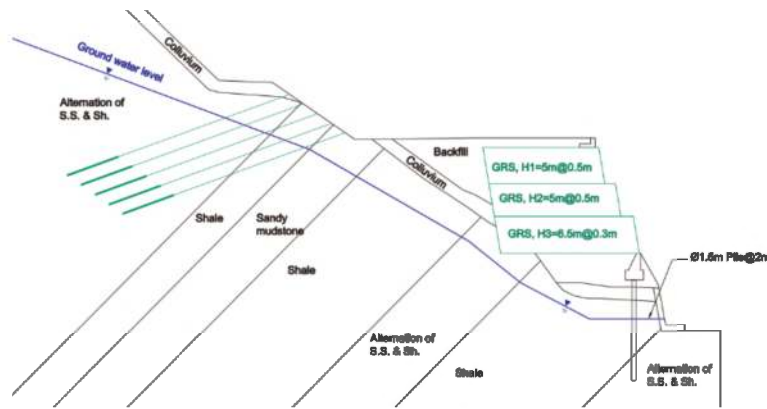
Figure 5 The design scheme of the GRS embankment (Sinotech engineering consultants Ltd. 2017).
