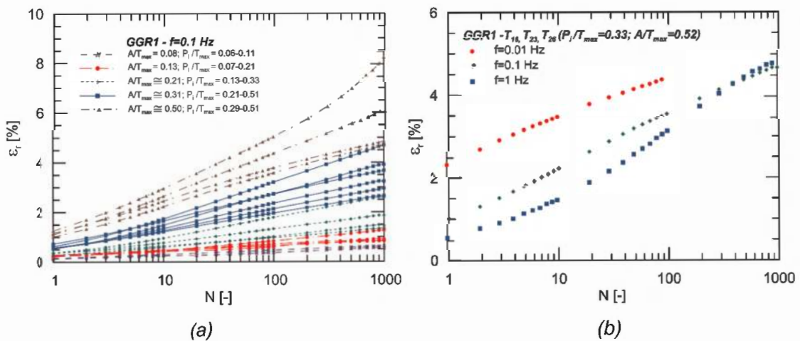
Figure 2. Trends in residual strain with the number of loading cycles for tests conducted at a frequency of 0.1 Hz (a) and tests with P_i/T_{max} equal to 0.33 and A/T_{max} equal to 0.52 at various frequencies (b) (Cardile et al. 2017b).
