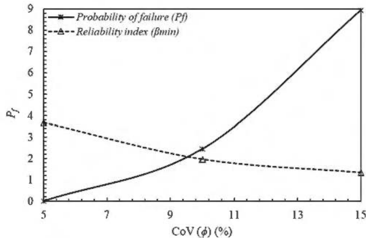
Figure 2. Plot of P_f against CoV ( \phi ).
