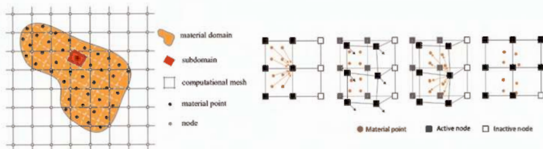
Figure 2. Concept of MPM computation.
