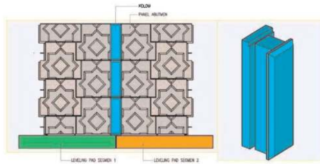
Figure 6. Dilated column detail.
