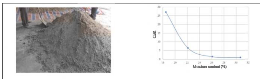
Figure 5. Subgrade soil and its calibrated CBR vs. moisture content curve.
