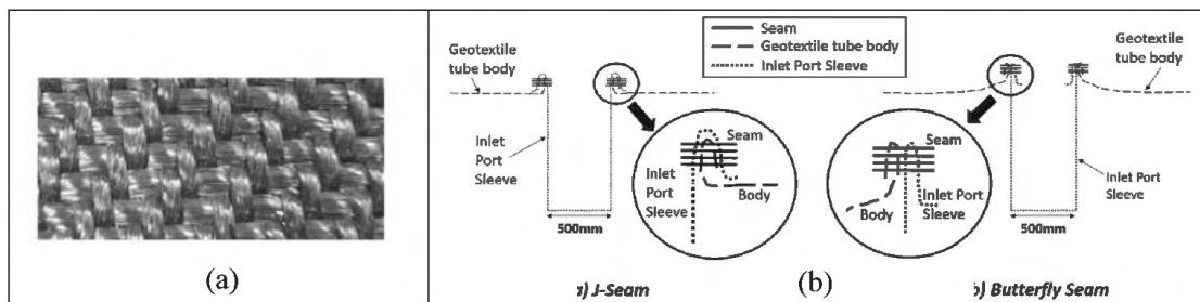
Figure 3. (a) Geotextile material; and (b) Seam designs.
