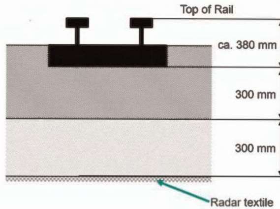
Figure 12. Section indicating RDG in track ballast renewal.
