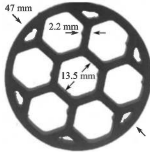
Figure 2. Honeycomb inclusion used for reinforcement.
