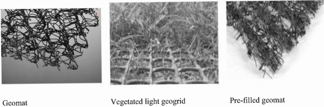
Figure 3. Examples of three-dimensional planar products provide surface erosion control (from ISO TR 128228-8).
