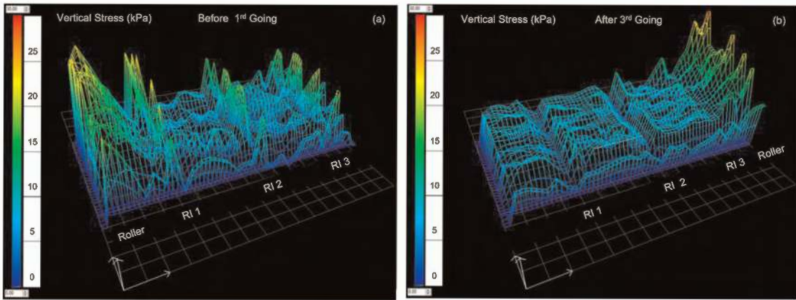
Figure 8. Vertical stress above the analog soft soil and the 3 RIs: a) before 1 st going; b) after 3 rd going.
