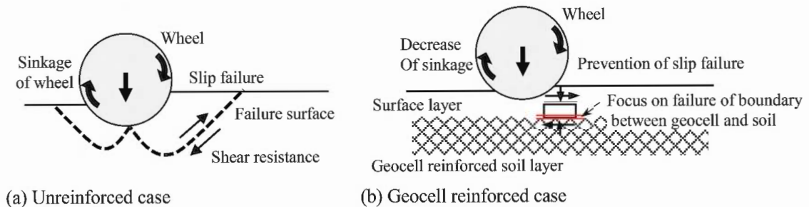
Figure 2. Effects of geocell reinforcement.
