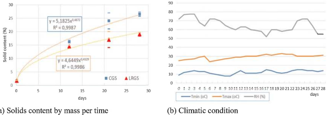
Figure 5. Solid contents and climatic condition during dewatering.
