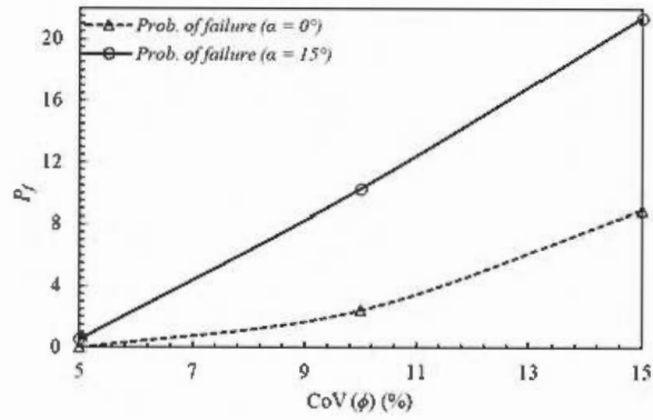
Figure 3. Plot of P_f against \text{CoV}(\phi) for different \alpha .
