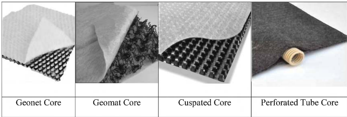
Figure 1. Examples of drainage cores (from ISOTS18198-08).
