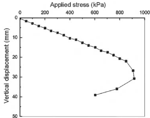
Figure 2. Applied load versus vertical displacement.
