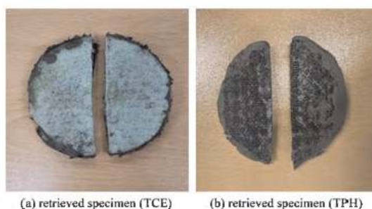
Figure 5. Retrieved Test specimens of geosynthetic oil absorbent liner.
