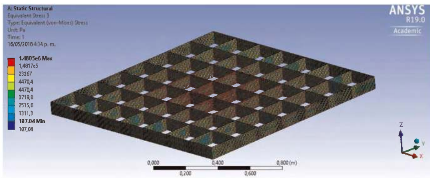
Figure 4. Stress in geocell matrix.
