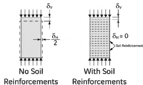
Figure 1. Effect of reinforcement on soil deformation.
