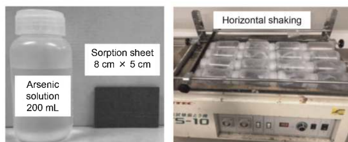
Figure 3. Set up of the batch sorption tests.
