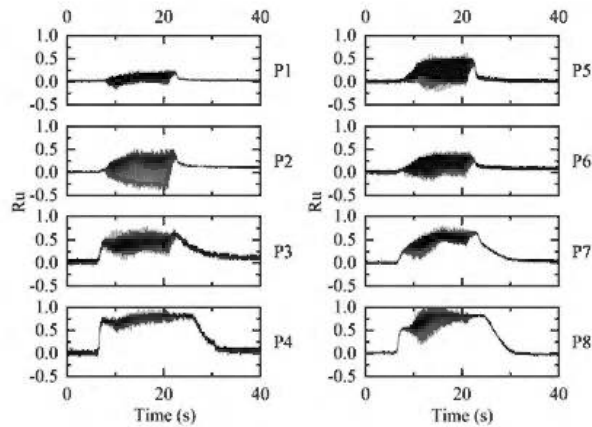
Figure 7. Time history of R_u in Case 2.
