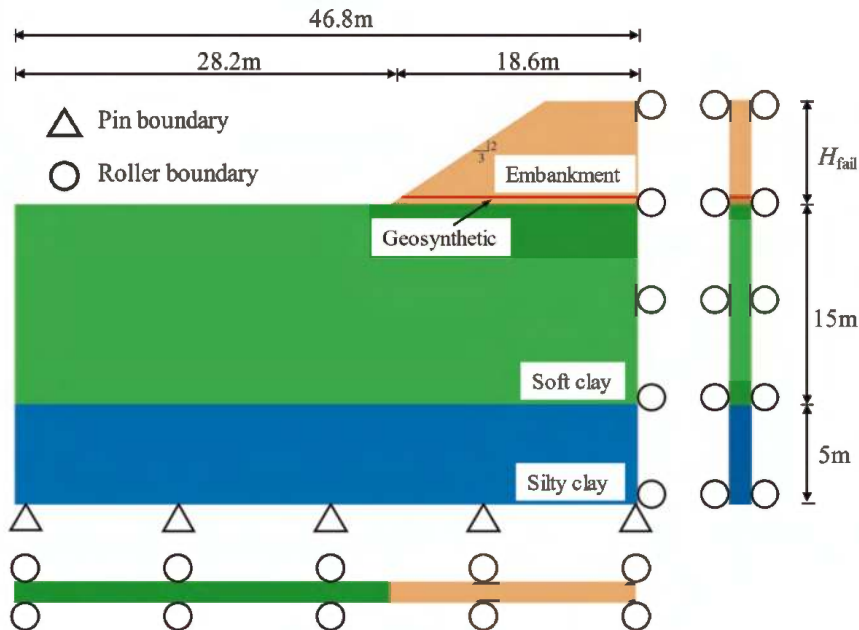
Figure 1. The configuration of the numerical model.
