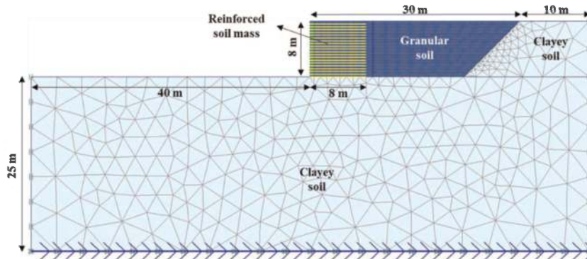
Figure 1. MSE wall model.
