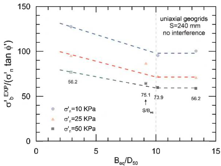
Figure 17. Scale effect: results of pullout tests in terms of \sigma'_b/(\sigma'_n \tan \phi') ratio, carried out on different soils using uniaxial geogrids in which interference effect is negligible (Cardile et al. 2017a).
