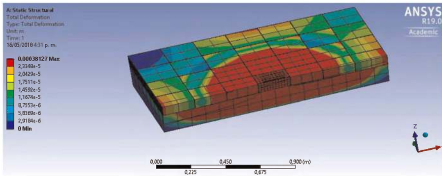
Figure 3. FEA total deformation.
