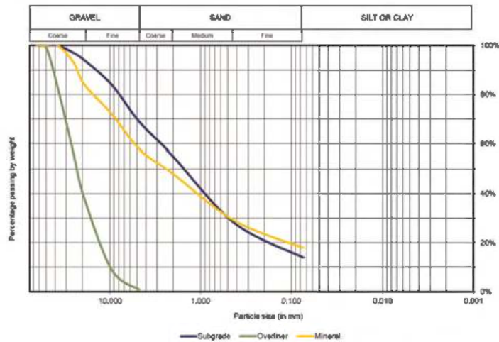
Figure 2. Size consists of granular materials.
