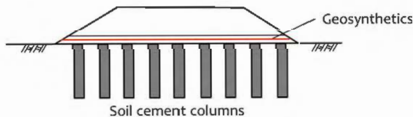
Figure 10. Geosynthetic basal reinforcement combined with deep mixing.
