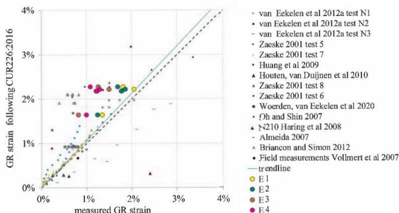
Figure 7. Extension of the validation of the CA model with the new data, with in the calculations: \varphi = 38^\circ , traffic load = 0 kPa and \kappa = 1.58 .
