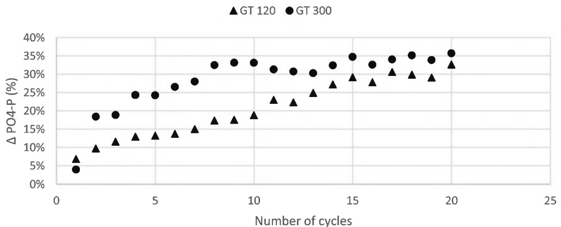
Figure 3. Variation of \text{PO}_4\text{-P} removal in permeameters.
