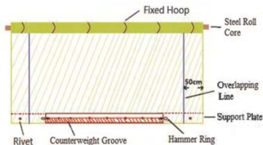
Figure 2. Schematic diagram of GCL composite component.
