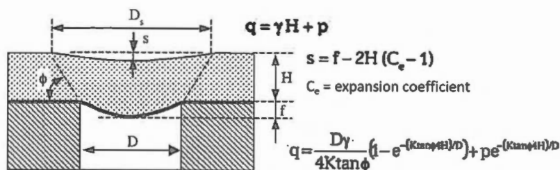
Figure 10. Geosynthetics for reinforcement karst reinforcement – Rafael method.
