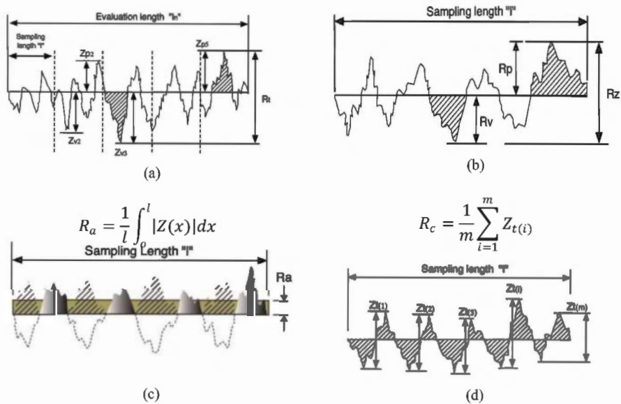
Figure 1. Investigated bidimensional roughness parameters: (a) R_t , (b) R_z , (c) R_a and (d) R_c .
