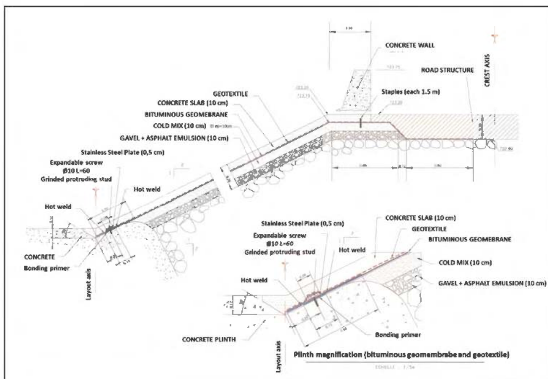
Figure 2. Typical cross-section of the upstream facing.
