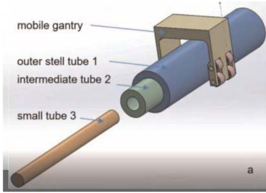
Figure 4. Drawings of roller design.
