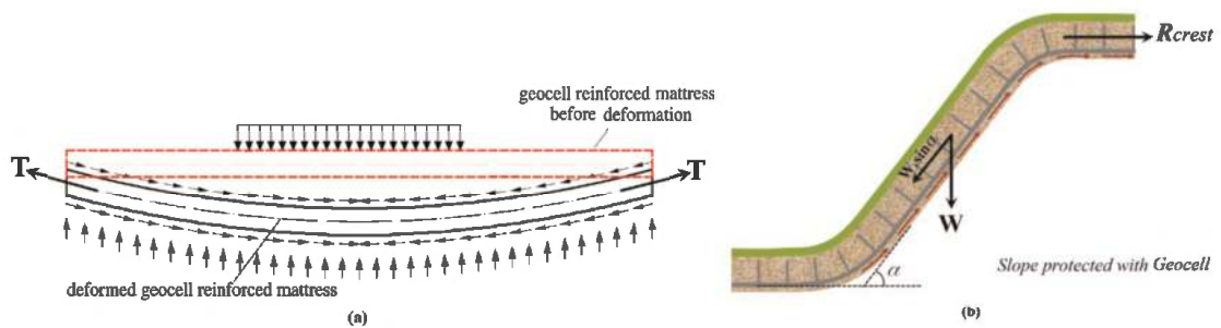
Figure 1. Example applications of geocells subjected to planar tensile forces: (a) Planar tensile forces (T) in a geocell (Zhang et al 2012), (b) a Slope protected by geocell subjected to downward tensile.
