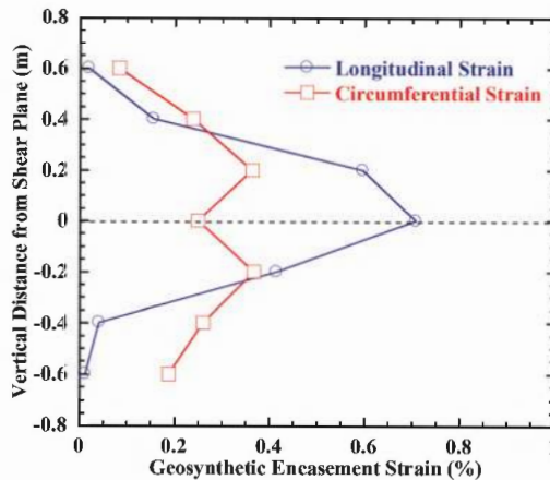
Figure 5. Geosynthetic encasement strain profiles.
