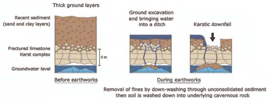
Figure 2. Kinematics of the karst collapse (2021-02-09).
