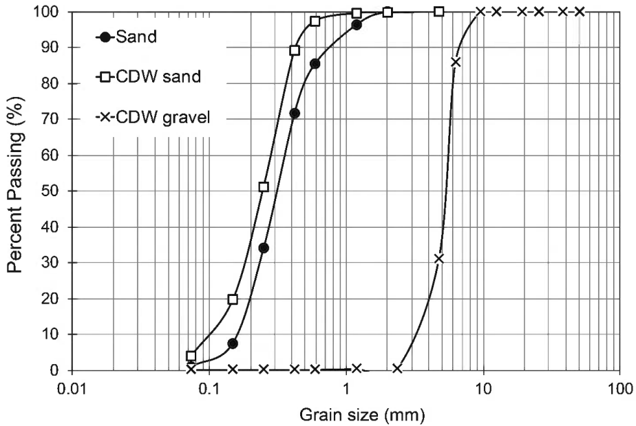
Figure 1. Particle size distribution curves.
