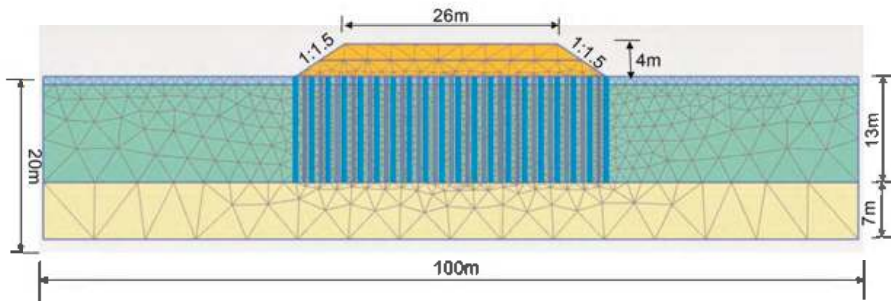
Figure 3. Geometry and mesh properties in numerical analysis.
