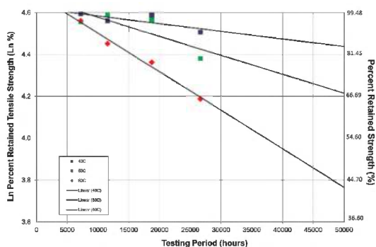
Figure 1. Average tensile strength retained for Geogrid A in pH 11.4.
