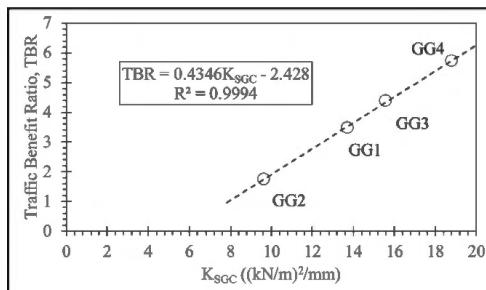
Figure 8. Traffic Benefit Ratio Vs. K_{SGC} .
