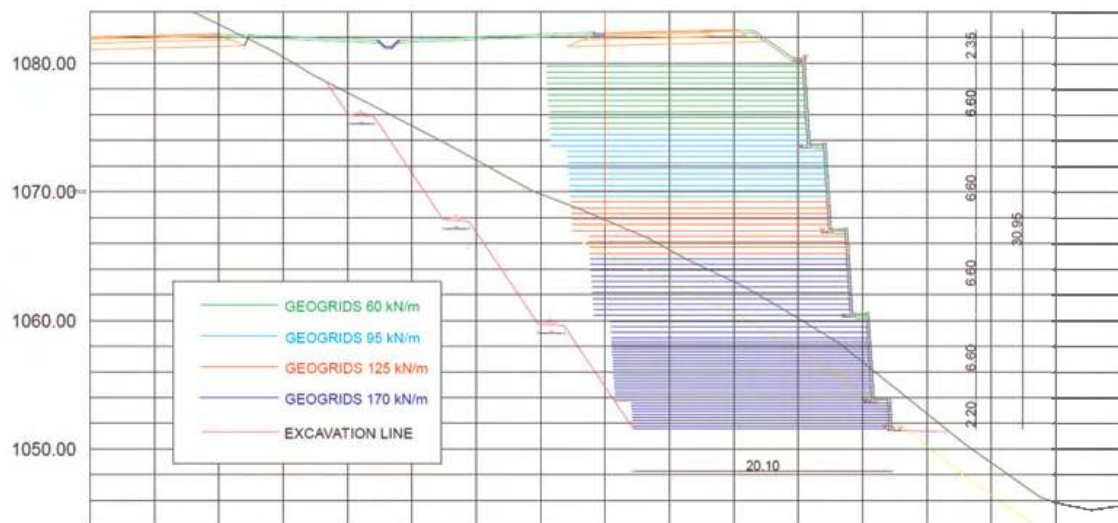
Figure 5. Cross-section of one of the tallest walls.
