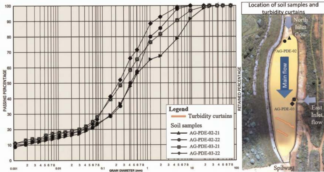
Figure 2. Grain size distribution curves of the soils.
