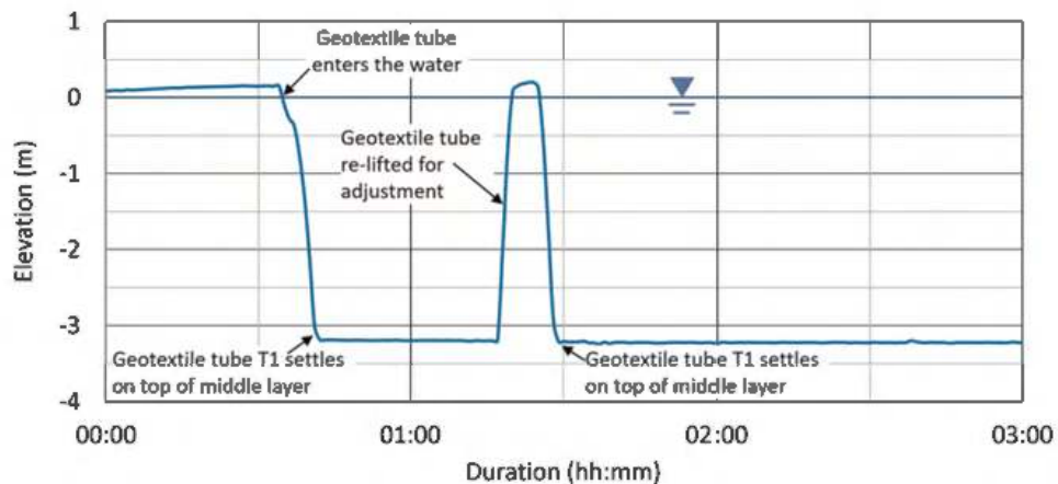
Figure 10. Movement of tube T1 during the lowering process.
