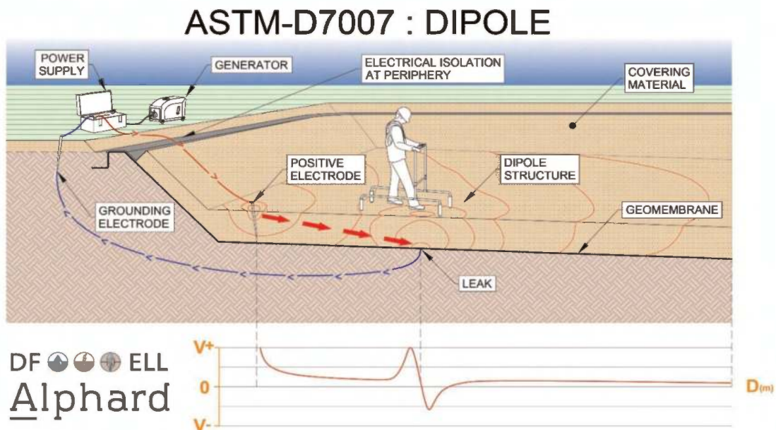
Figure 2. Dipole method schematic.
