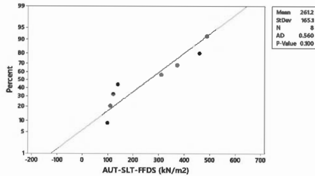
Figure 3. Anderson-Darling test results for AUT-SLT-FFDS ( \text{kN}\cdot\text{m}^2 ).
