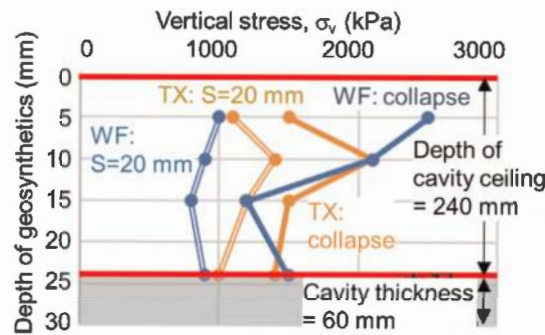
Figure 10. \sigma_v to cause S=20 mm and collapse.
