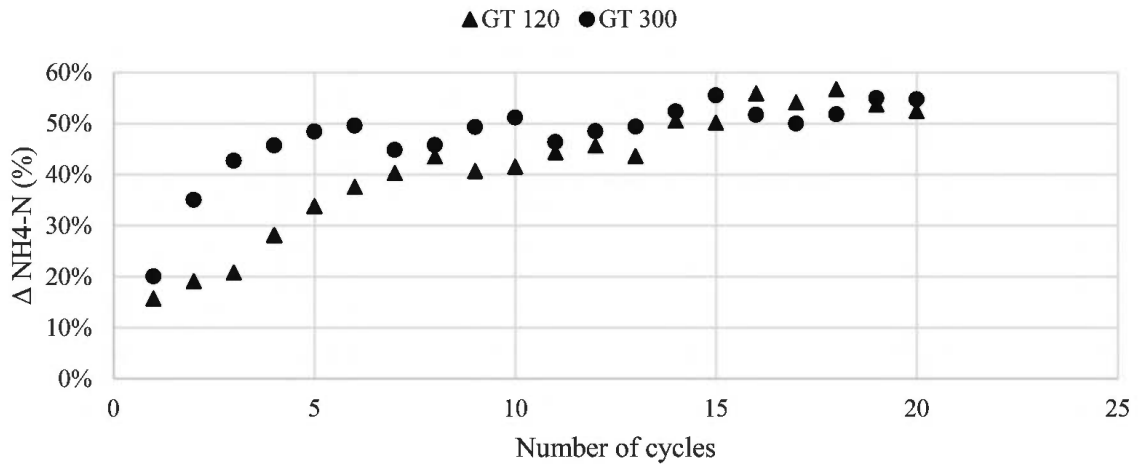
Figure 2. Variation of \text{NH}_4\text{-N} removal in permeameters.
