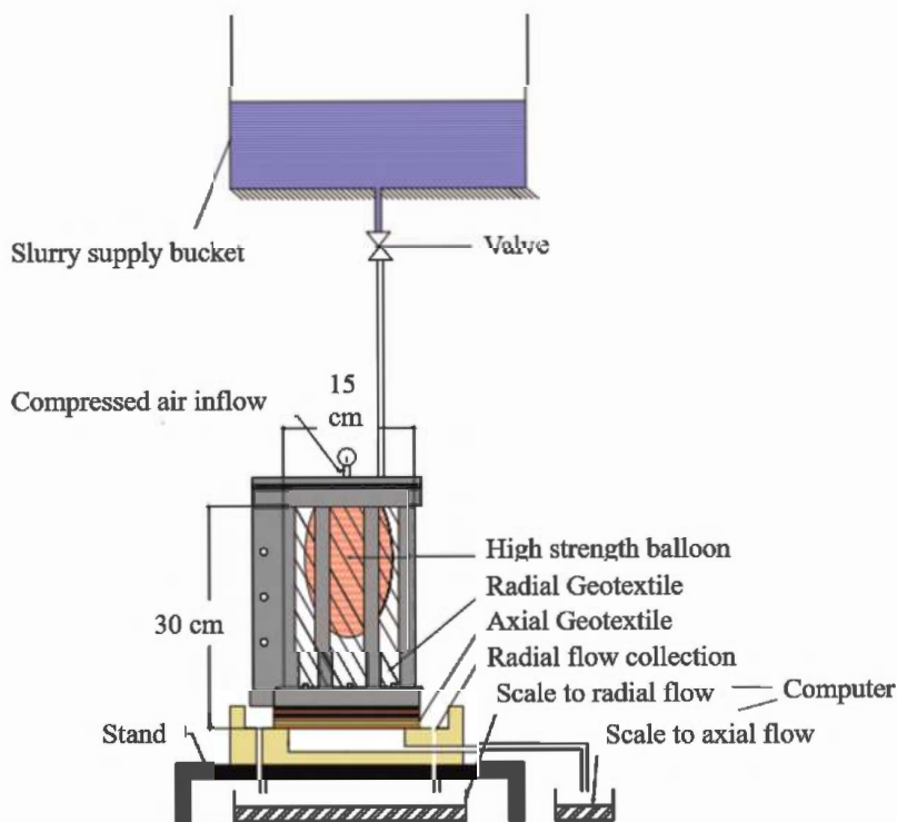
Figure 1. Schematic diagram of P2DT setup.
