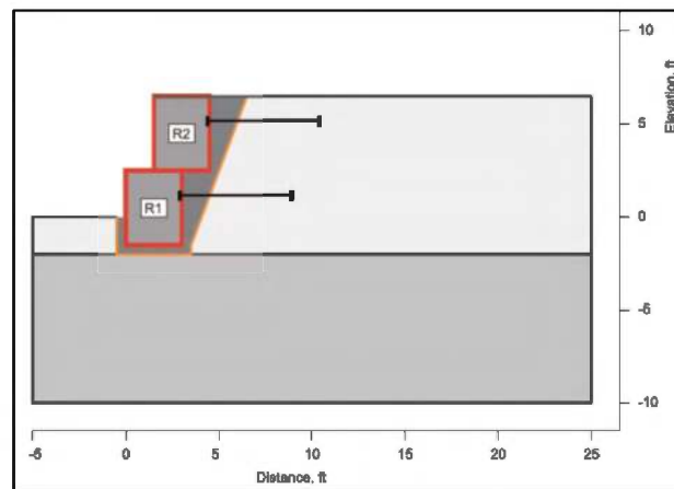
Figure 4. 1-1 Anchored SCOURLOK configuration.
