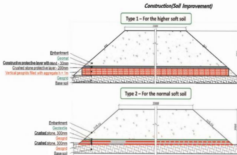
Figure 3. General design solution.
