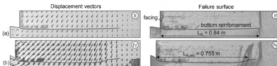
Figure 5. Total displacements vectors (a) and failure surface (b) in small-scale test.
