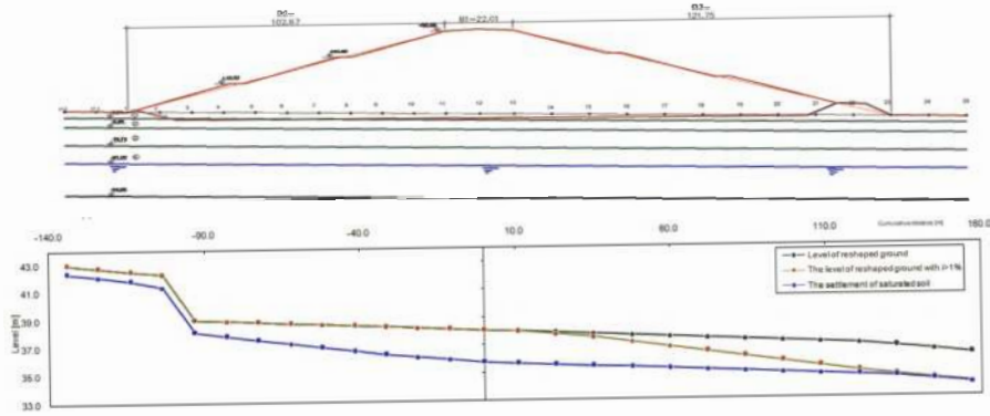
Figure 7. Reshaping the slope of the base of the landfill in order to obtain a slope >1\% after consumption of the settlements.
