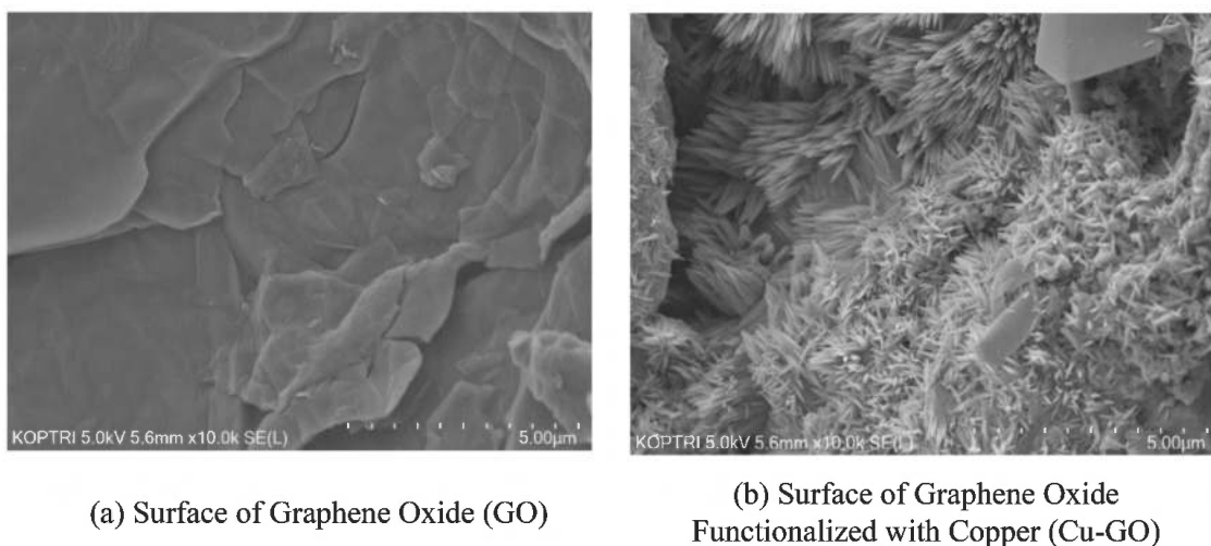
Figure 1. Confirmation of functionalization by SEM.
