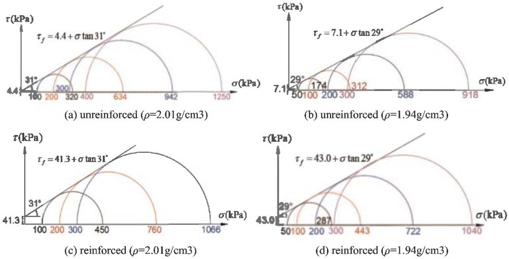
Figure 5. Mohr circles of unreinforced and reinforced clay.
