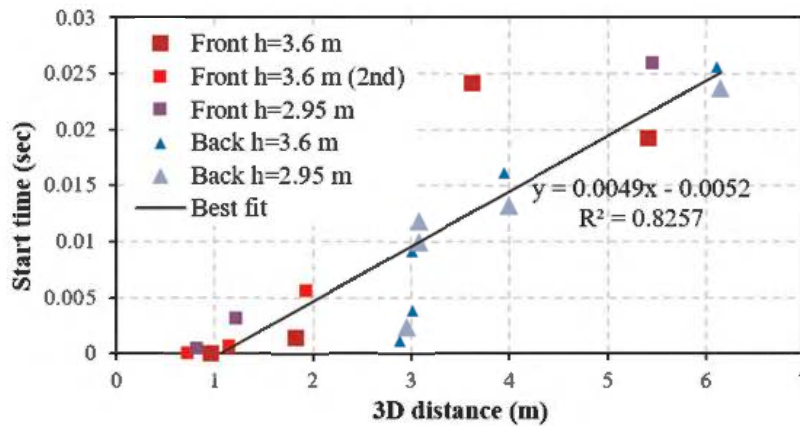
Figure 6. Determination of the impact wave propagation speed.
