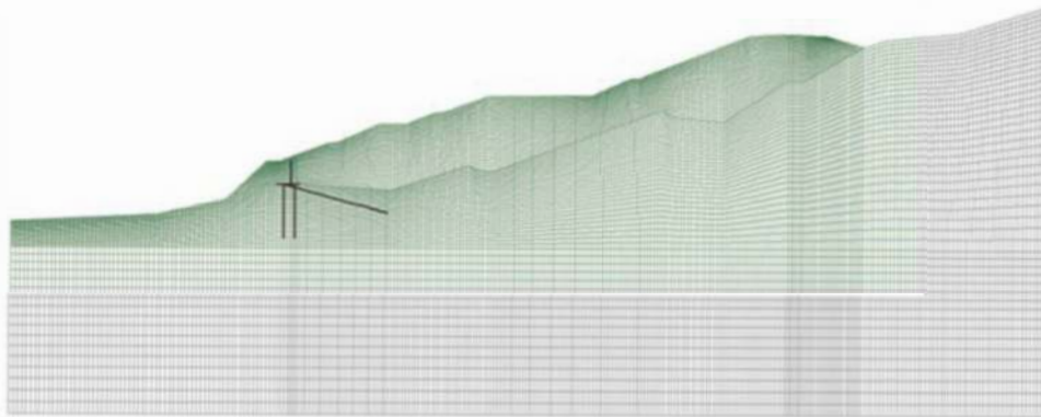
Figure 3. FLAC-2D model.
