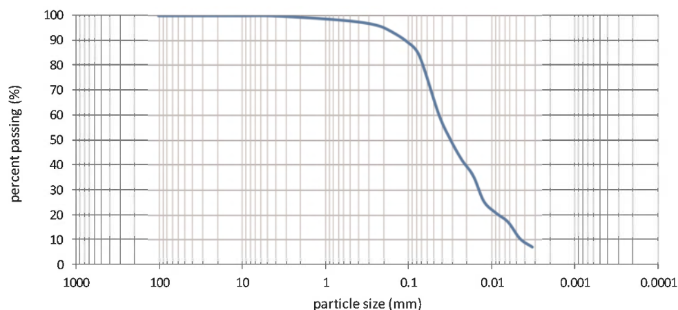
Figure 4. Particle size distribution of the tested soil.
