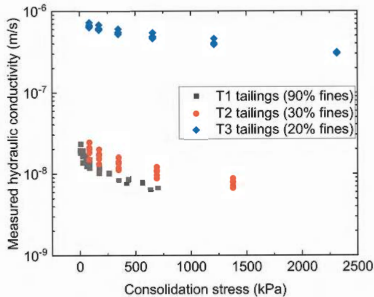
Figure 3. Measured hydraulic conductivity of three tailings via the stress-dependent permeameter by Fan et al. (2022) (Notes: hydraulic conductivity was first presented by Fan and Rowe (2022a) for T1, Rowe and Fan (2022) for T2, Fan and Rowe (2022b) for T3).
