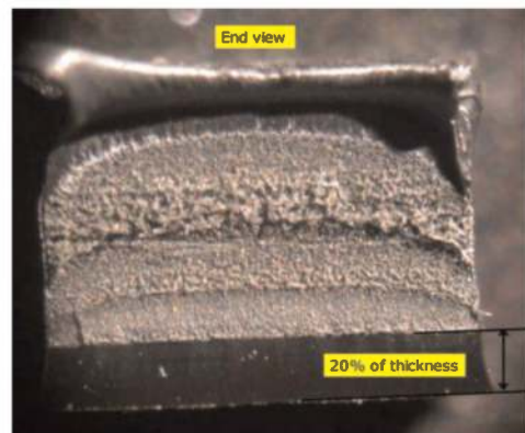
Figure 5. Verifying notch depth.
