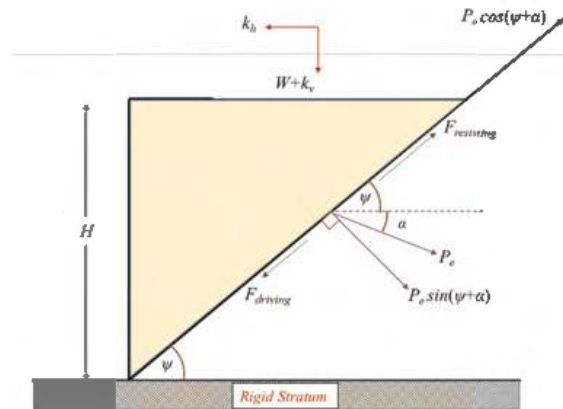
Figure 1. Free-body diagram of a RW.
