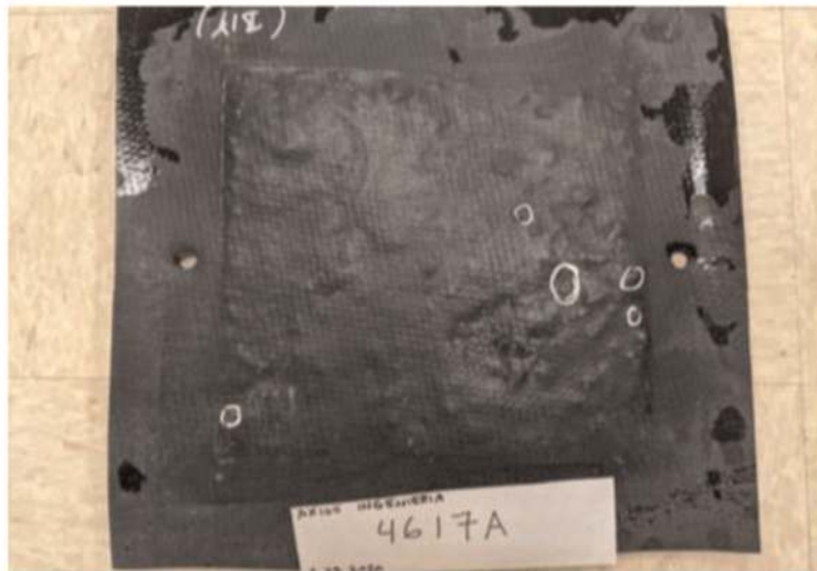
Figure 4. 2mm HDPE Geomembrane after puncture test.
