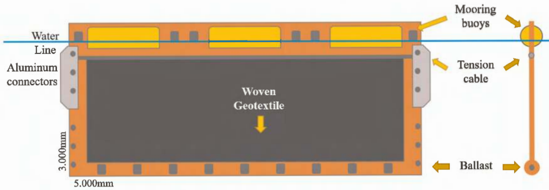
Figure 1. Schematic drawing of the curtains.
