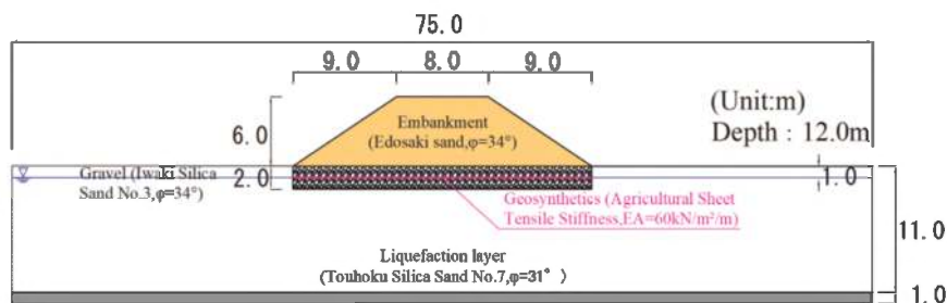
Figure 1. Outline of model ground.
