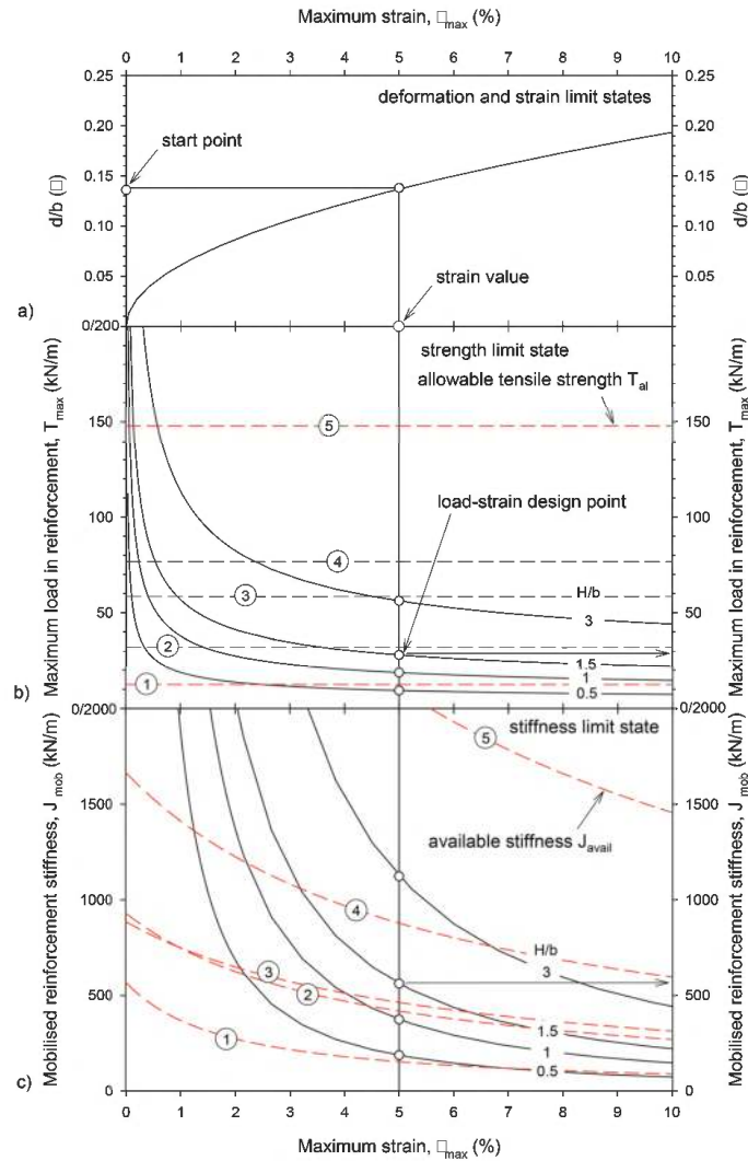
Figure 2. Flow chart illustrating calculation steps for an unsurcharged reinforced fill layer over a long void using BS 8006-1 (2010) method for: a) deformation and reinforcement strain limit states; b) maximum reinforcement tensile strength limit state, and; c) reinforcement stiffness limit state. Problem parameters: b = 1 m, H = 0.5, 1, 1.5 and 3 m, \gamma = 18 kN/m 3 and \phi = 35^\circ .
