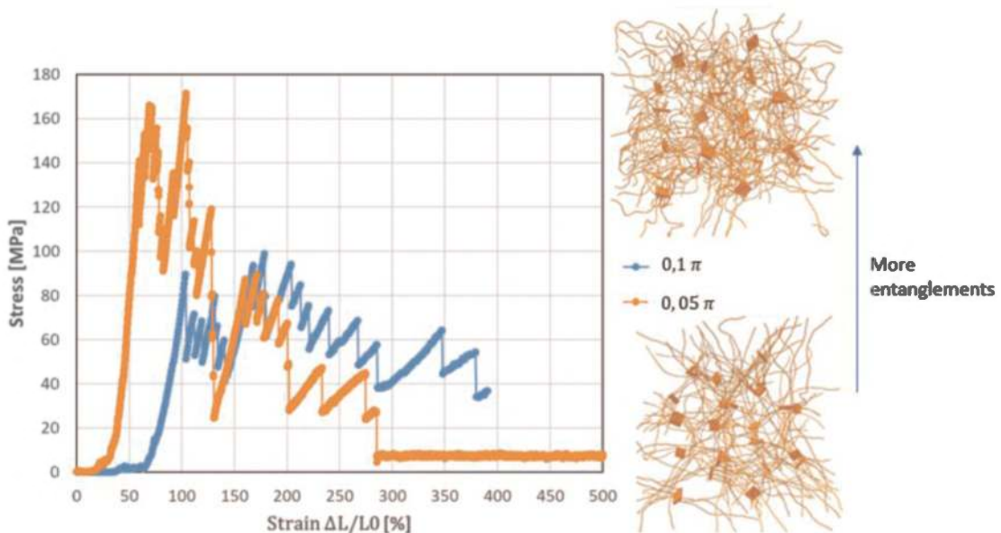
Figure 7. Preliminary results of the stress strain behavior under Traction Test of two different configurations of PVC geomembrane microstructure with two different values of \theta_{\max} .
