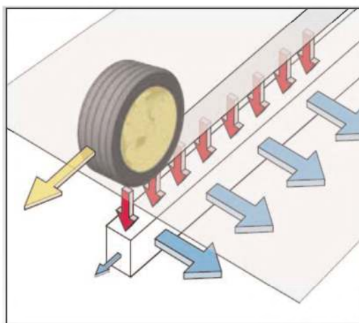
Figure 1. Geogrid in plain strain-stress condition.
