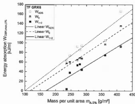
Figure 9. Example of the EA in ADS W_{ADS} , after damaging “between the wheels” W_0 and after damaging “under the wheels” W_{1+2} shown as EA vs. mass per unit area.
