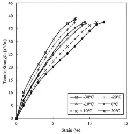
Figure 4. Load-strain curves of the geocomposite at temperatures ranging from -30^{\circ}\text{C} to 20^{\circ}\text{C} .
