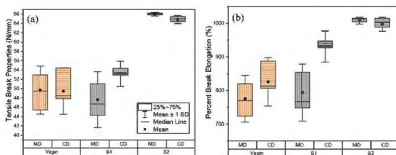
Figure 5. Box plots of tensile break strength (a) and percent break elongation (b) obtained with the virgin and the exhumed HDPE GMs.
