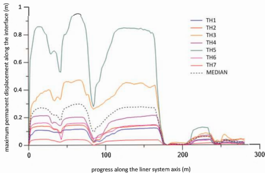
Figure 6. Maximum permanent displacements along the liner system at the end of the two-dimensional dynamic analyses (displacements in m).
