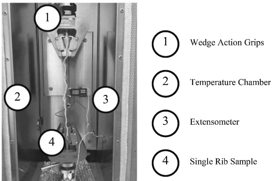
Figure 1. MTS testing machine and its temperature chamber.
