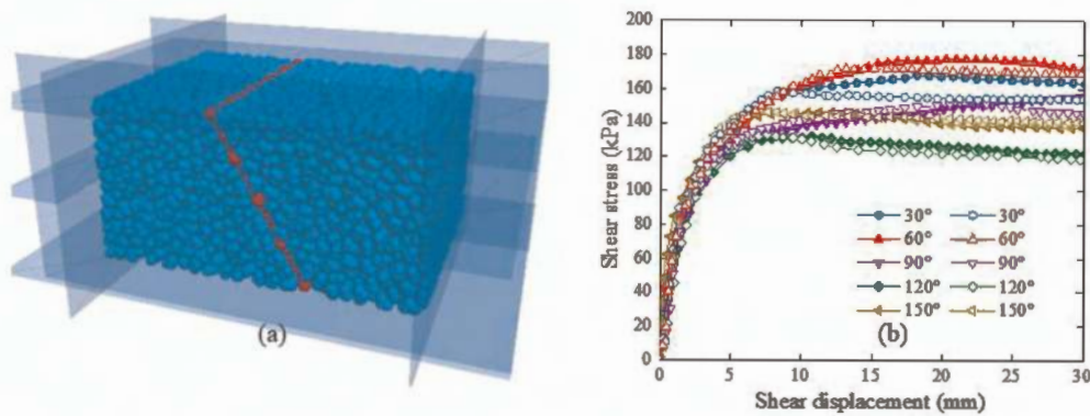
Figure 6. Discrete element simulation (a) Numerical model (b) The comparison curve of shear test and simulation results for different angles of geogrid under vertical stress of 200 kPa.
