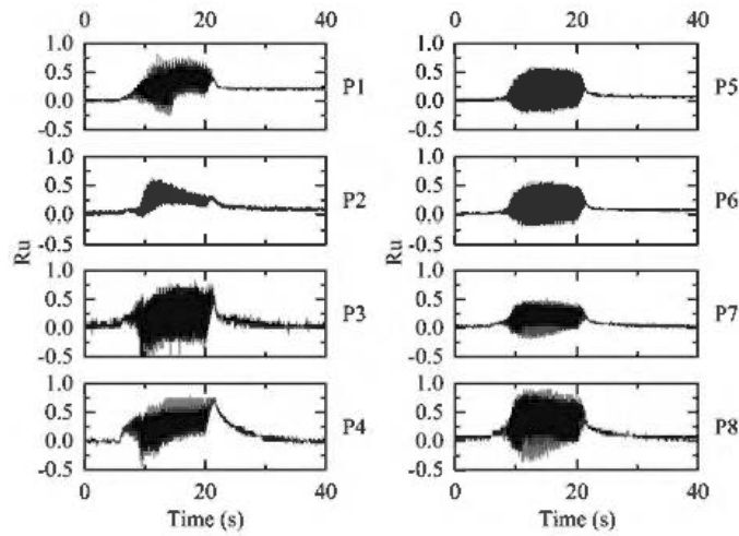
Figure 6. Time history of R_u in Case 1.
