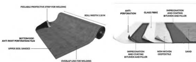
Figure 3. BGM structure.
