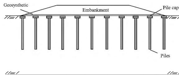
Figure 1. Pile-supported embankment with geosynthetics.
