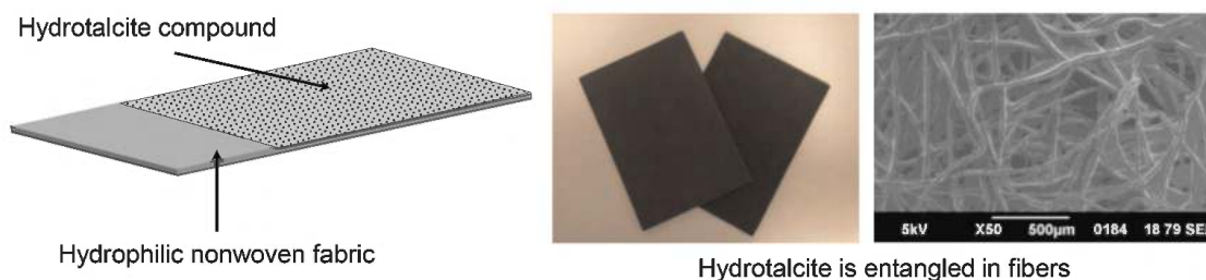
Figure 2. Geosynthetic sorption sheet used in this study.
