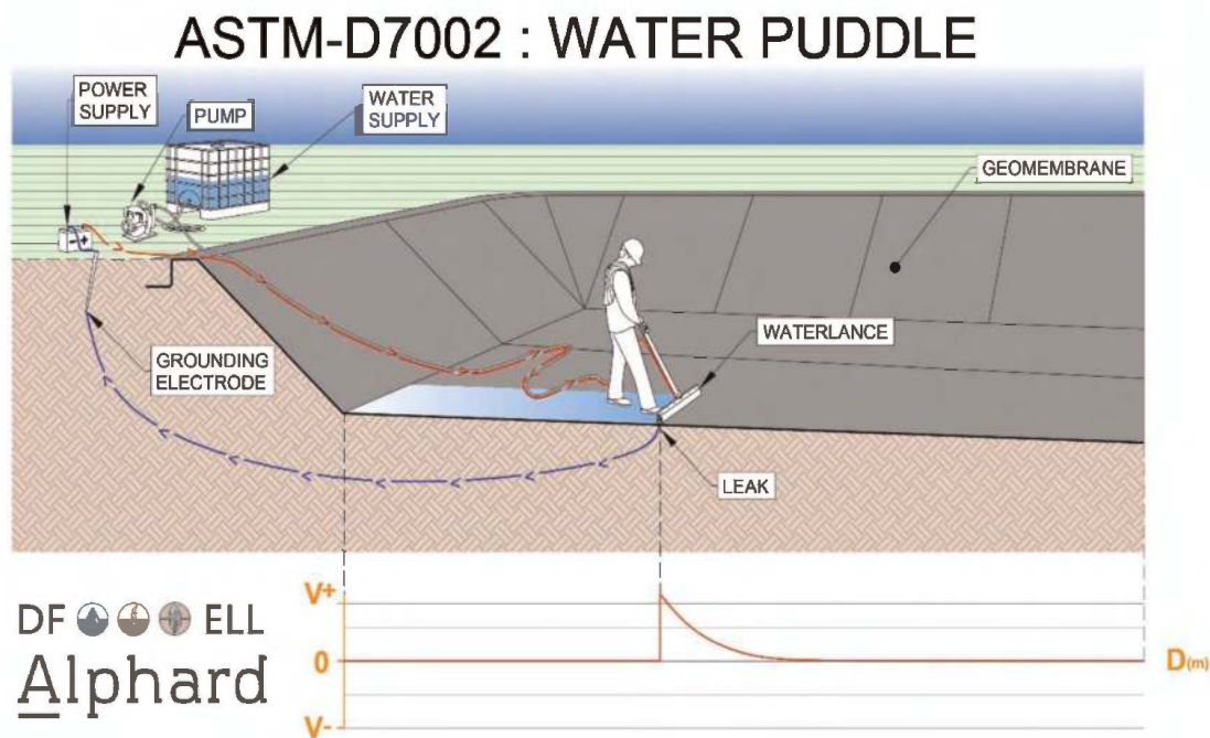
Figure 1. Water puddle method schematic.
