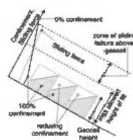
Figure 1b. Geocell confinement.
