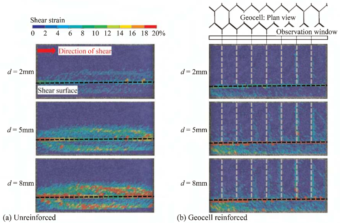
Figure 5. Development of shear displacement in soil.
