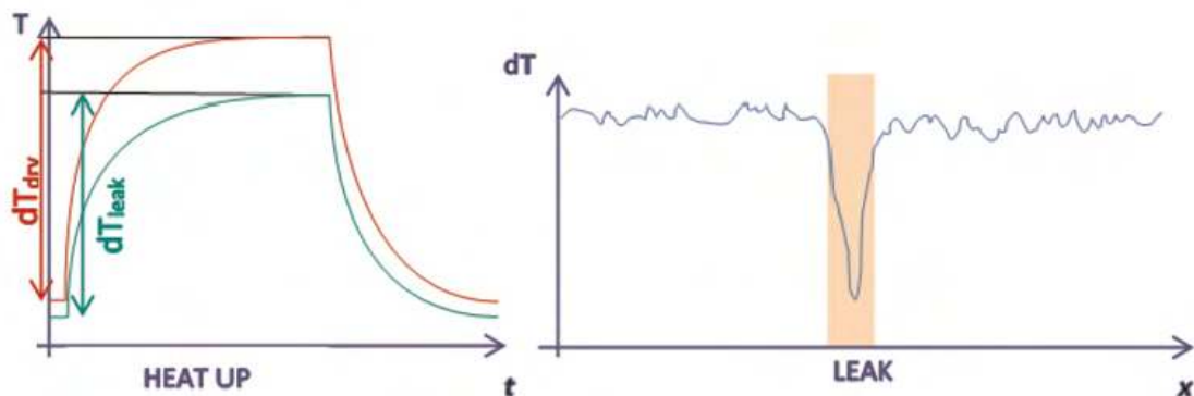
Figure 2. HPM principle.
