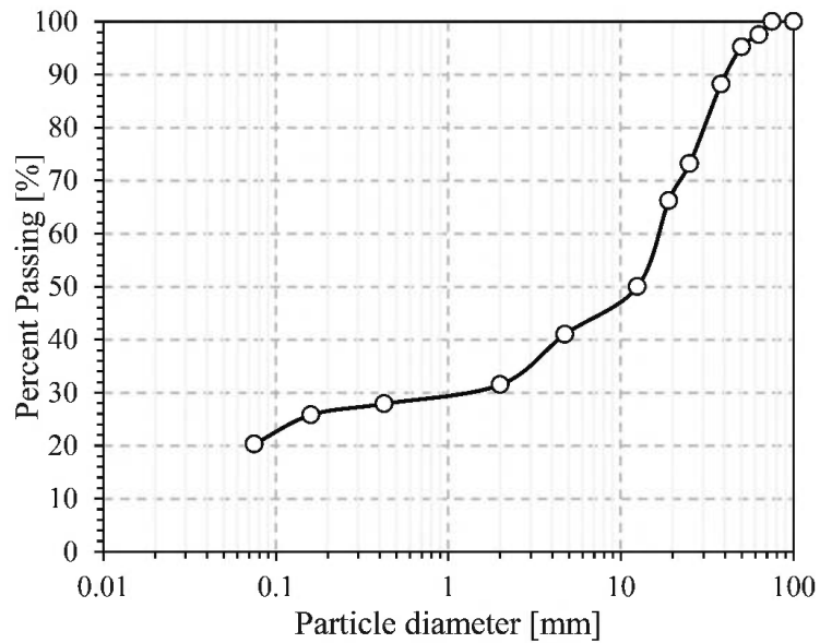
Figure 3. Overliner grain-size curve.
