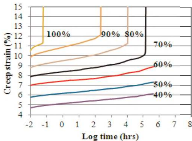
Figure 1. Creep properties of carbon geogrid.
