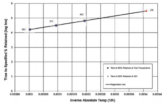
Figure 4. Degradation curve of Geogrid B in pH 11.4.
