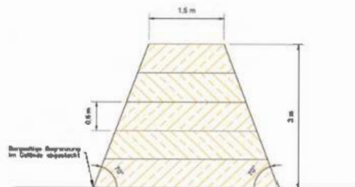
Figure 8. Cross section of the protection dam.
