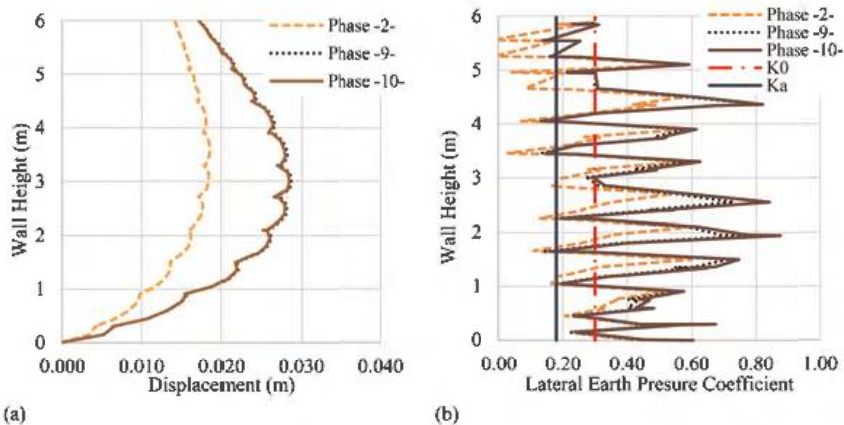
Figure 2. (a) Displacement directly behind the wall & (b) Lateral earth pressure coefficient directly behind the wall.
