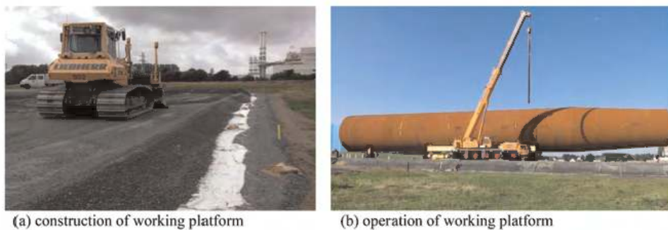
Figure 11. Geosynthetic reinforced working platform (Nordenham, Germany).
