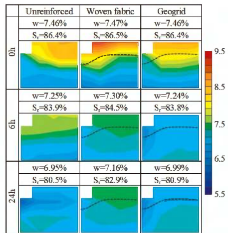
Figure 9. Distribution of water content on elapsed time.
