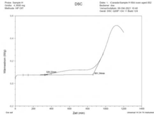
Figure 1. HP-OIT with shoulder.
