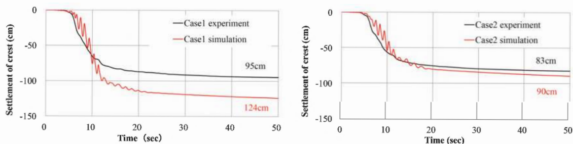
Figure 5. Relation of embankment settlement against times(Experiment · Simulation).
