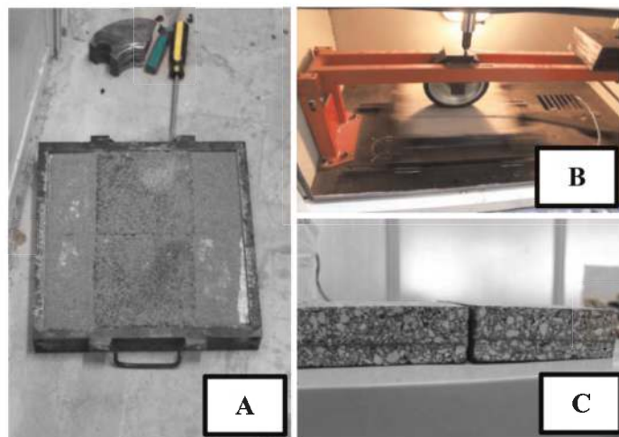
Figure 1. Specimen preparation and rutting test set-up.
