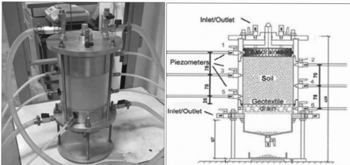
Figure 1. Test apparatus (Moraci et al. 2023).
