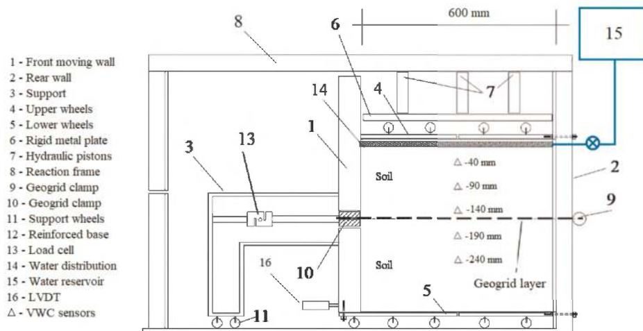
Figure 1. Geosynthetic reinforcement layer experimental device.
