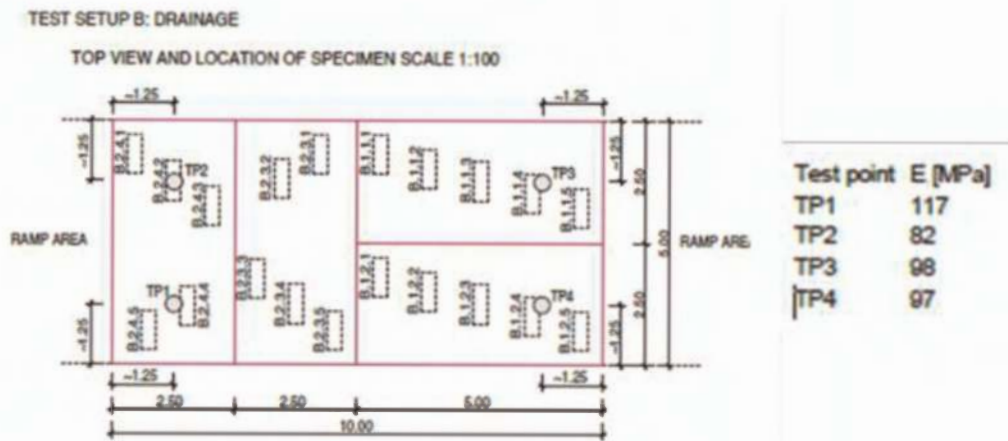
Figure 3. Arrangement of drainage geosynthetic samples.
