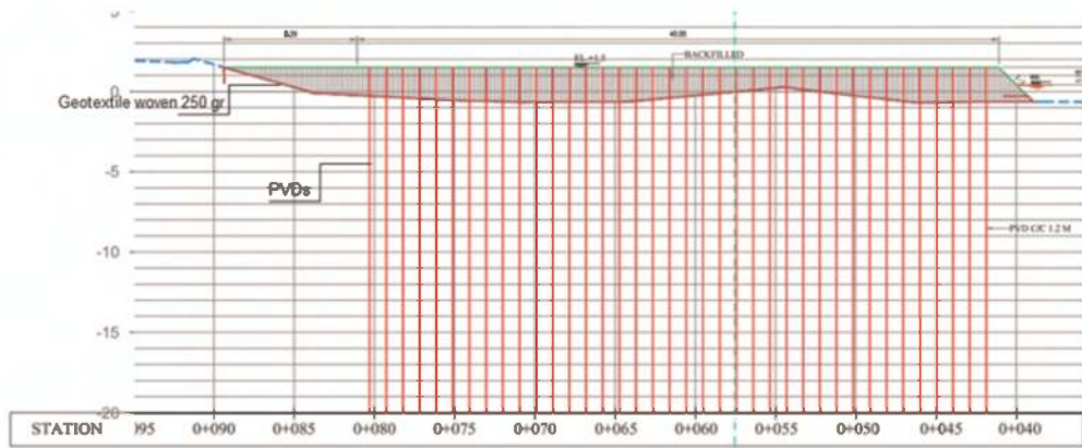
Figure 2. The long section of the test area.
