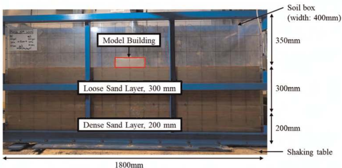
Figure 2. Test model on the 1-g shaking table.
