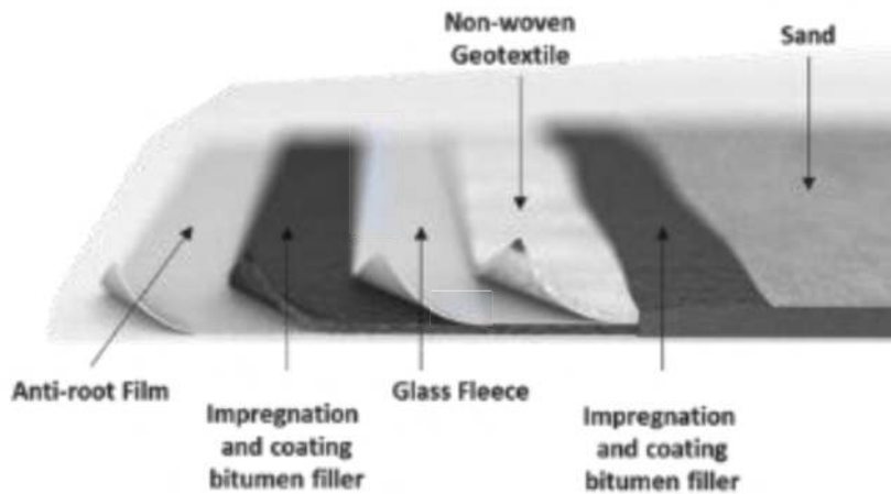
Figure 1. BGM structure.
