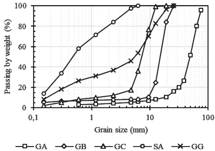
Figure 1. Grain size curves of RCDW.
