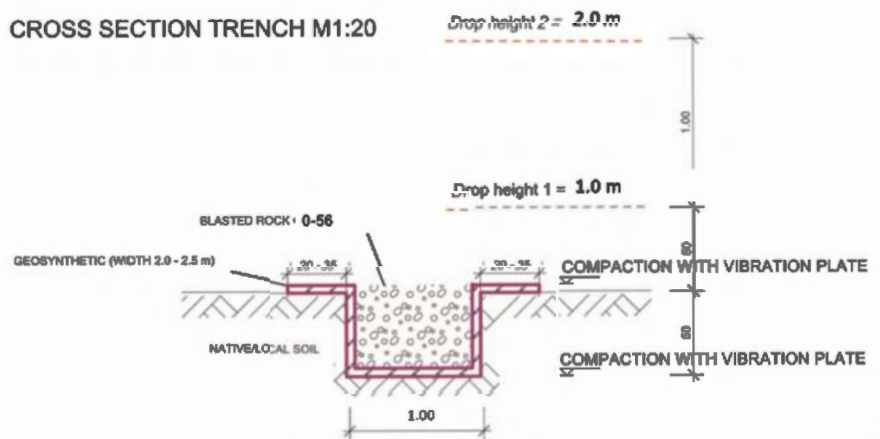
Figure 3. Cross section of the drainage trench.
