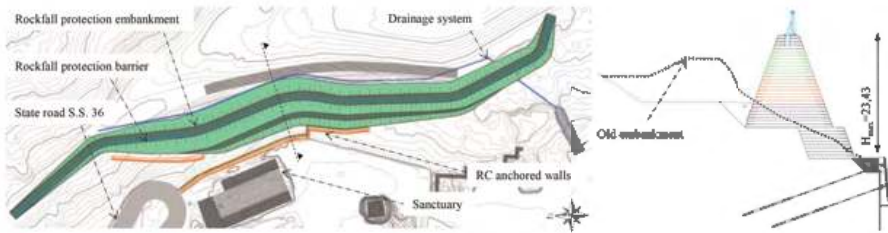
Figure 3. Plan view and typical cross-section.
