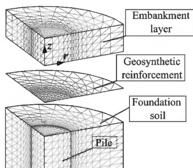
Figure 2. FLAC3D numerical model layout and spatial discretization.
