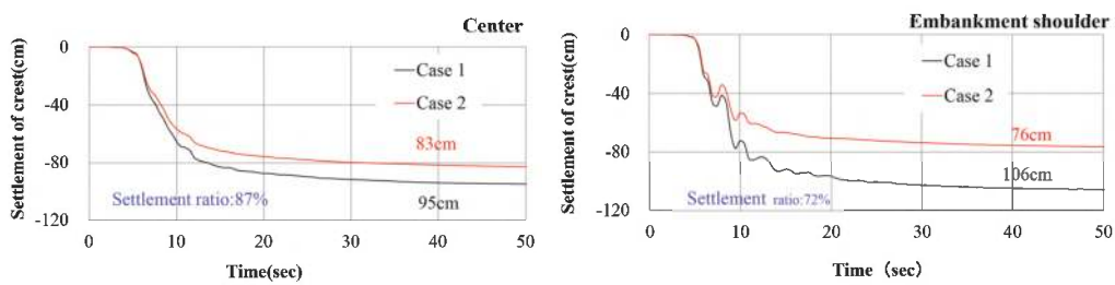
Figure 2. Relation of embankment crest settlement with times.
