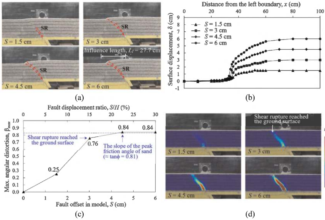
Figure 3. Results of the unreinforced foundation test (Test U) at various fault offsets: (a) test images; (b) surface displacement profiles; (c) maximum angular distortion; (d) shear strain contours.
