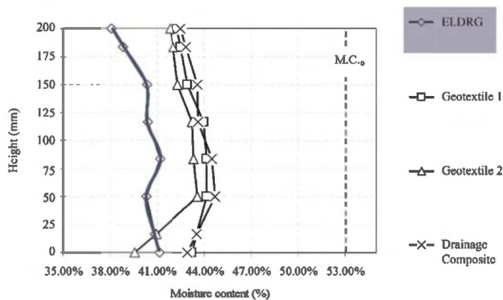
Figure 1. Rain infiltration tests (Zhang et al. 2009).
