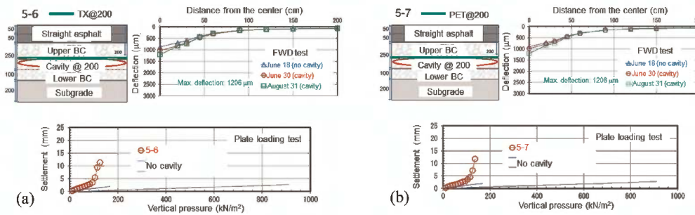
Figure 5. Loading tests on the cavities at 200 mm. (a) 5-6 (TX at 200 mm). (b) 5-7 (PET at 200 mm).
