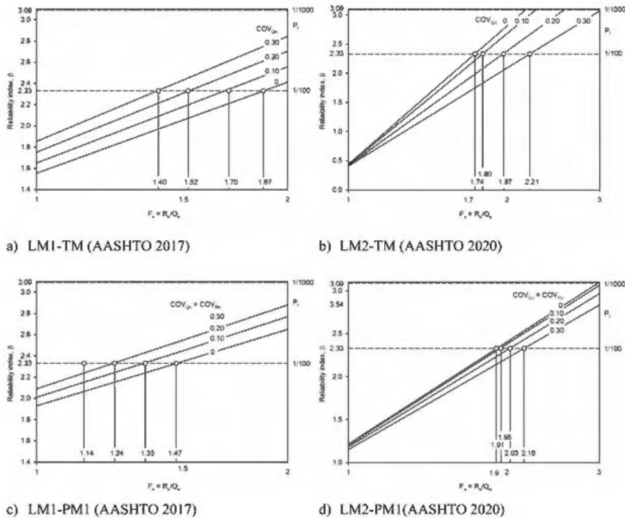
Figure 3. Reliability index versus ratio of nominal resistance to nominal load. a) LM1-TM (AASHTO 2017) b) LM2-TM (AASHTO 2020) c) LM1-PM1 (AASHTO 2017) d) LM2-PM1 (AASHTO 2020).
