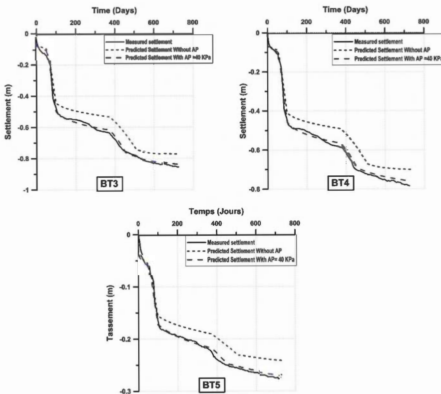
Figure 5. Measured and predicted settlements under the embankment.
