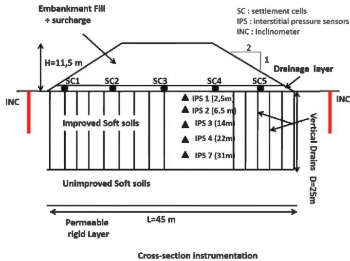
Figure 3. Field monitoring and PVD's arrangement.
