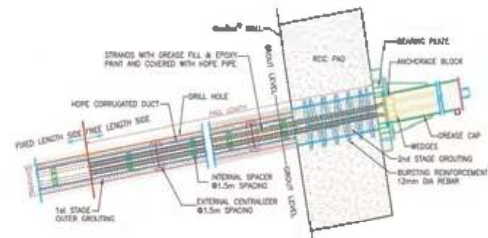
Figure 4. Typical ground anchor detail.
