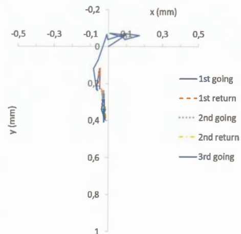
Figure 10. Trajectory of the marker fixed to geogrid.
