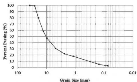
Figure 4. Grain size distribution for the base course.
