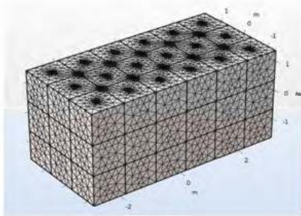
Figure 4. Meshing of the model (Sayami 2021).
