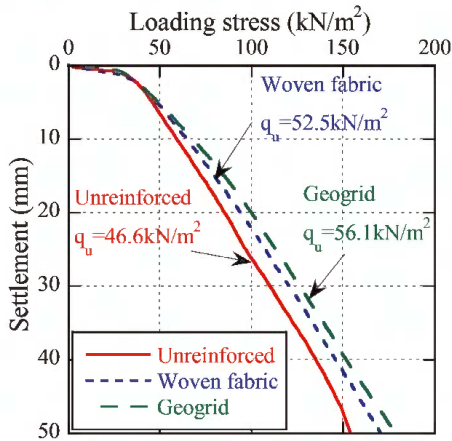
Figure 5. Loading stress and settlement.
