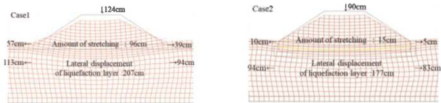
Figure 7. Deformation after seismic motion.
