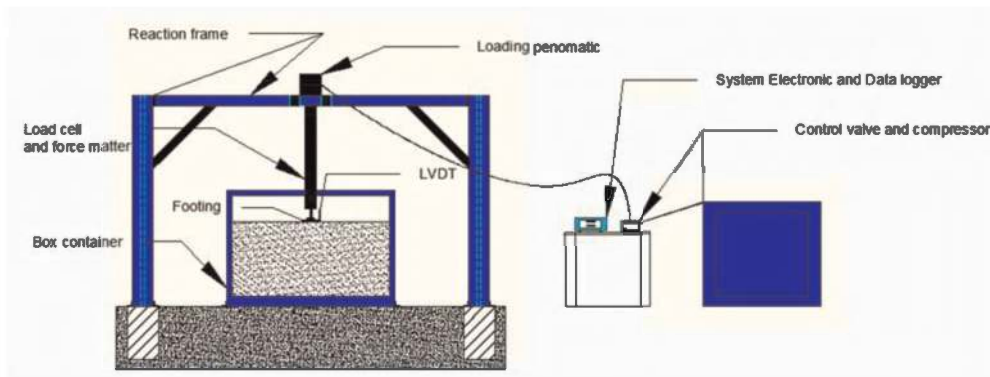
Figure 2. Schematic view of the experimental model study.
