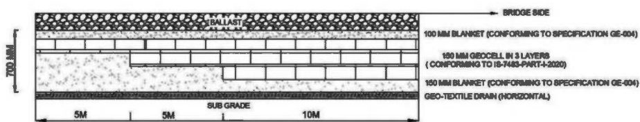
Figure 3. Section for trials.
