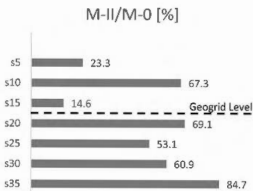
Figure 7. Lateral pressures in M-II vs M-0 (%).
