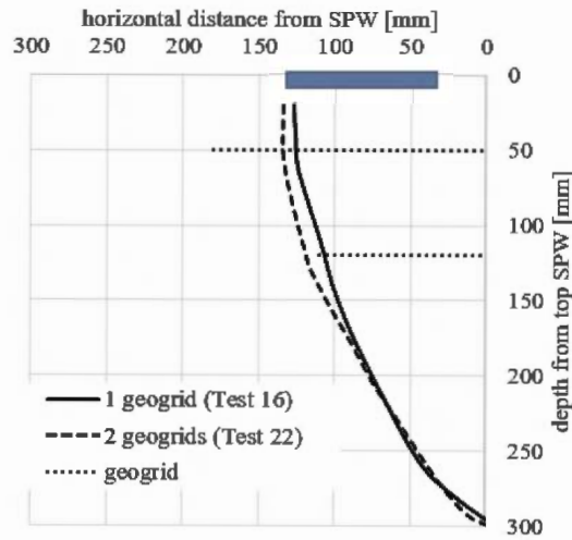
Figure 6. Slip planes for 1 or 2 geogrids.
