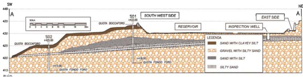
Figure 4. Geological longitudinal section of the drainage system.
