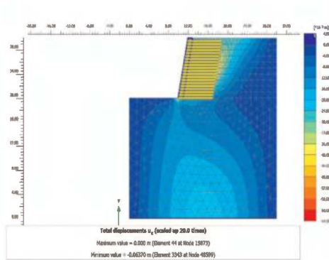
Figure 6. Vertical displacement.
