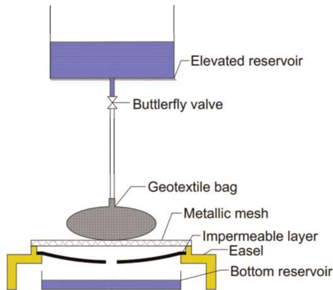
Figure 2. Schematic diagram of GDT setup.
