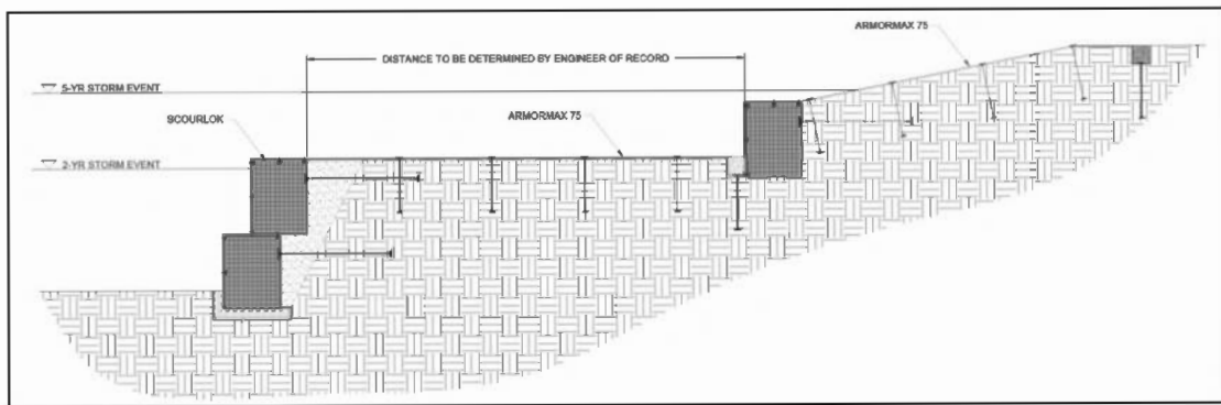
Figure 3. SCOURLOK / ARMORMAX Riverbank cross-section configuration.
