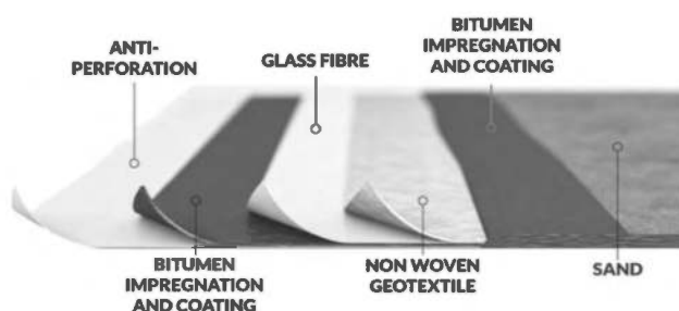
Figure 1. Diagram of a typical BGM composition.
