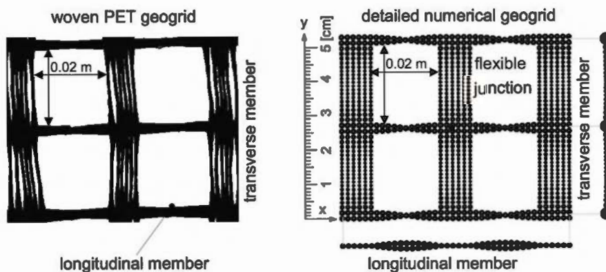
Figure 1. Woven PET geogrid Fortrac® by Huesker and its numerical model (modified from Dijak 2012).
