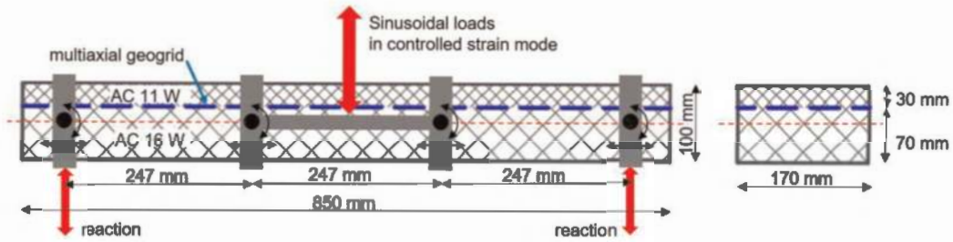
Figure 2. Scheme of the 4PB test configuration.
