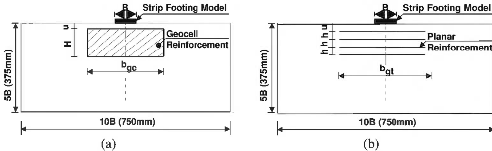
Figure 9. Geometry of the (a) geocell reinforced foundation bed (b) geotextile reinforced foundation bed (Moghaddas Tafreshi & Dawson 2010).
