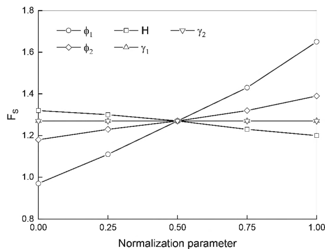
Figure 2. Sensitivity analysis of GRSS at Yeager airport.
