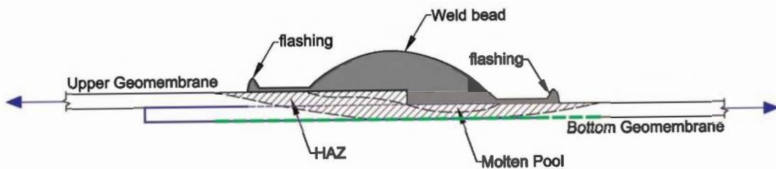
Figure 1. Cross-section of typical HDPE extrusion weld.
