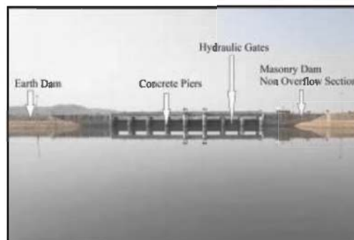
Figure 1. Components of a typical dam - upstream view.
