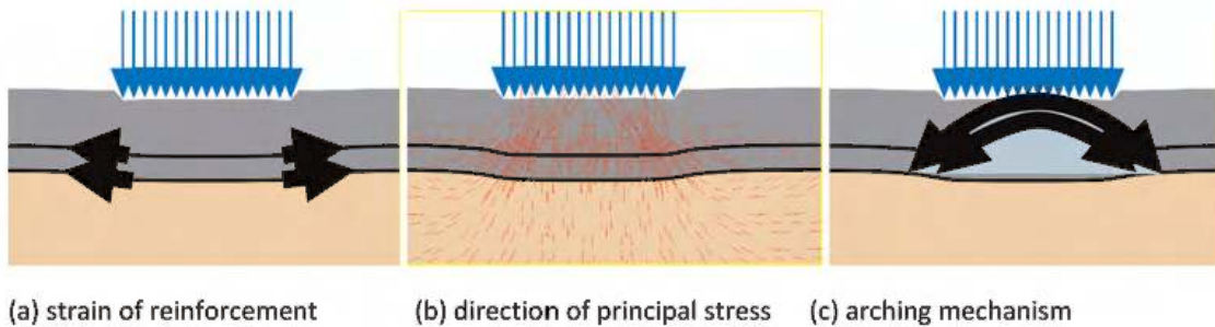
Figure 4. Load transfer mechanism in the working platform.
