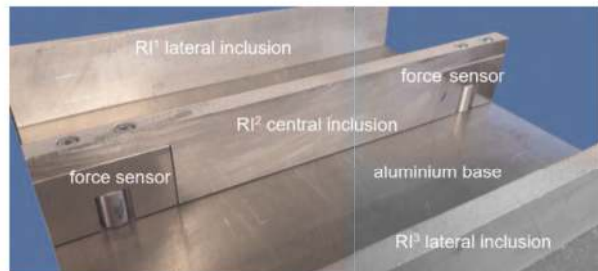
Figure 7. Location of vertical force sensors.
