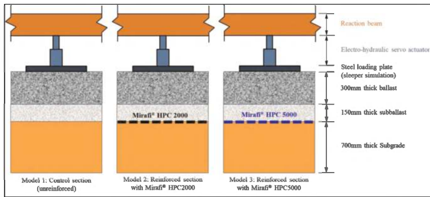
Figure 3. Typical section of steel test box and loading apparatus.
