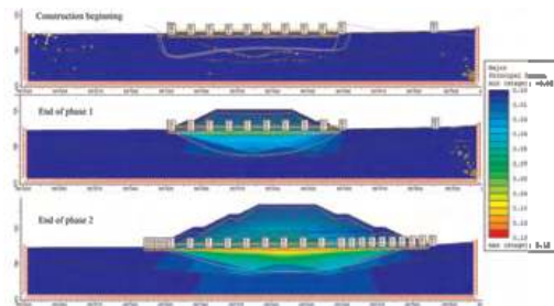
Figure 2. Maximum principal strain at the liner layer.
