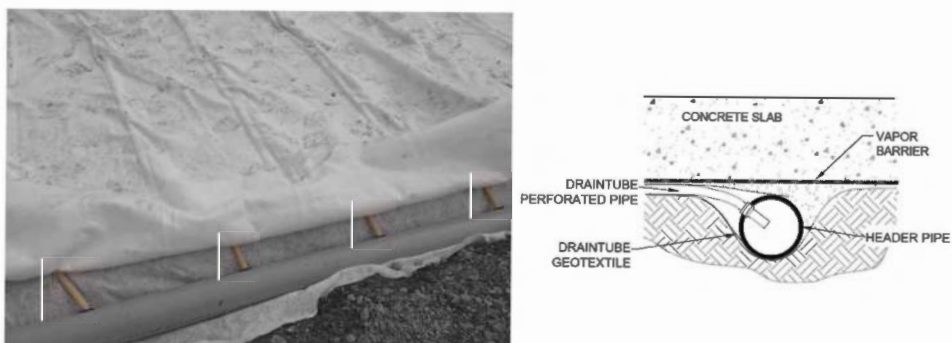
Figure 3. Connection to the header pipe.
