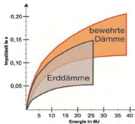
Figure 9. Impact time and energy absorbed.
