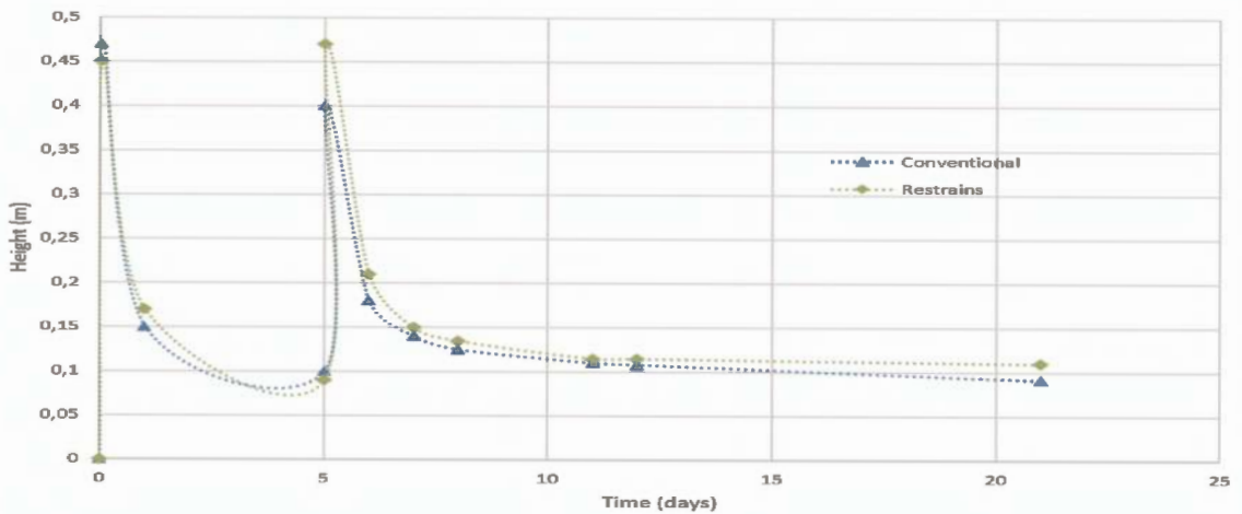
Figure 2. Filling heights per time.
