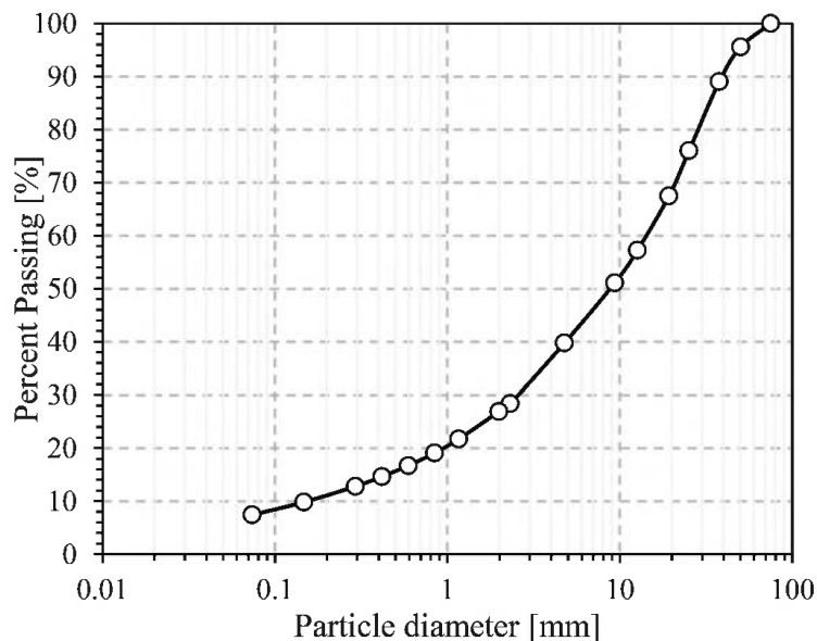
Figure 6. Overliner materials sieve analysis curve.
