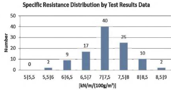
Figure 9. Specific tensile strength by test results.
