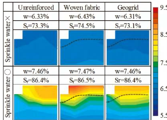
Figure 7. Distribution of water content on water infiltration.
