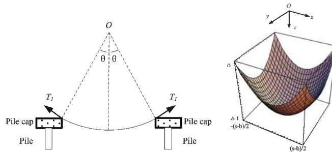
Figure 3. Settlement analysis of the two regions.
