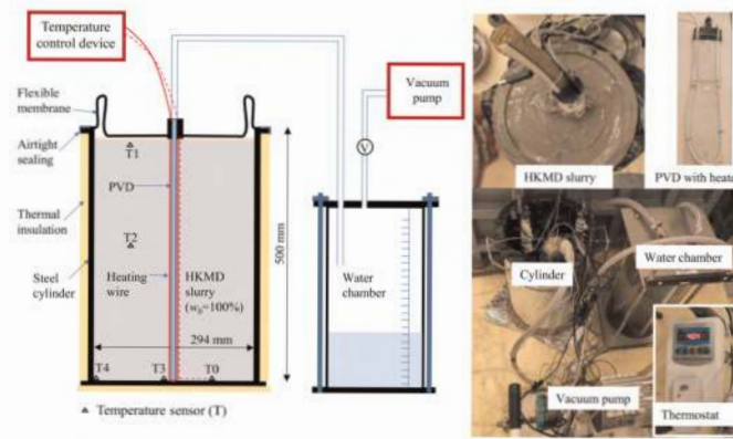
Figure 2. Setup of the model test.
