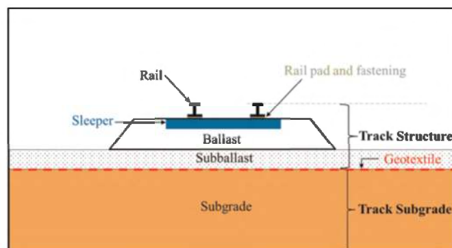
Figure 1. Typical section of railway track.
