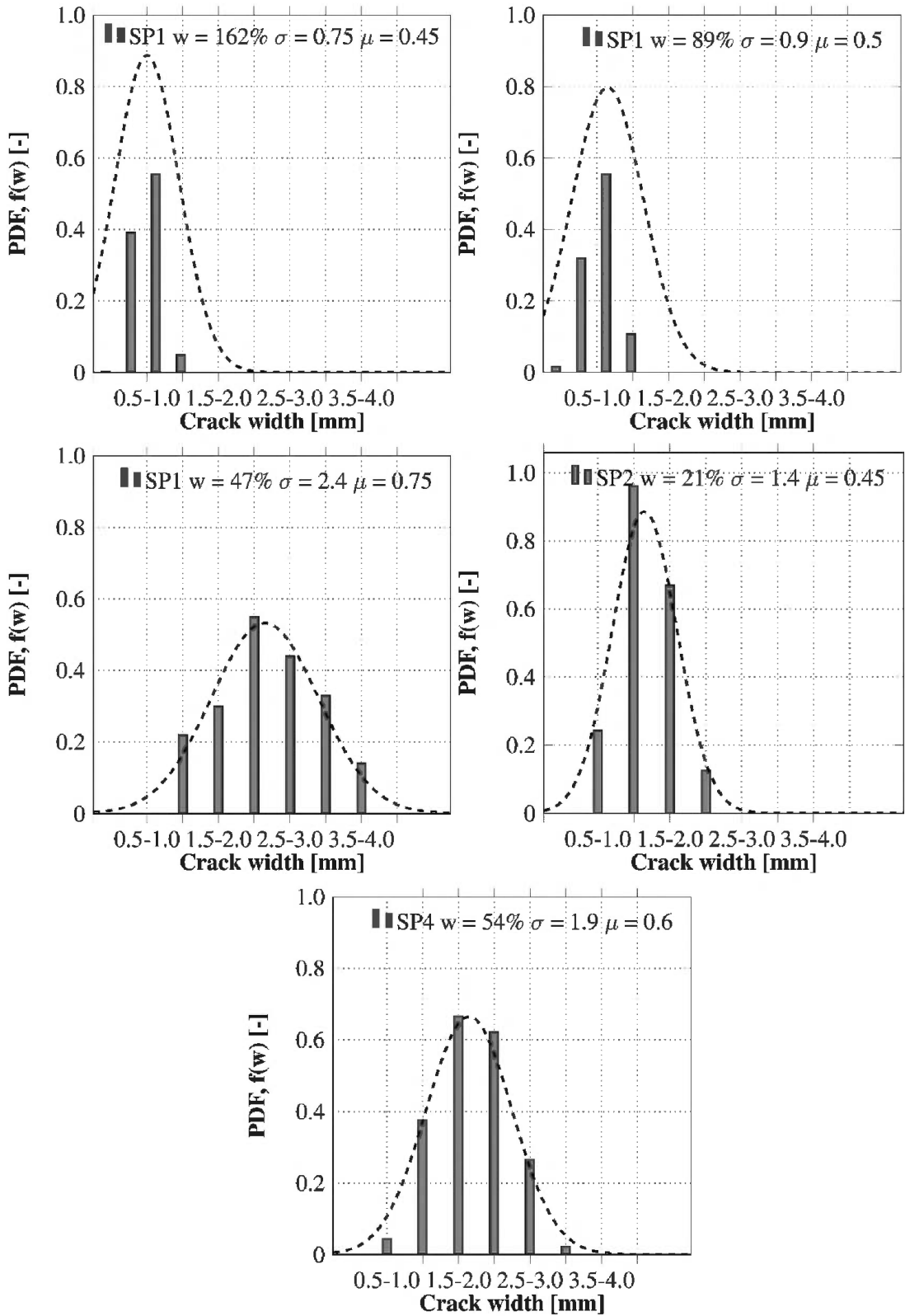
Figure 2. Probability density function of crack width for SP1, SP2 and SP4 at different water contents.
