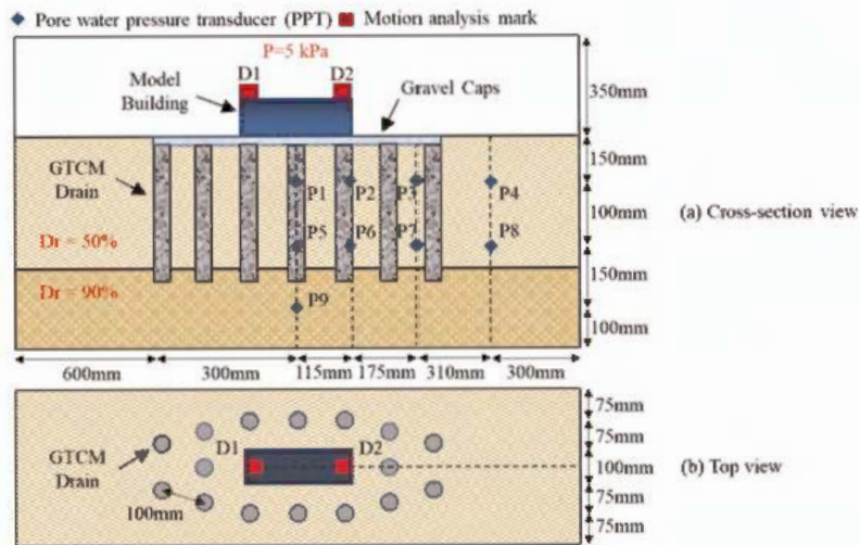
Figure 3. Layout of model test Case 1.
