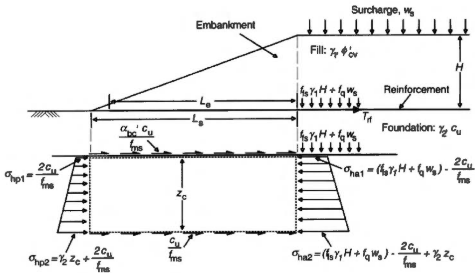
Figure 4. Analysis of foundation extrusion stability.
