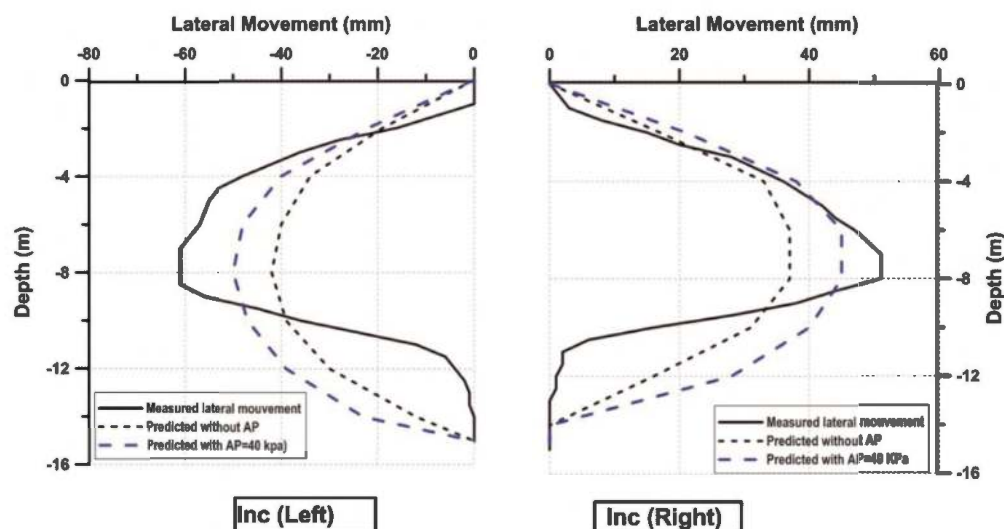
Figure 6. Measured and predicted lateral movements.
