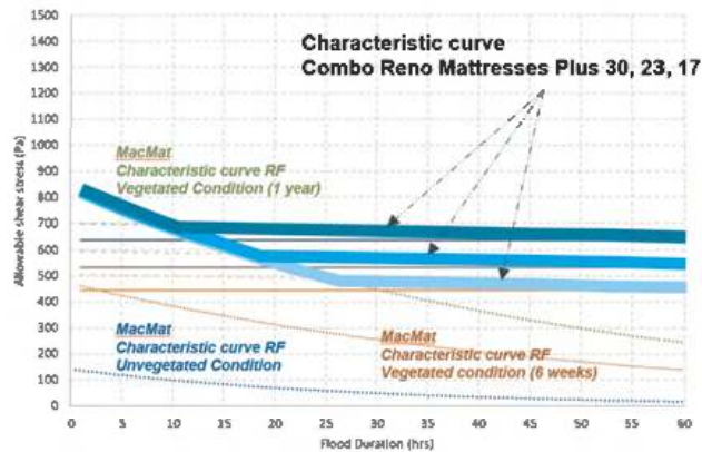
Figure 7. Design chart for Maccaferri Reno Mattresses Plus.
