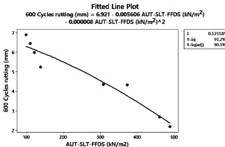
Figure 7. Overlay shear bonding versus rut depth.
