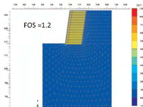
Figure 7. Factor of safety.
