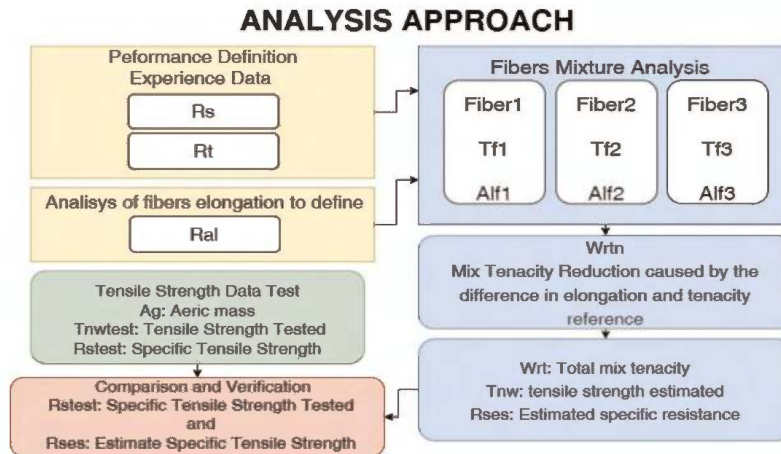
Figure 1. Approach scheme.
