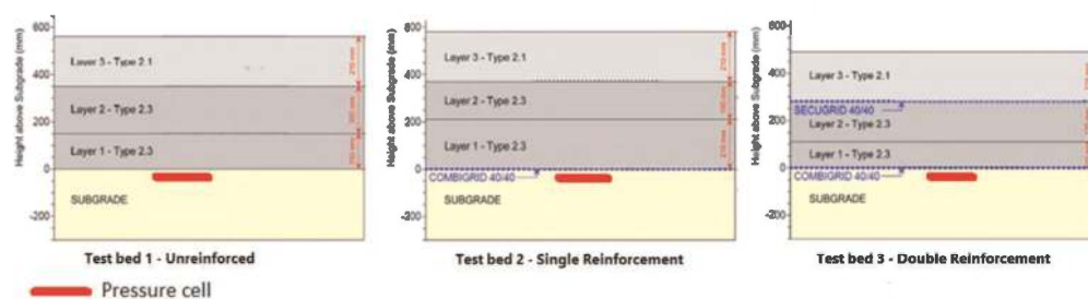
Figure 1. Test cross sections.
