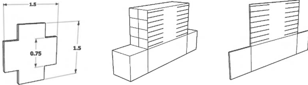
Figure 2. Three-dimensional view of a back-to-back reinforced wall.
