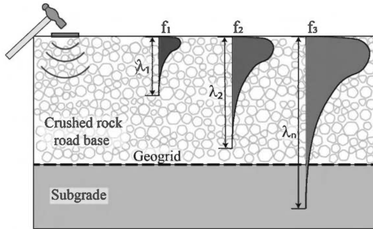
Figure 1. Surface wave analysis through aggregate.
