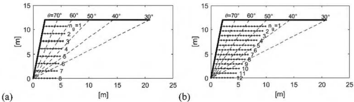
Figure 2. Sketch of (a) disposal 1 and (b) disposal 2.
