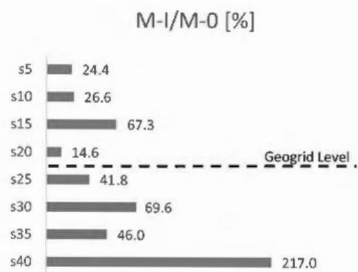
Figure 6. Lateral pressures in M-I vs M-0 (%).
