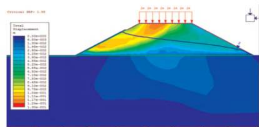
Figure 6. Output: Failure surface with displacement contours.
