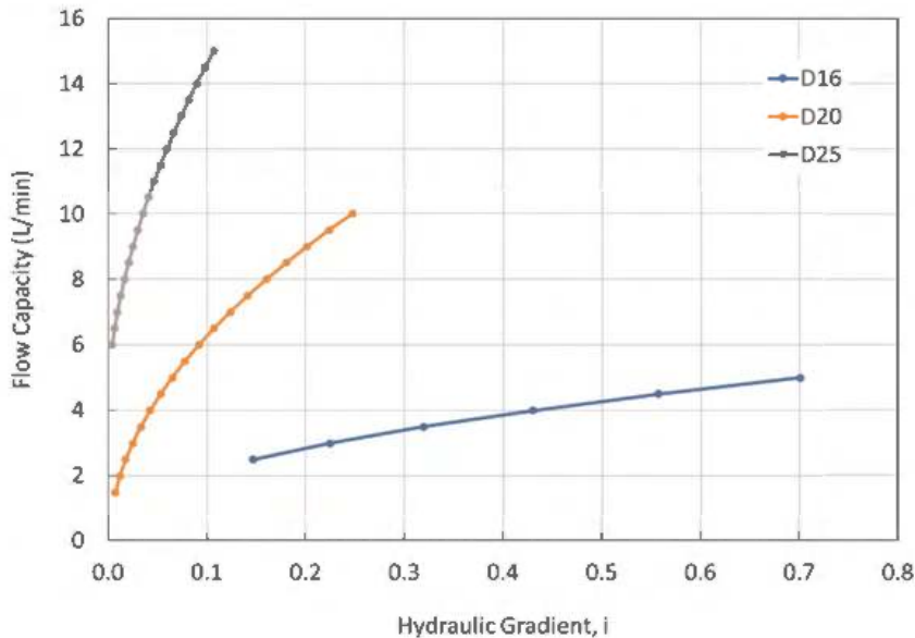
Figure 3. Flow capacity of the 3 mini-pipe diameters.
