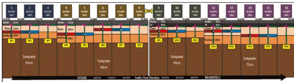
Figure 1. Schematic representation of the trial road.
