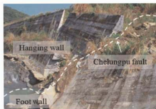
Figure 2. Failure of reinforced concrete revetments caused by Chelungpu fault (Chiang et al. 2022).
