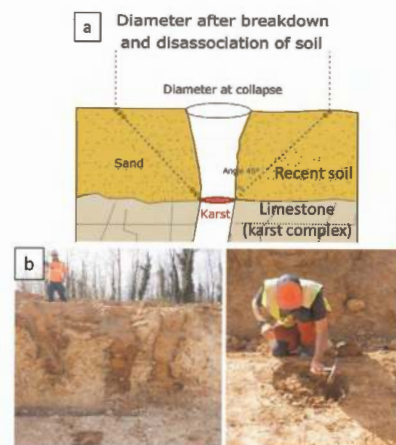
Figure 5. Hourglass effect (a), karstic wells (b).
