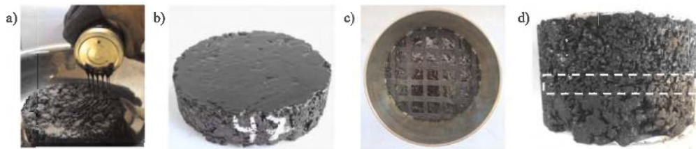
Figure 2. Specimen preparation: (a) applying asphalt binder tack coat; (b) lower layer surface after tack coat application; (c) geosynthetic installed; (d) double layered specimen.
