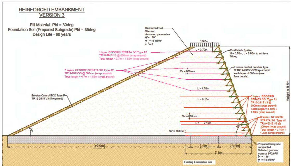
Figure 5. Cross-section design of bund.
