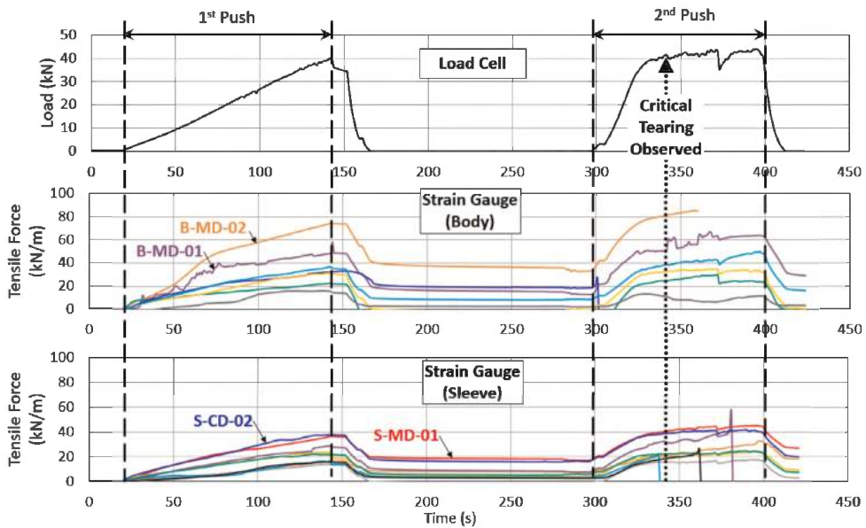
Figure 8. Results of inlet port test T2.
