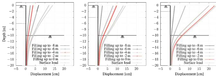
Figure 6. Sheet pile wall deformation for all backfilling phases for Geogrid at -6 m (left), at -4 m (middle) and at -2 m (right).
