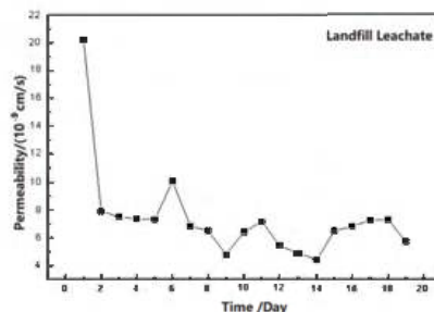
Figure 4. Effect of landfill leachate on permeability of GCL.
