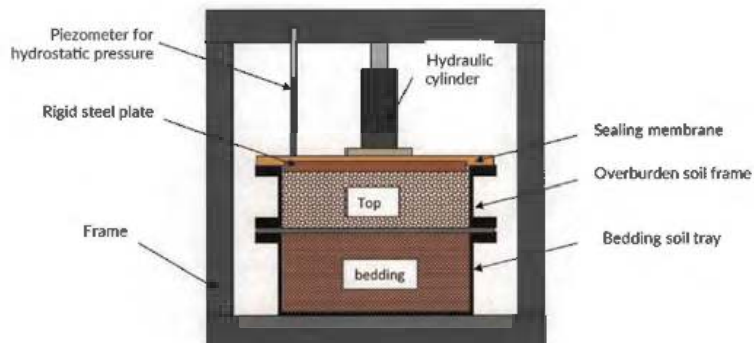
Figure 3. Schematic of puncture testing device.
