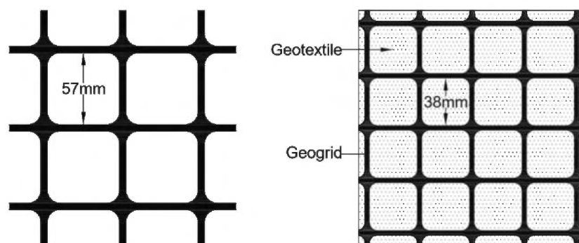
Figure 2. Biaxial geogrid (left) and geocomposite (right).
