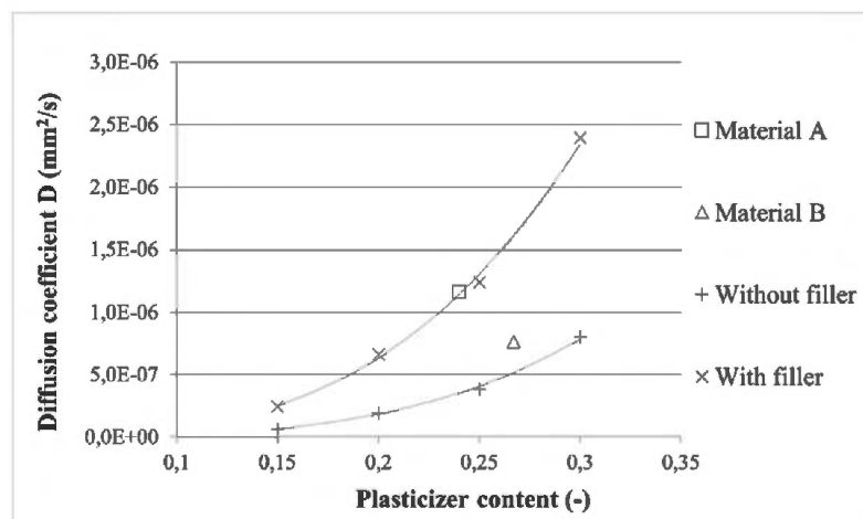
Figure 2. Results of plasticizer absorption tests at 75°C.
