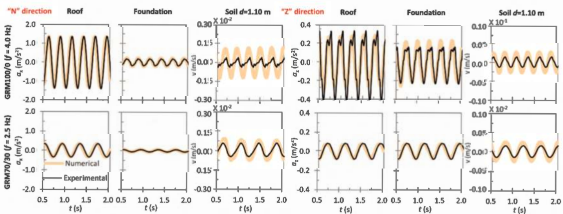
Figure 3. Experimental versus numerical results at the roof and at the foundation in terms of acceleration time histories and on the soil (at 1.10 m from the foundation) in terms of velocity time histories.
