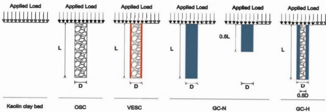
Figure 3. Schematics of different types of columns testing.
