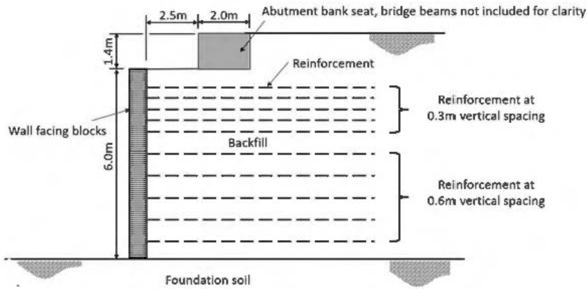
Figure 1. Schematic of GRS-IBS investigated in this study.
