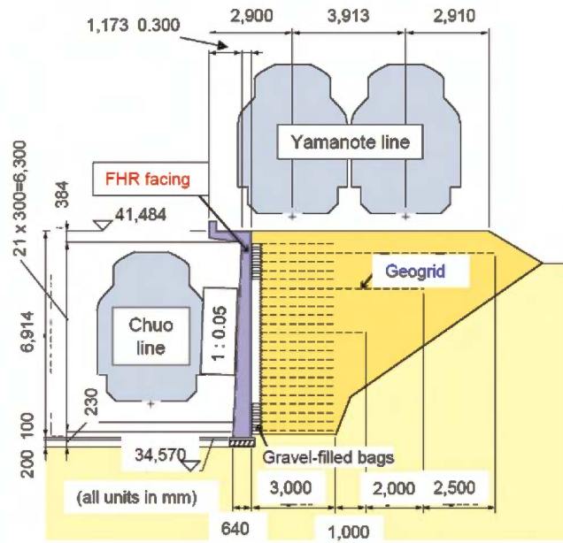
Figure 1. Typical FHR-GRS wall section (Tatsuoka 2008).
