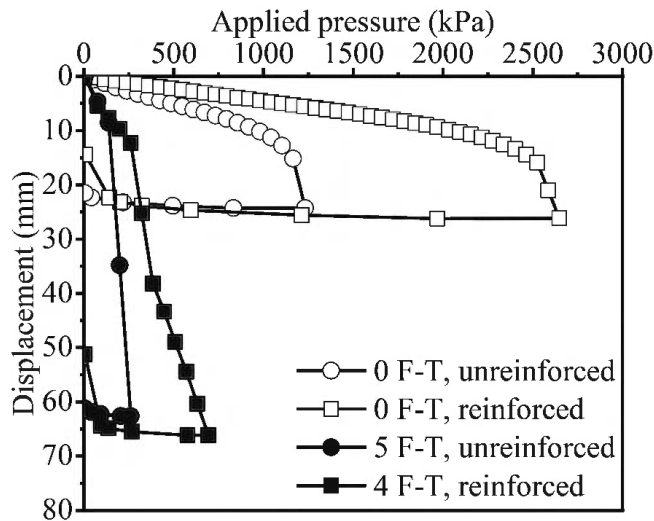
Figure 4. Load-movement curves for unreinforced and reinforced bases.
