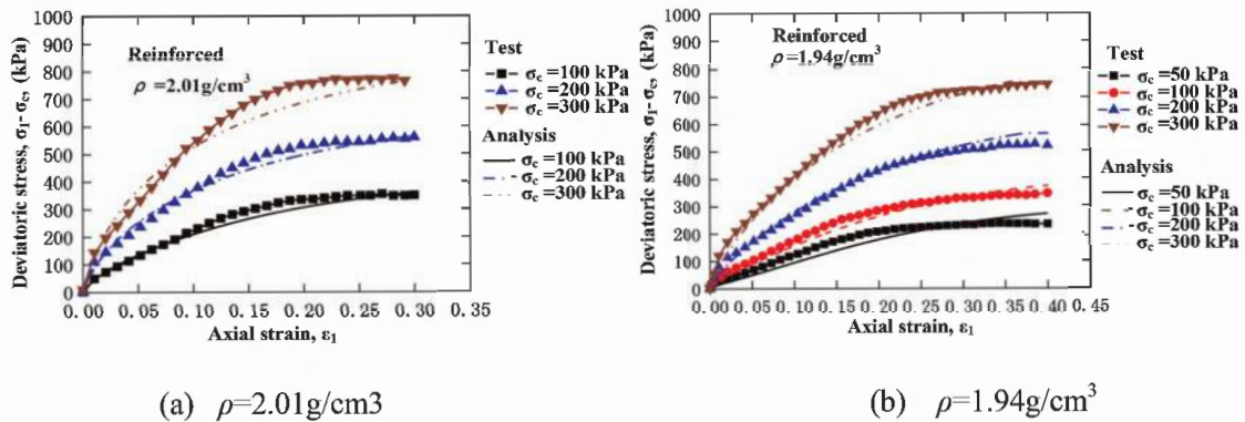
Figure 7. Validation of the proposed method via triaxial compression test results.
