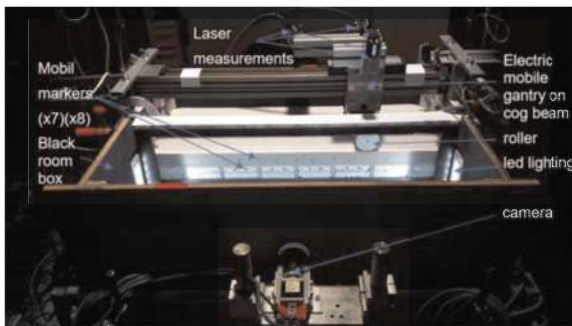
Figure 2. The roller in the transparent-faced strongbox.
