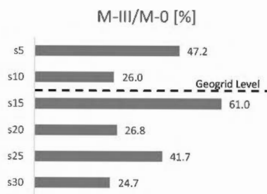
Figure 8. Lateral pressures in M-III vs M-0 (%).
