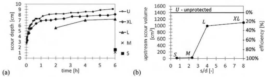
Figure 5. Measured scour: (a) temporal trends of the spatially-maximum scour depth; (b) 6-hours scour volume measured between the upstream edge of the scour hole and the cross section at the pier axis, for increasing s/d mesh size ratios.
