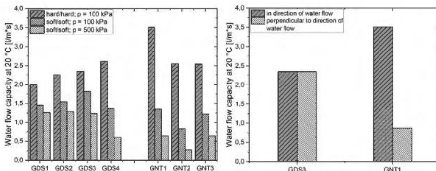
Figure 4. a) Comparison of the water flow capacity of GDS and GNT at different test conditions regarding the bedding situation and the compressive stress ( i = 1.0 ) b) Comparison of the water flow capacity of GDS and GNT as a function of the installation direction ( p = 100 kPa, i = 1.0 , hard/hard).
