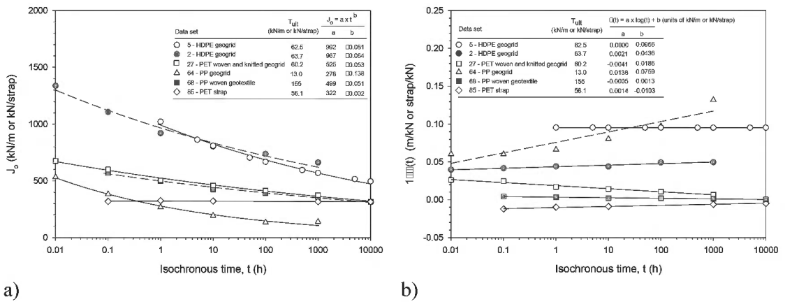
Figure 3. Example plots of hyperbolic model parameters versus isochronous time t : a) J_0 , and; b) 1/\chi(t) (data from Bathurst & Naftchali 2021).
