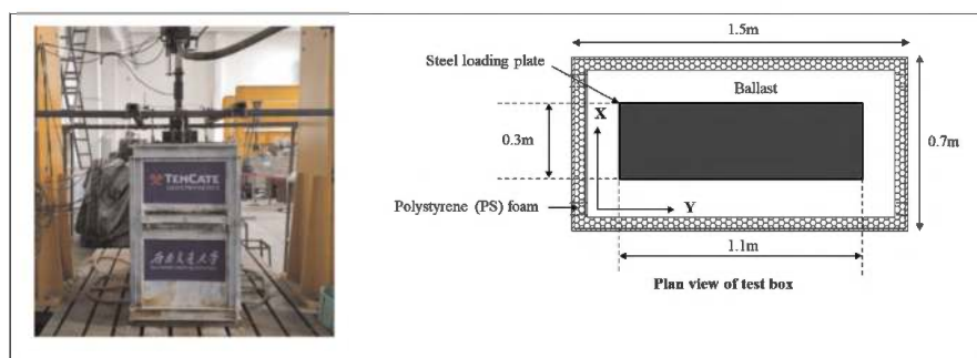
Figure 2. Cyclic train loading test box.
