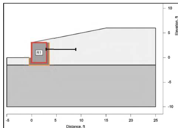
Figure 5. 1-Unit anchored SCOURLOK configuration.
