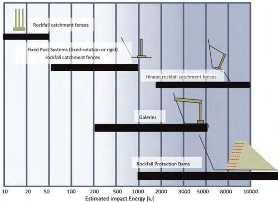
Figure 5. Schematic overview on rockfall protection structures.
