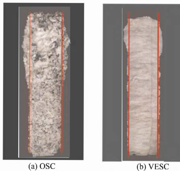
Figure 2. Deformation of columns after test.
