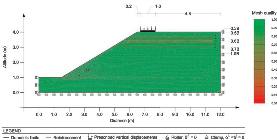
Figure 2. Model boundary conditions and mesh quality ratio.
