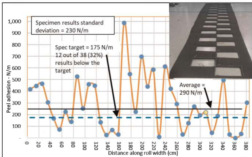
Figure 5. Results of contiguous peel tests across geocomposite panel width (from Thiel & Gatrell 2019).
