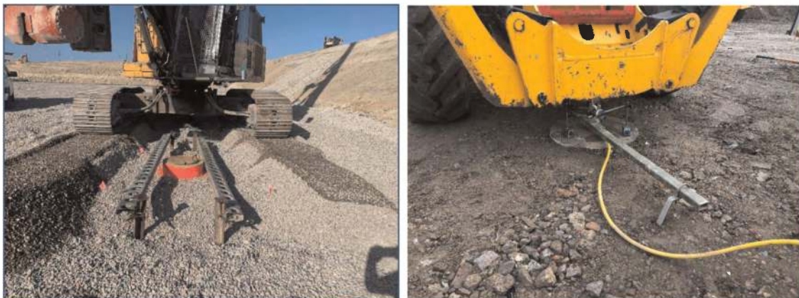
Figure 5. Left: Sand Diego USA 2022 PLT test; Right: Great Yarmouth, UK 2022 PLT.
