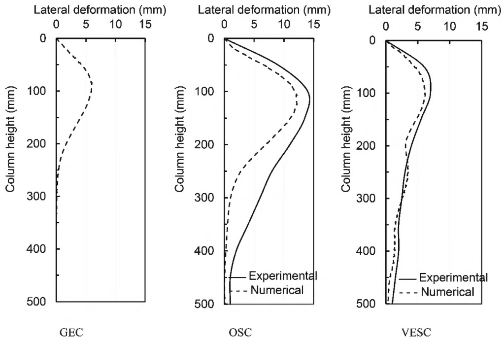
Figure 3. Lateral deformation of the columns ( D = 100 mm).
