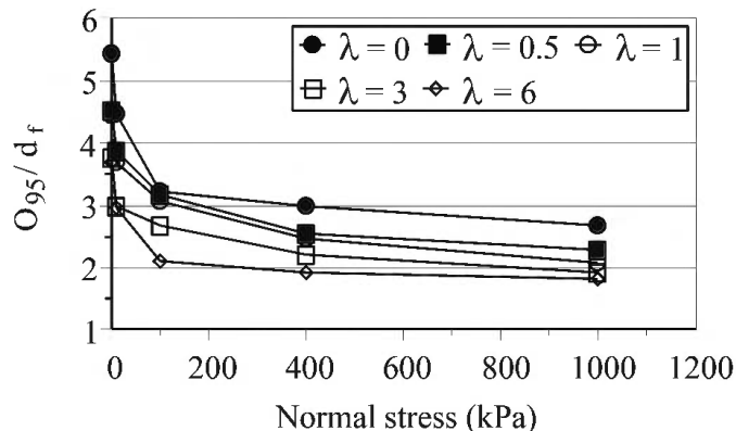
Figure 8. Geotextile filtration opening size vs. confining stress for different impregnation levels (Palmeira & Trejos-Galvis, 2017).
