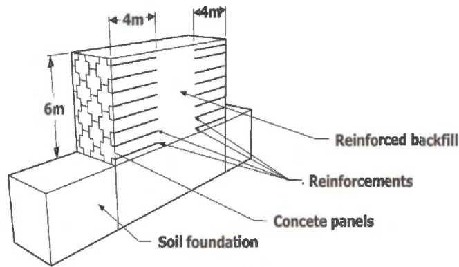
Figure 1. Schematic view of a back-to-back reinforced wall.
