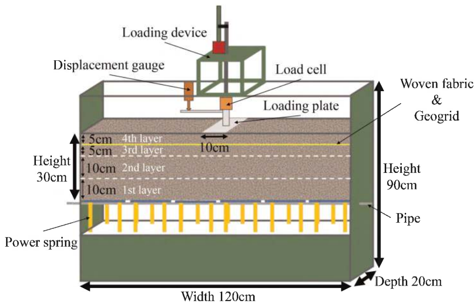
Figure 2. Schematic diagram of the experimental apparatus.
