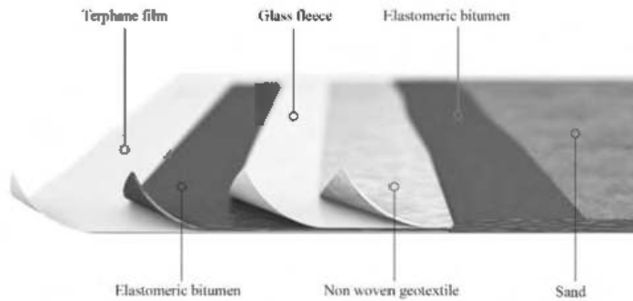
Figure 1. Cross section of bituminous geomembrane.
