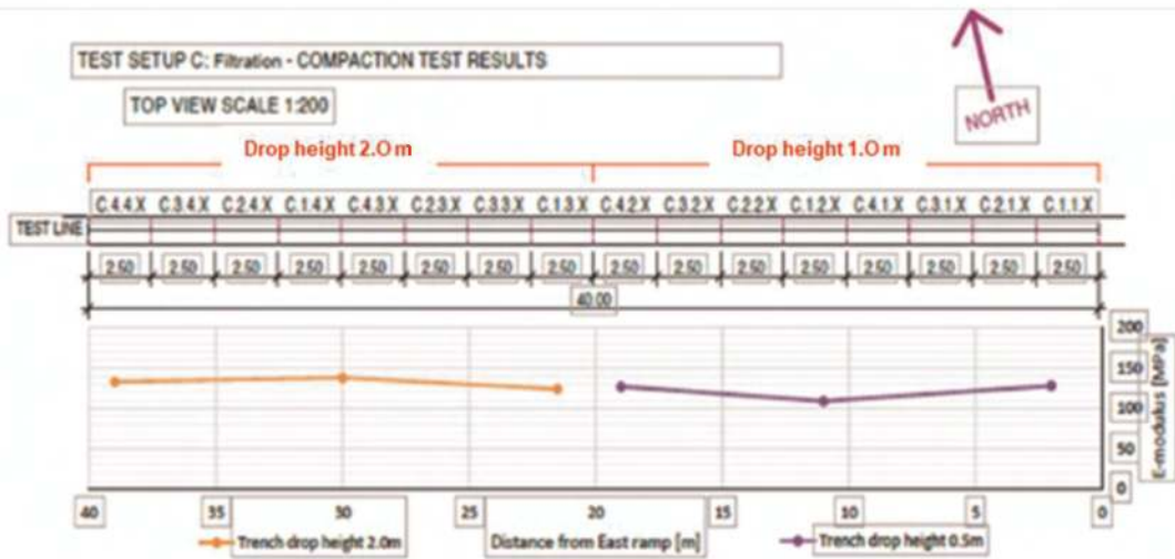
Figure 8. Compaction controls values and arrangement of samples.
