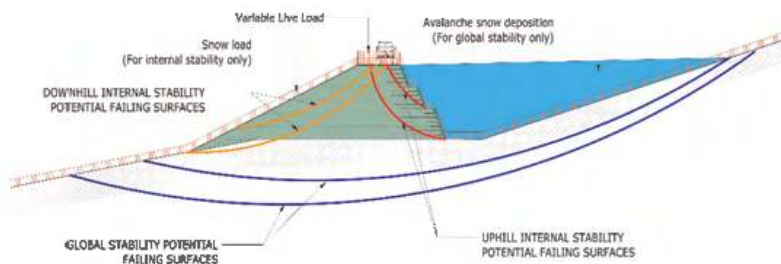
Figure 6. Internal (red) and global (blue) potential failing surfaces.
