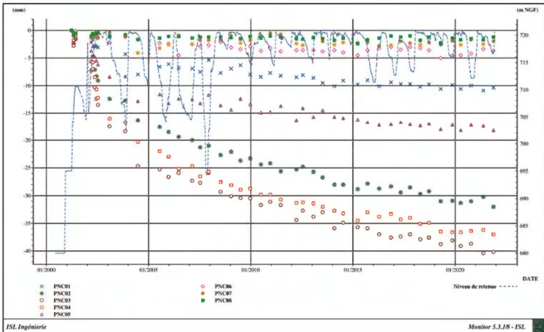
Figure 9. Time evolution of crest elevation measurements.
