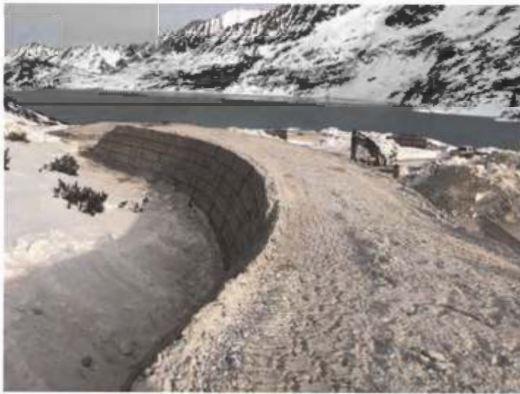
Figure 2. Tauernmoos avalanche deflecting dam during construction. (Nov. 2021).
