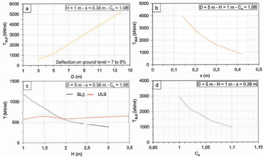
Figure 11. Geosynthetics design – parametric study.
