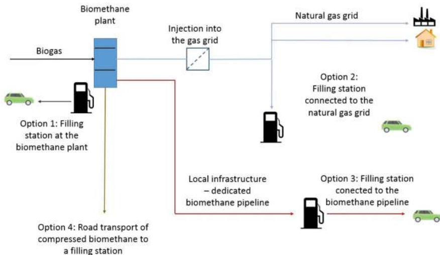
Figure 1. Technical options of filling biomethane for vehicles.
