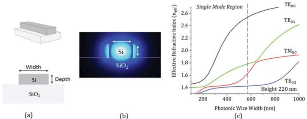
Figure 11. (a) Silicon-on-insulator wire waveguide, (b) quasi-TE mode of a 220-nm-high and 450-nm-wide silicon waveguide at wavelength of 1.55 μm, and (c) effective refractive index ( n_{eff} ) at 1550 nm for a 220-nm-high silicon photonic wire waveguide. The left of the hashed line is the single-mode region.
