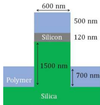
Figure 18. Schematic of an augmented waveguide.
