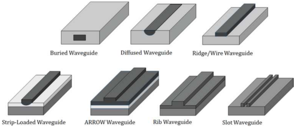
Figure 10. Schematic representation of various channel waveguides.
