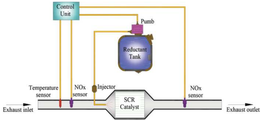
Figure 6. NH 3 -SCR system.
