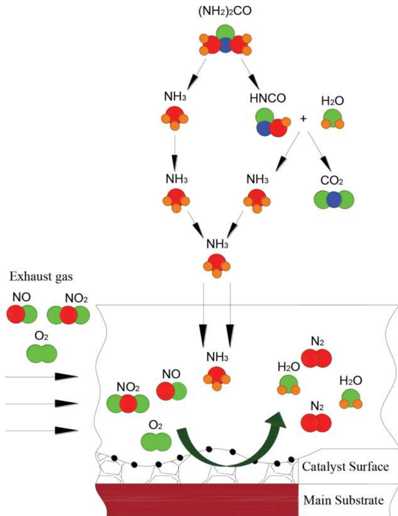
Figure 5. NO x conversion reactions in NH 3 -SCR.
