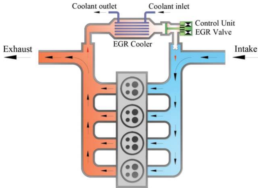
Figure 4. Exhaust gas recirculation (EGR).
