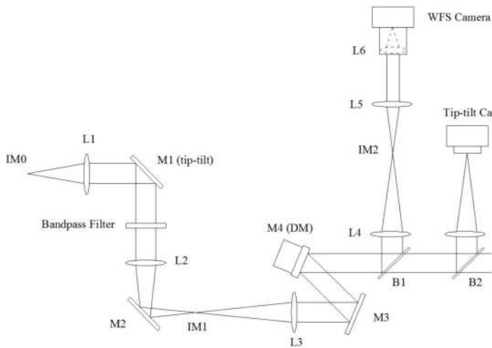
Figure 1. The optical layout of the PSAO.
