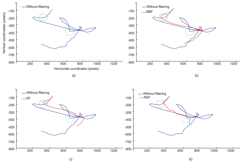
Fig. 15. Pointer path a) without filtering b) with BBF c) with KF d) with RKF
