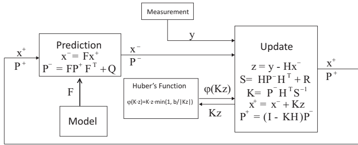
Fig. 14. Block diagram of the robust Kalman filter
