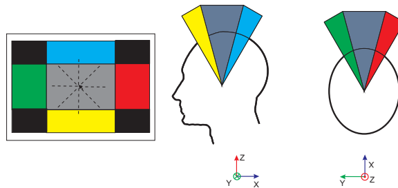
Fig. 9. Control space of joystick mode
