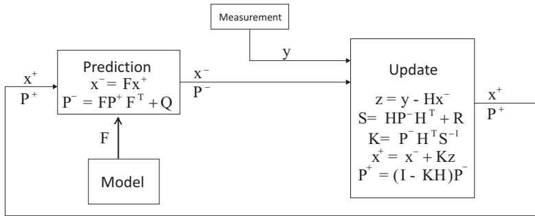
Fig. 12. Block diagram of the Kalman filter
