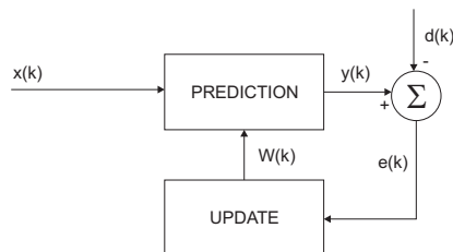
Fig. 10. Block diagram of adaptive filtering implementation
