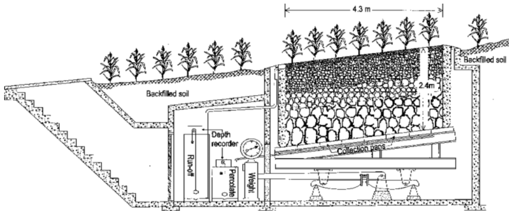
Figure 9. Schematic profile of an underground weighing lysimeter with an undisturbed profile of weathered bedrock near the bottom and soil at the top.
