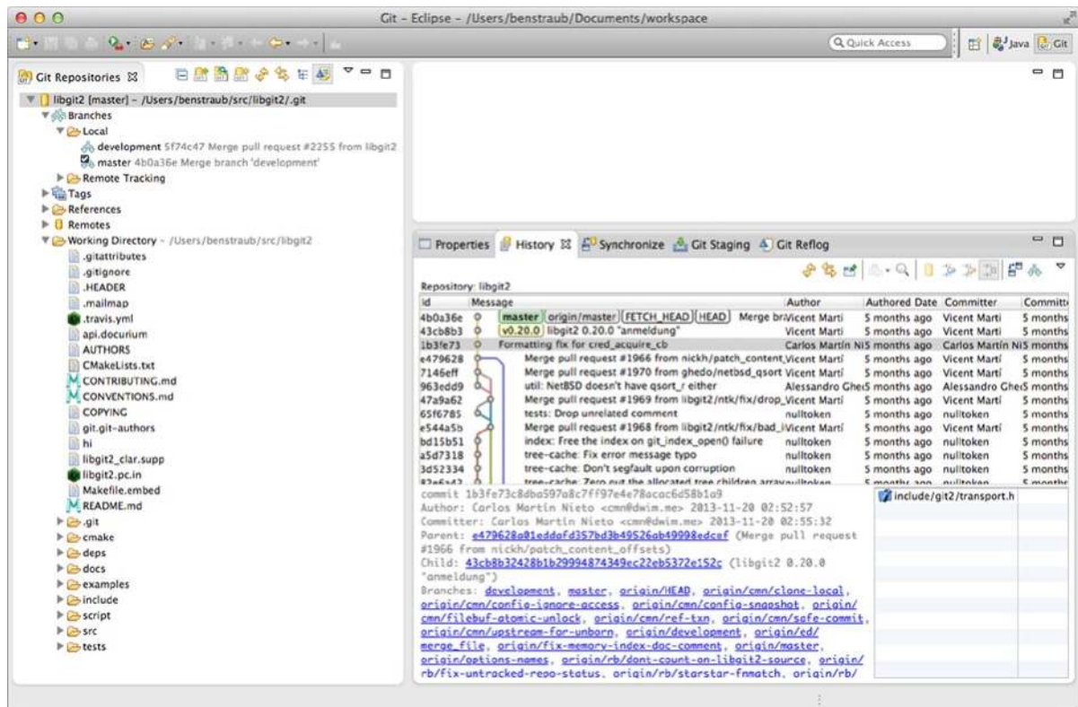
Figure A-9. Eclipse's EGit environment
