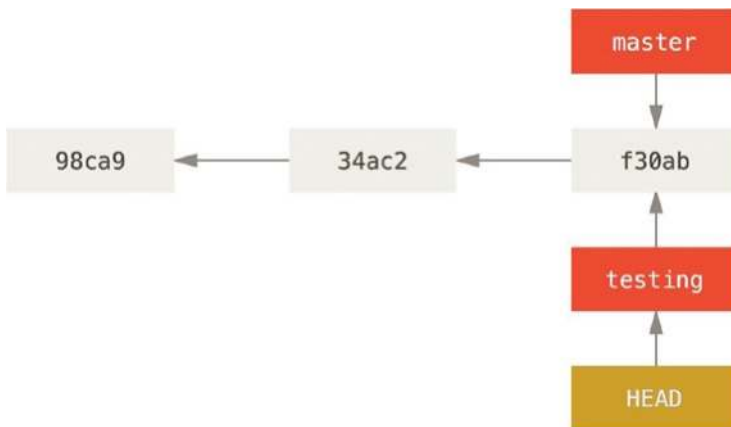
Figure 3-6. HEAD points to the current branch
