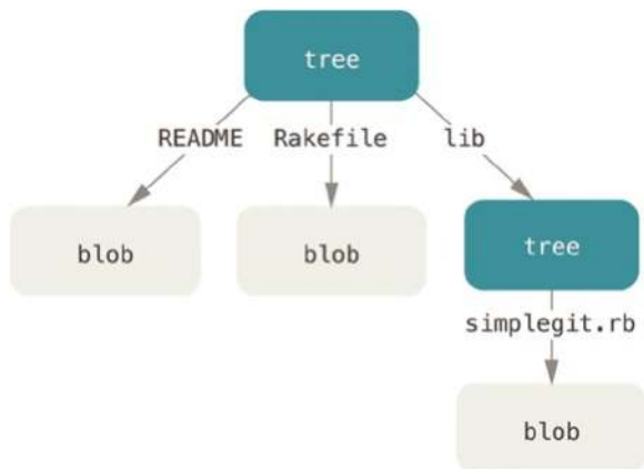
Figure 10-1. Simple version of the Git data model
