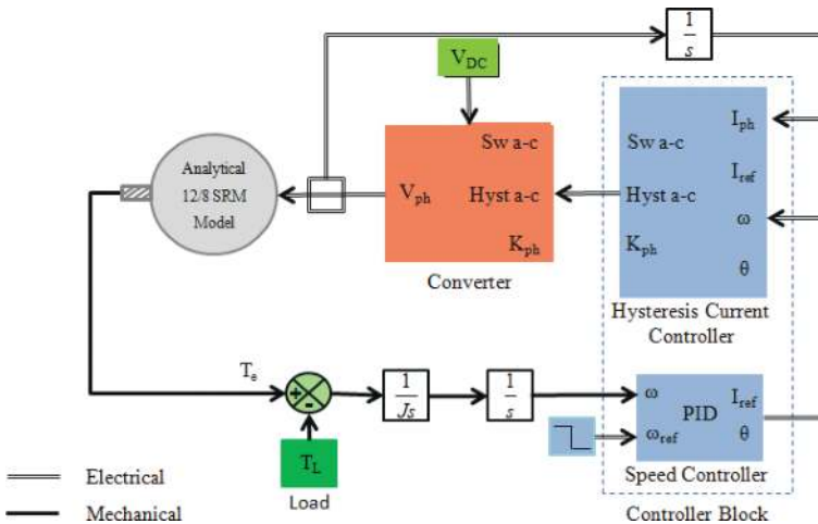
Figure 9. Simulation block diagram of analytical SRM model.
