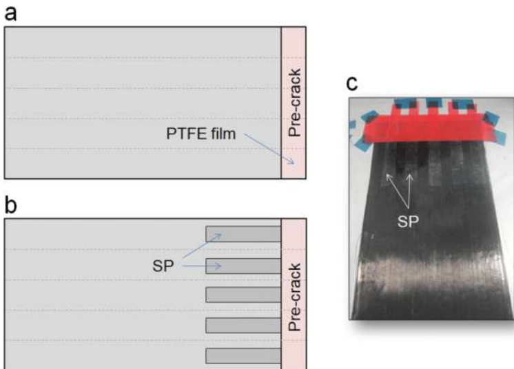
Figure 4. Schematic representation of (a) the reference plate and (b) the modified plate. (c) Photograph of the mid-plane placement of SP film, together with the PTFE initial crack formation.
