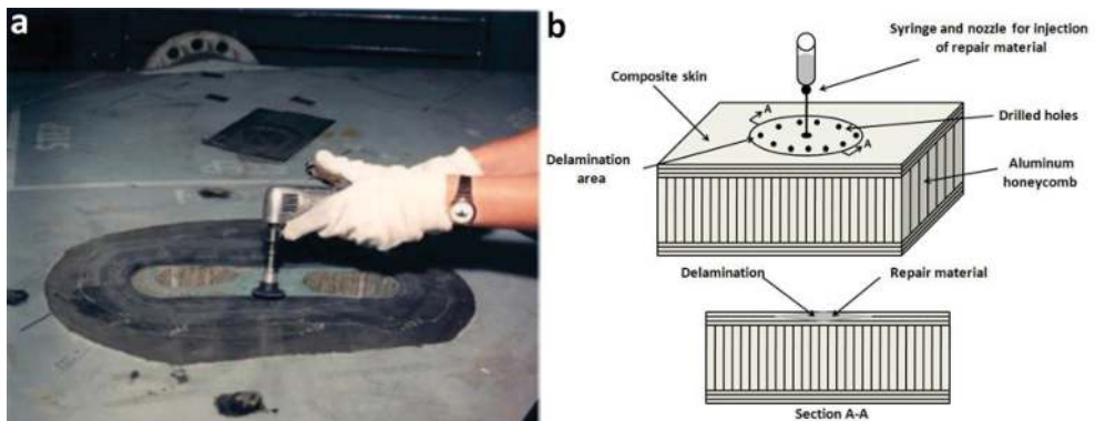
Figure 2. (a) Scarf cavity formation prior to patch repair [15]. (b) Depiction of the resin injection process into honeycomb panel skin's composite.
