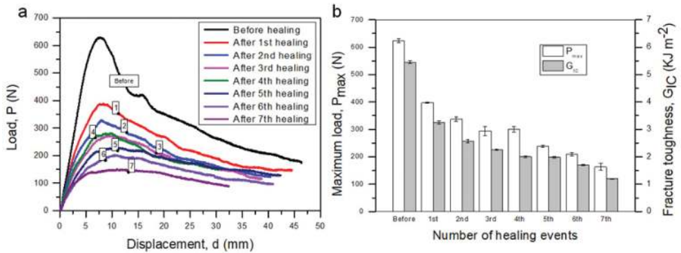
Figure 11. (a) Representative load (P) versus crack opening displacement (d) curves before and after the healing cycles during the mode I experiments. (b) Bar diagrams for the P max and G IC values, before and after the healing cycles in mode I experiments.
