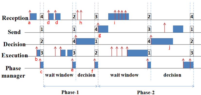
Fig. 8. Temporal diagram of a scheduling sample
