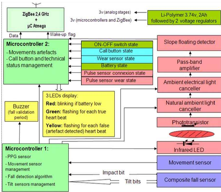
Fig. 3. Internal structure of the wearable device (RFpat)
