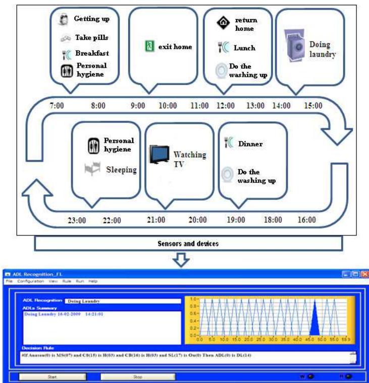
Fig. 9. ADLs recognition experiment for a stream data.
