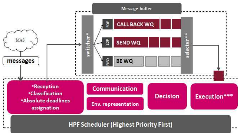
Fig. 7. Real-time scheduling of the central agent.
