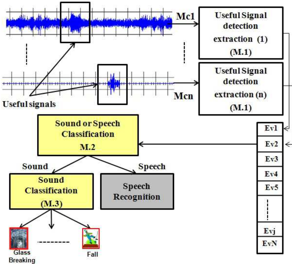
Fig. 2. Anason software architecture
