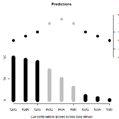
Figure 5.1: Predicted question responses percent (bar plot) and reaction times (points) for the 9 resynthesis conditions: f and d indicate f0 contours and durational patterns, Q , A and S indicate question-like, ambiguous and statement-like patterns. See Cangemi and D’Imperio (2013).
