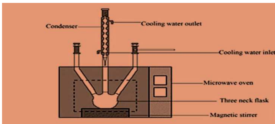
Figure 9. Microwave setup for biodiesel synthesis.
