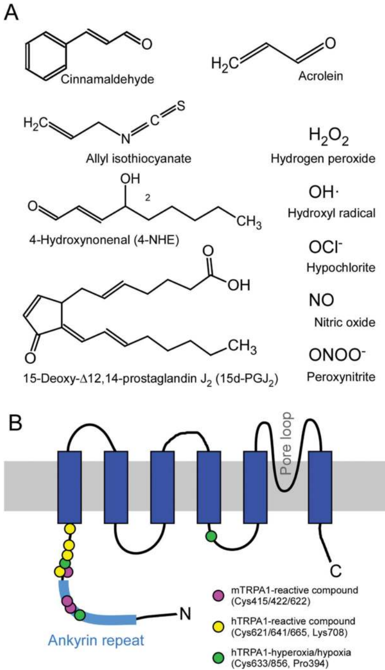
Figure 1. Chemical structure of TRPA1-activating reactive compounds (A) and reported target amino acid residues in TRPA1 (B).
