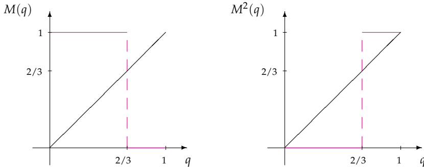
Figure 2. First (left) and second (right) iterations of the maximization map for the mixed-strategy Chicken game. Attached to each plot, a line at 45° which intersects each function at its fixed points. The point q = 2/3 is mapped both under M and M^2 into the whole interval [0, 1] (dashed lines).
