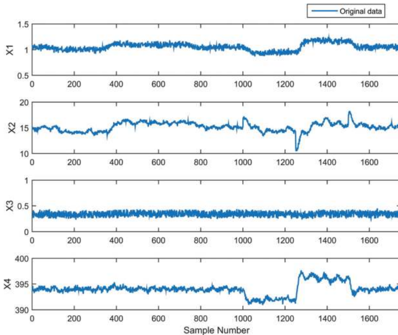
Figure 11. Generated continuously stirred tank reactor (CSTR) data.
