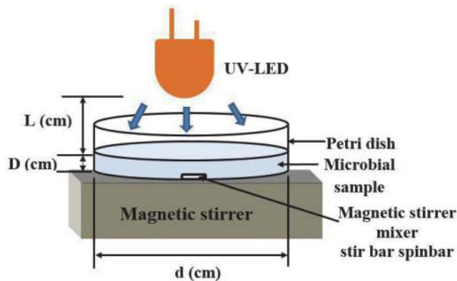
Figure 2. Set-up of a batch disinfection reactor.
